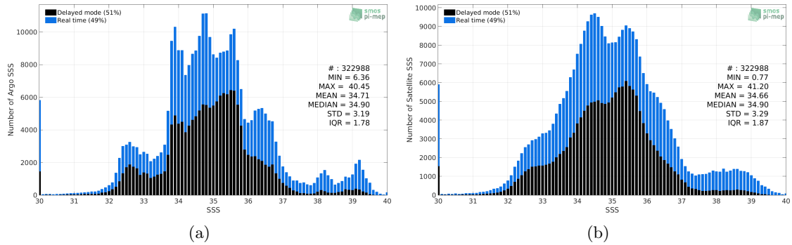
Figure 2: Histograms of SSS from Argo (a) and SMAP-L3-RSS-V4-8DAY-RUNNING (b) considering all match-up pairs per bins of 0.1 over the SMOS coastal zone (<800km) 60N-60S Pi-MEP region and for the full satellite product period.
