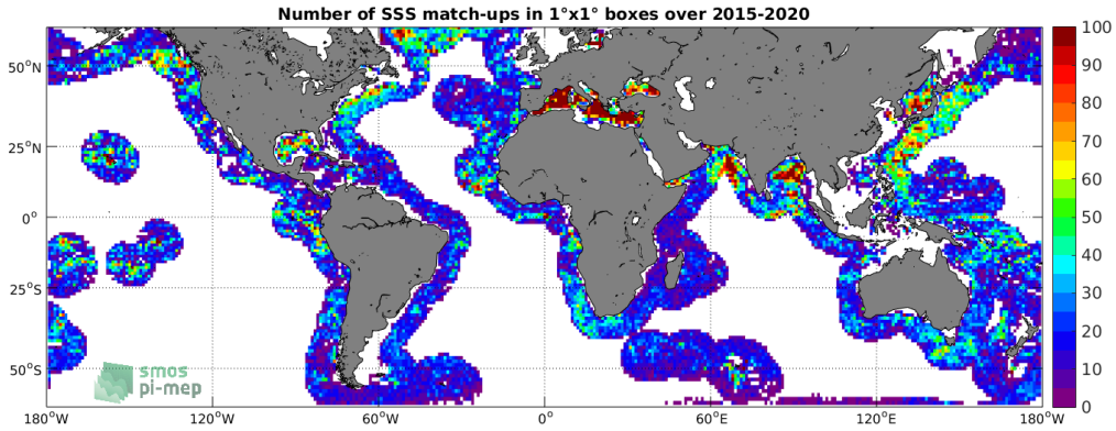
Figure 4: Number of SSS match-ups between Argos SSS and the SMAP-L3-RSS-V4-8DAY-RUNNING SSS product for the SMOS coastal zone (<800km) 60N-60S Pi-MEP region over 1°x1° boxes and for the full satellite product period.
