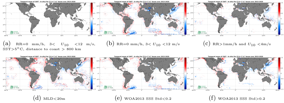
Figure 12: Temporal mean gridded over spatial boxes of size 1^\circ \times 1^\circ of \Delta SSS (SMAP-L3-RSS-V4-8DAY-RUNNING - Argo) for 6 different subdatasets corresponding to: RR=0 mm/h, 3 < U_{10} < 12 m/s, SST > 5^\circ C , distance to coast > 800 km (a), RR=0 mm/h, 3 < U_{10} < 12 m/s (b), RR > 1 mm/h and U_{10} < 4 m/s (c), MLD < 20 m (d), WOA2013 SSS Std < 0.2 (e), WOA2013 SSS Std > 0.2 (f).
