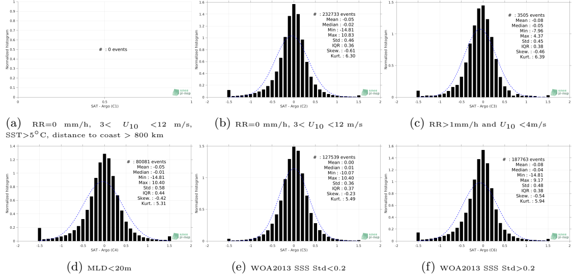
Figure 13: Normalized histogram of \Delta SSS (SMAP-L3-RSS-V4-8DAY-RUNNING - Argo) for 6 different subdatasets corresponding to: RR=0 mm/h, 3 < U_{10} < 12 m/s, SST>5°C, distance to coast > 800 km (a), RR=0 mm/h, 3 < U_{10} < 12 m/s (b), RR>1mm/h and U_{10} < 4 m/s (c), MLD<20m (d), WOA2013 SSS Std<0.2 (e), WOA2013 SSS Std>0.2 (f).
