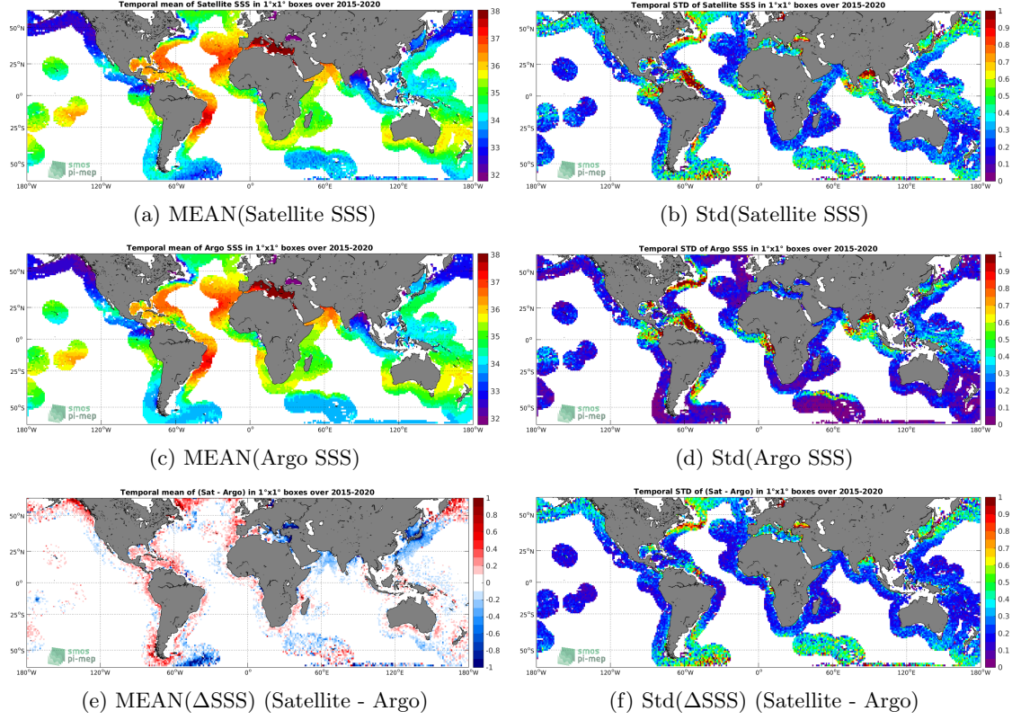
Figure 6: Temporal mean (left) and Std (right) of SSS from SMAP-L3-RSS-V4-8DAY-RUNNING (top), Argo (middle), and of \Delta SSS (Satellite - Argo). Only match-up pairs are used to generate these maps.
