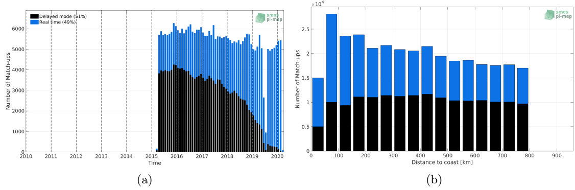
Figure 1: Number of match-ups between Argo and SMAP-L3-RSS-V4-8DAY-RUNNING SSS as a function of time (a) and as function of the distance to coast (b) over the SMOS coastal zone (<800km) 60N-60S Pi-MEP region and for the full satellite product period.
