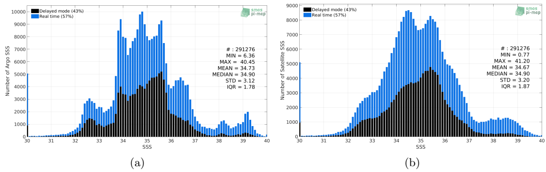
Figure 2: Histograms of SSS from Argo (a) and SMAP-L3-RSS-V4-8DAY-RUNNING (b) considering all match-up pairs per bins of 0.1 over the SMOS coastal zone ( \pm 800 km) 60N-60S Pi-MEP region and for the full satellite product period.
