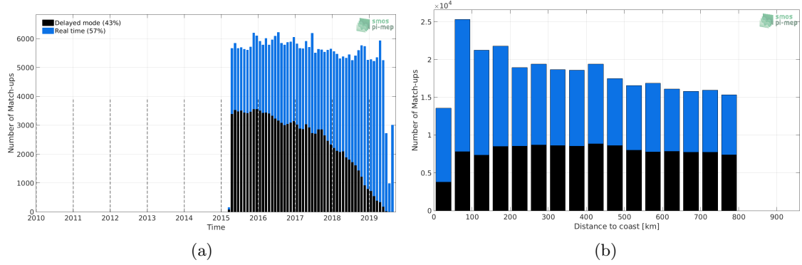
Figure 1: Number of match-ups between Argo and SMAP-L3-RSS-V4-8DAY-RUNNING SSS as a function of time (a) and as function of the distance to coast (b) over the SMOS coastal zone ( \pm 800 km) 60N-60S Pi-MEP region and for the full satellite product period.
