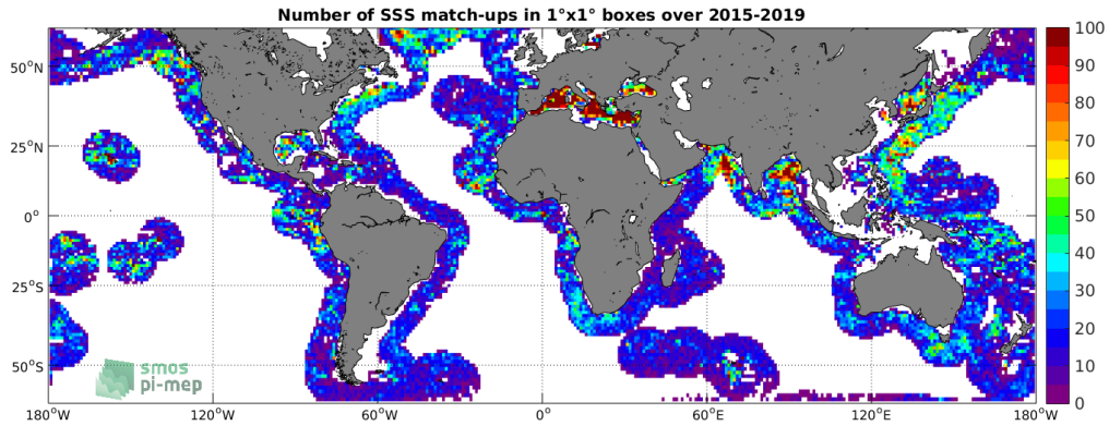
Figure 4: Number of SSS match-ups between Argo SSS and the SMAP-L3-RSS-V4-8DAY-RUNNING SSS product for the SMOS coastal zone ( \pm 800\text{km} ) 60N-60S Pi-MEP region over 1^\circ \times 1^\circ boxes and for the full satellite product period.
