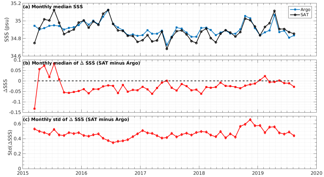
Figure 7: Time series of the monthly median SSS (top), median of \Delta SSS (Satellite - Argo) and Std of \Delta SSS (Satellite - Argo) over the SMOS coastal zone ( \geq 800 km) 60N-60S Pi-MEP region considering all match-ups collected by the Pi-MEP.
