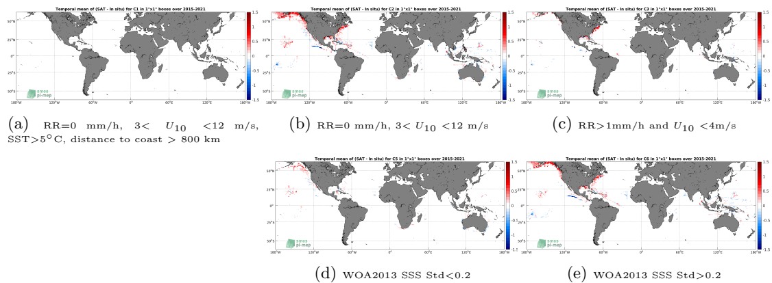
Figure 12: Temporal mean gridded over spatial boxes of size 1^\circ \times 1^\circ of \Delta SSS (SMAP SSS L3 v4 - Monthly (RSS) - TSG (SAMOS)) for 5 different subdatasets corresponding to:RR=0 mm/h, 3 < U_{10} < 12 m/s, SST >5^\circ C, distance to coast > 800 km (a), RR=0 mm/h, 3 < U_{10} < 12 m/s (b), RR >1 mm/h and U_{10} < 4 m/s (c), WOA2013 SSS Std <0.2 (d), WOA2013 SSS Std >0.2 (e).
