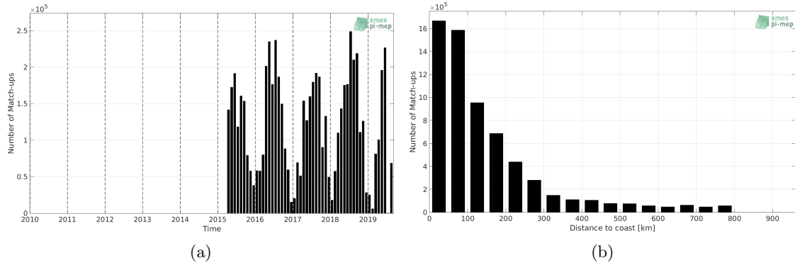
Figure 1: Number of match-ups between TSG-SAMOS and SMAP-L3-RSS-V4-MONTHLY SSS as a function of time (a) and as function of the distance to coast (b) over the SMOS coastal zone ( \pm 800\text{km} ) 60N-60S Pi-MEP region and for the full satellite product period.
