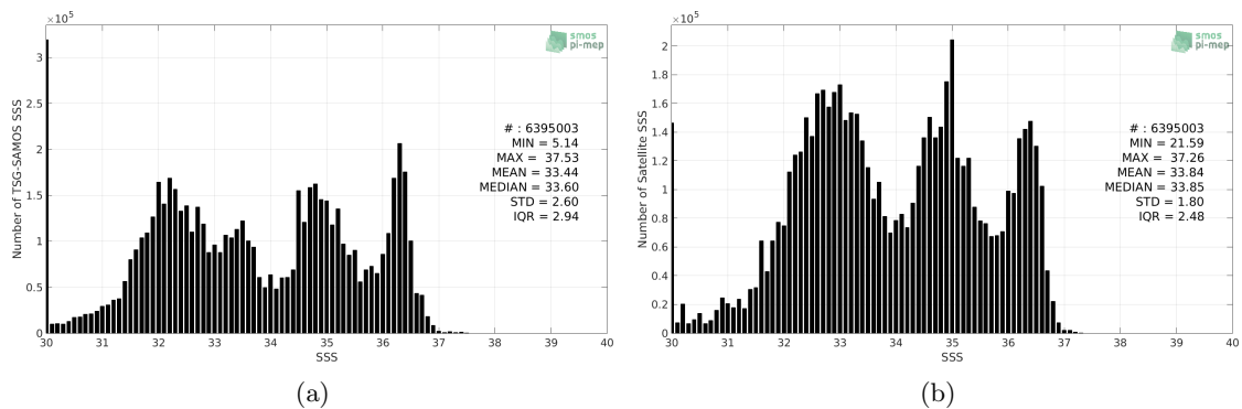
Figure 2: Histograms of SSS from TSG-SAMOS (a) and SMAP-L3-RSS-V4-MONTHLY (b) considering all match-up pairs per bins of 0.1 over the SMOS coastal zone ( \pm 800\text{km} ) 60N-60S Pi-MEP region and for the full satellite product period.
