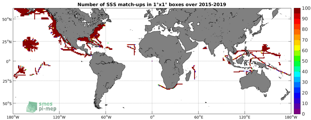
Figure 4: Number of SSS match-ups between TSG-SAMOS SSS and the SMAP-L3-RSS-V4-MONTHLY SSS product for the SMOS coastal zone ( \approx 800 km) 60N-60S Pi-MEP region over 1^\circ \times 1^\circ boxes and for the full satellite product period.
