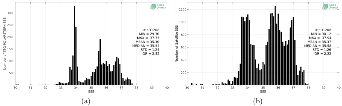
Figure 2: Histograms of SSS from TSG-POLARSTERN (a) and SMAP-L3-RSS-V4-MONTHLY (b) considering all match-up pairs per bins of 0.1 over the SMOS coastal zone (<800km) 60N-60S Pi-MEP region and for the full satellite product period.
