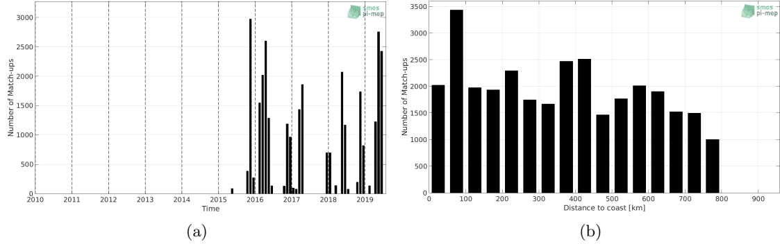
Figure 1: Number of match-ups between TSG-POLARSTERN and SMAP-L3-RSS-V4-MONTHLY SSS as a function of time (a) and as function of the distance to coast (b) over the SMOS coastal zone (<800km) 60N-60S Pi-MEP region and for the full satellite product period.
