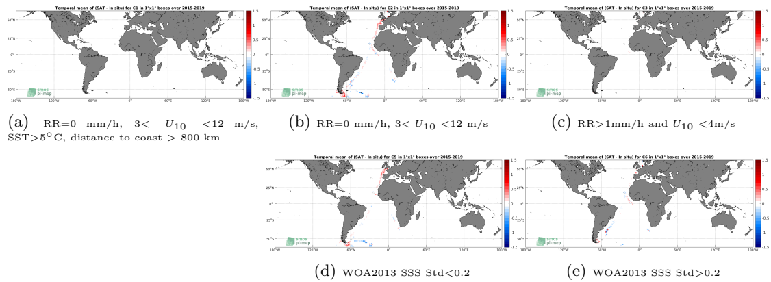
Figure 12: Temporal mean gridded over spatial boxes of size 1^\circ \times 1^\circ of \Delta SSS (SMAP-L3-RSS-V4-MONTHLY - TSG-POLARSTERN) for 5 different subdatasets corresponding to:RR=0 mm/h, 3 < U_{10} < 12 m/s, SST >5^\circ\text{C} , distance to coast > 800 km (a), RR=0 mm/h, 3 < U_{10} < 12 m/s (b), RR >1 mm/h and U_{10} < 4 m/s (c), WOA2013 SSS Std <0.2 (d), WOA2013 SSS Std >0.2 (e).
