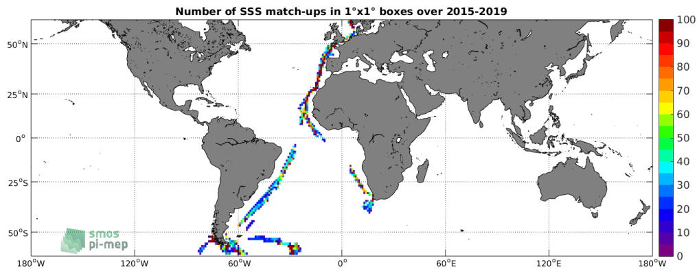
Figure 4: Number of SSS match-ups between TSG-POLARSTERN SSS and the SMAP-L3-RSS-V4-MONTHLY SSS product for the SMOS coastal zone (<800km) 60N-60S Pi-MEP region over 1°x1° boxes and for the full satellite product period.
