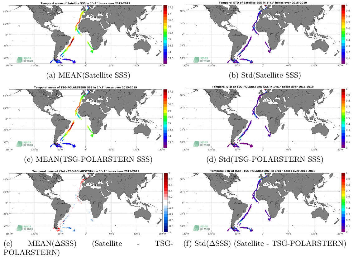
Figure 6: Temporal mean (left) and Std (right) of SSS from SMAP-L3-RSS-V4-MONTHLY (top), TSG-POLARSTERN (middle), and of \Delta SSS (Satellite - TSG-POLARSTERN). Only match-up pairs are used to generate these maps.
