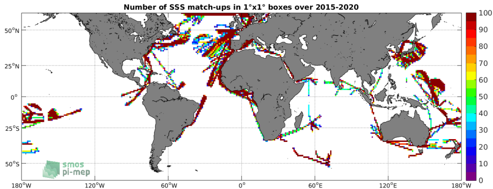
Figure 4: Number of SSS match-ups between TSG (LEGOS-DM) SSS and the SMAP SSS L3 v4 - Monthly (RSS) SSS product for the SMOS coastal zone (<800km) 60N-60S Pi-MEP region over 1°×1° boxes and for the full satellite product period.
