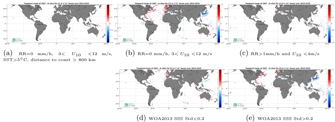
Figure 12: Temporal mean gridded over spatial boxes of size 1^\circ \times 1^\circ of \Delta SSS (SMAP-L3-RSS-V4-MONTHLY - TSG-LEGOS-DM) for 5 different subdatasets corresponding to:RR=0 mm/h, 3 < U_{10} < 12 m/s, SST >5^\circ\text{C} , distance to coast > 800 km (a), RR=0 mm/h, 3 < U_{10} < 12 m/s (b), RR >1 mm/h and U_{10} < 4 m/s (c), WOA2013 SSS Std <0.2 (d), WOA2013 SSS Std >0.2 (e).
