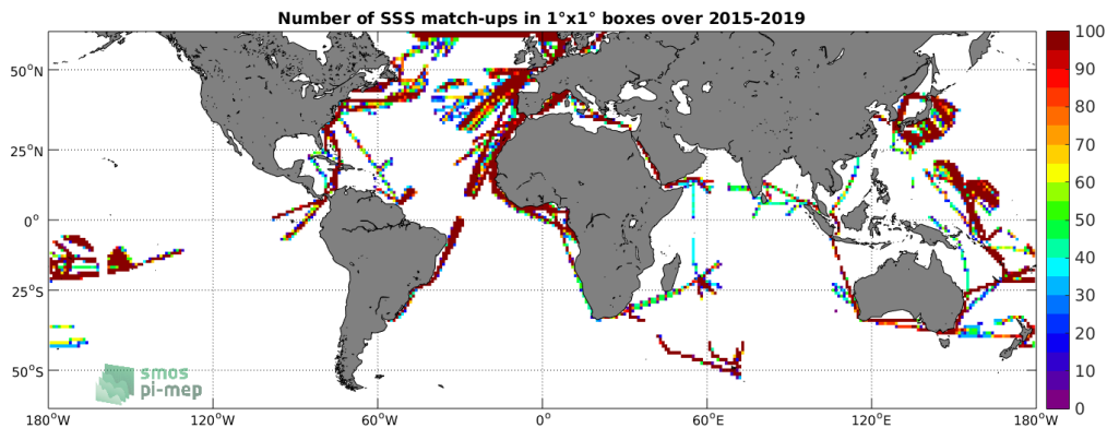
Figure 4: Number of SSS match-ups between TSG-LEGOS-DM SSS and the SMAP-L3-RSS-V4-MONTHLY SSS product for the SMOS coastal zone (<800km) 60N-60S Pi-MEP region over 1^\circ \times 1^\circ boxes and for the full satellite product period.
