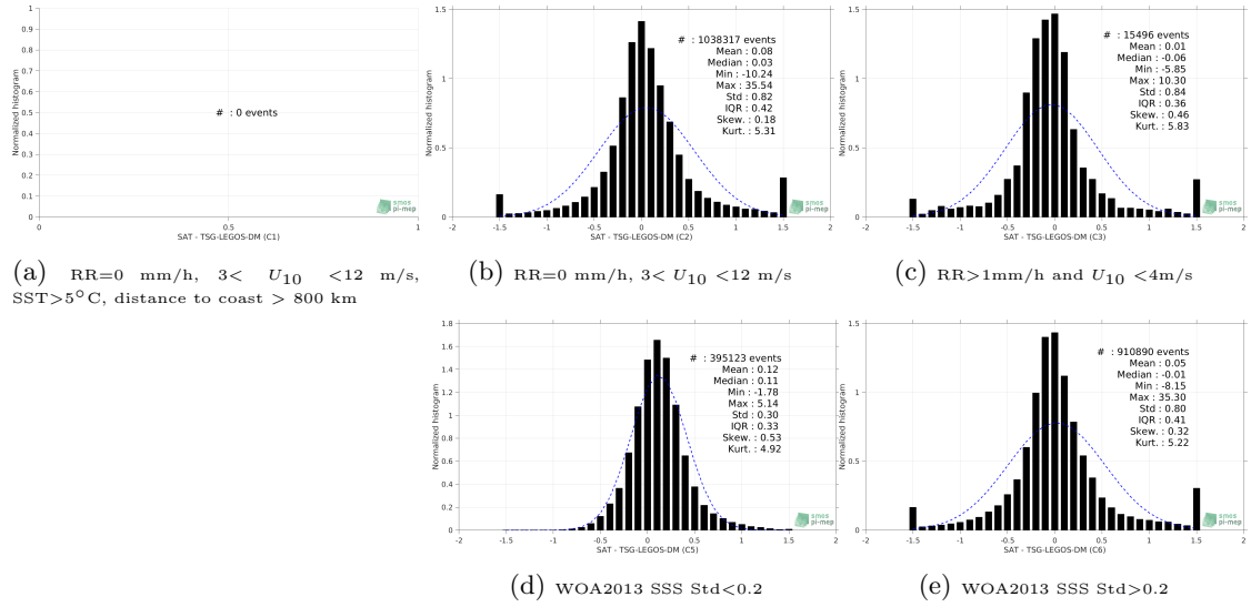
Figure 13: Normalized histogram of \Delta SSS (SMAP-L3-RSS-V4-MONTHLY - TSG-LEGOS-DM) for 5 different subdatasets corresponding to: RR=0 mm/h, 3 < U_{10} < 12 m/s, SST > 5°C, distance to coast > 800 km (a), RR=0 mm/h, 3 < U_{10} < 12 m/s (b), RR > 1mm/h and U_{10} < 4 m/s (c), WOA2013 SSS Std < 0.2 (d), WOA2013 SSS Std > 0.2 (e).
