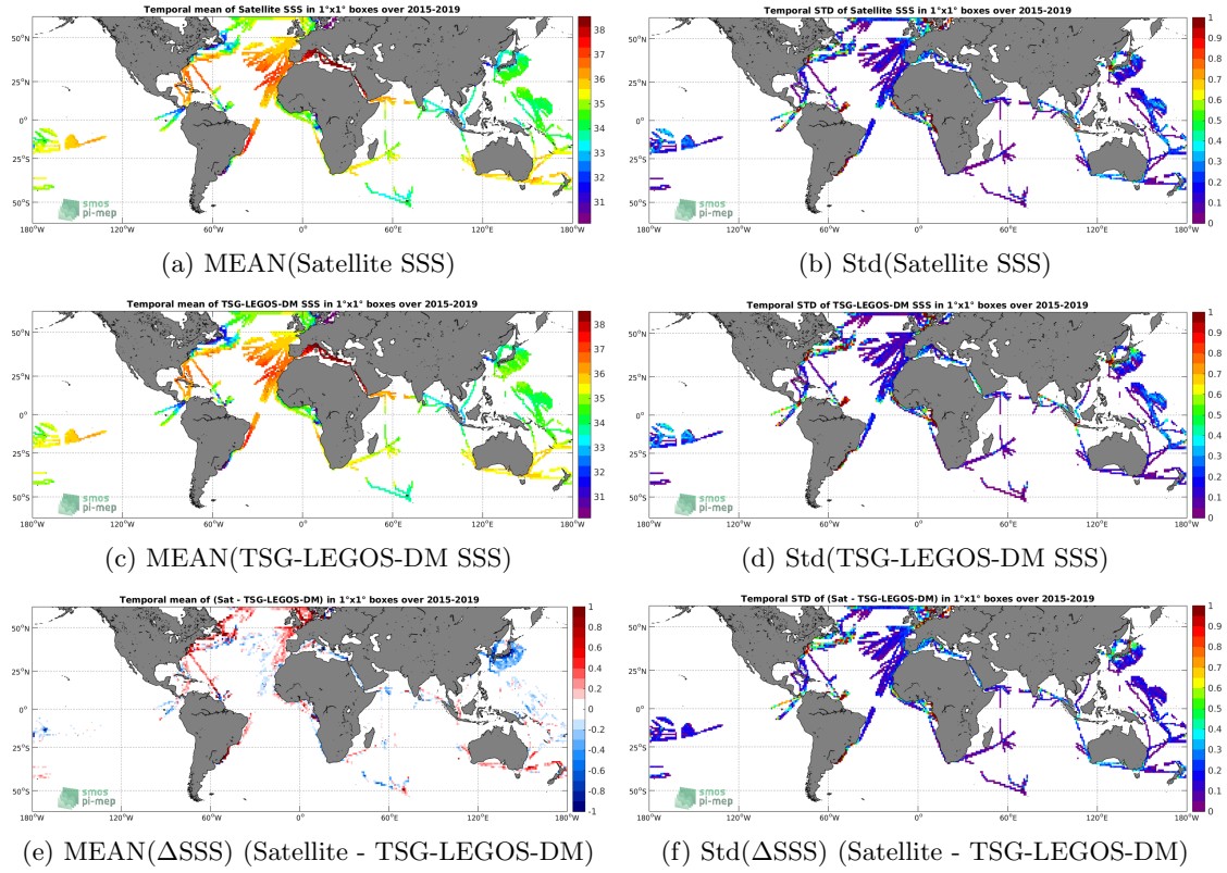
Figure 6: Temporal mean (left) and Std (right) of SSS from SMAP-L3-RSS-V4-MONTHLY (top), TSG-LEGOS-DM (middle), and of \Delta SSS (Satellite - TSG-LEGOS-DM). Only match-up pairs are used to generate these maps.
