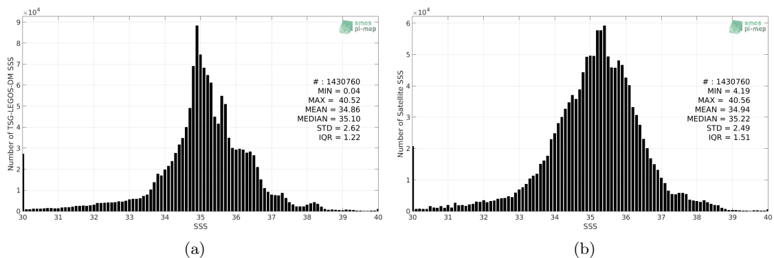
Figure 2: Histograms of SSS from TSG-LEGOS-DM (a) and SMAP-L3-RSS-V4-MONTHLY (b) considering all match-up pairs per bins of 0.1 over the SMOS coastal zone (<800km) 60N-60S Pi-MEP region and for the full satellite product period.
