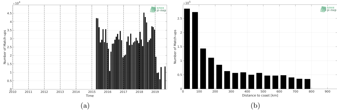
Figure 1: Number of match-ups between TSG-LEGOS-DM and SMAP-L3-RSS-V4-MONTHLY SSS as a function of time (a) and as function of the distance to coast (b) over the SMOS coastal zone (<800km) 60N-60S Pi-MEP region and for the full satellite product period.
