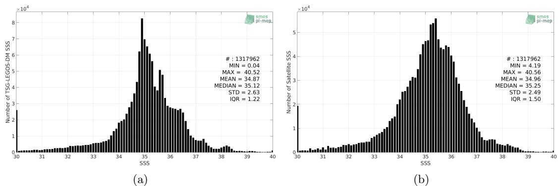
Figure 2: Histograms of SSS from TSG-LEGOS-DM (a) and SMAP-L3-RSS-V4-MONTHLY (b) considering all match-up pairs per bins of 0.1 over the SMOS coastal zone ( \pm 800 km) 60N-60S Pi-MEP region and for the full satellite product period.
