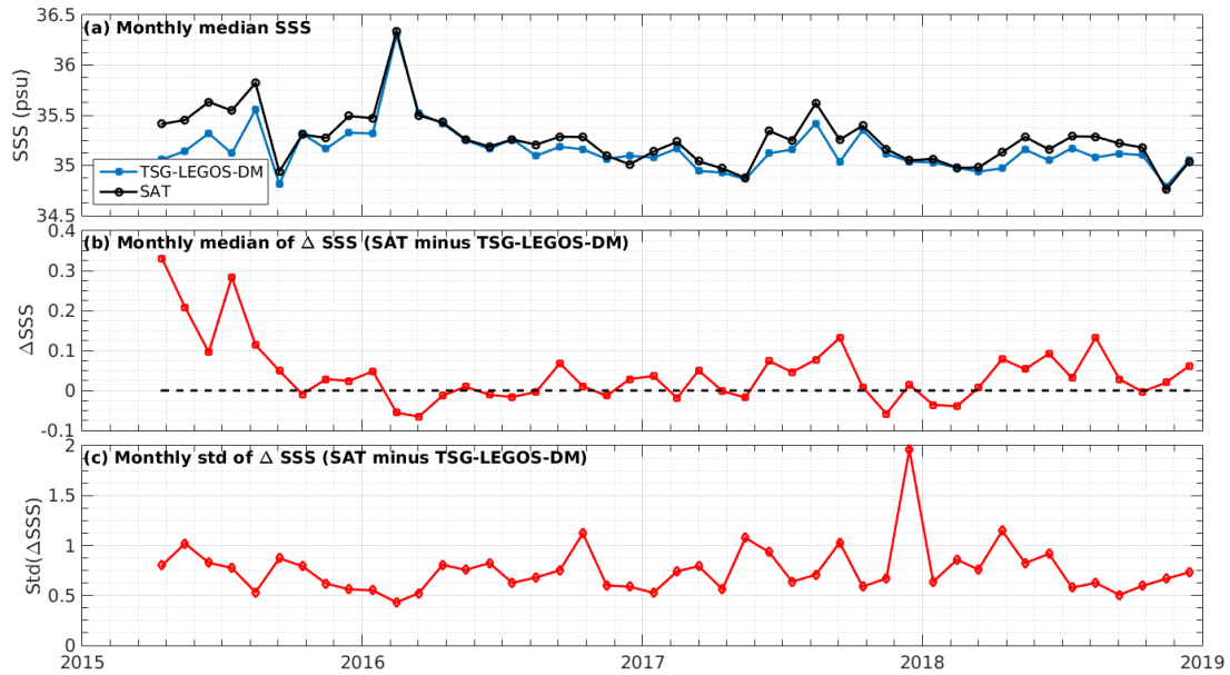
Figure 7: Time series of the monthly median SSS (top), median of \Delta SSS (Satellite - TSG-LEGOS-DM) and Std of \Delta SSS (Satellite - TSG-LEGOS-DM) over the SMOS coastal zone ( \approx 800 km) 60N-60S Pi-MEP region considering all match-ups collected by the Pi-MEP.
