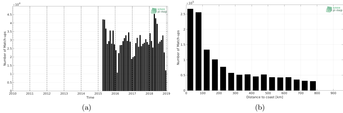
Figure 1: Number of match-ups between TSG-LEGOS-DM and SMAP-L3-RSS-V4-MONTHLY SSS as a function of time (a) and as function of the distance to coast (b) over the SMOS coastal zone ( \pm 800 km) 60N-60S Pi-MEP region and for the full satellite product period.
