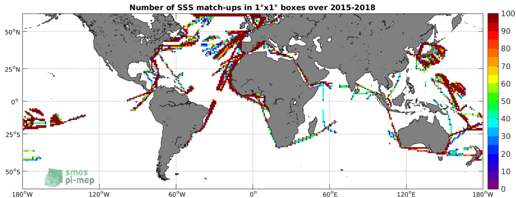
Figure 4: Number of SSS match-ups between TSG-LEGOS-DM SSS and the SMAP-L3-RSS-V4-MONTHLY SSS product for the SMOS coastal zone ( \pm 800\text{km} ) 60N-60S Pi-MEP region over 1^\circ \times 1^\circ boxes and for the full satellite product period.
