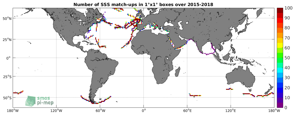
Figure 4: Number of SSS match-ups between TSG (GOSUD-Sailing-ship) SSS and the SMAP SSS L3 v4 - Monthly (RSS) SSS product for the SMOS coastal zone (<800km) 60N-60S Pi-MEP region over 1^\circ \times 1^\circ boxes and for the full satellite product period.
