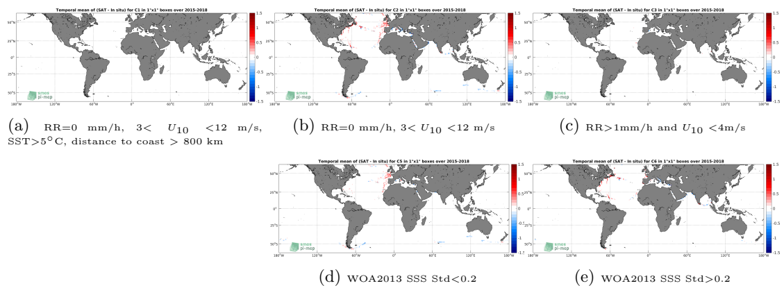
Figure 12: Temporal mean gridded over spatial boxes of size 1^\circ \times 1^\circ of \Delta\text{SSS} (SMAP SSS L3 v4 - Monthly (RSS) - TSG (GOSUD-Sailing-ship)) for 5 different subdatasets corresponding to:RR=0 mm/h, 3 < U_{10} < 12 m/s, SST>5°C, distance to coast > 800 km (a), RR=0 mm/h, 3 < U_{10} < 12 m/s (b), RR>1mm/h and U_{10} < 4 m/s (c), WOA2013 SSS Std<0.2 (d), WOA2013 SSS Std>0.2 (e).
