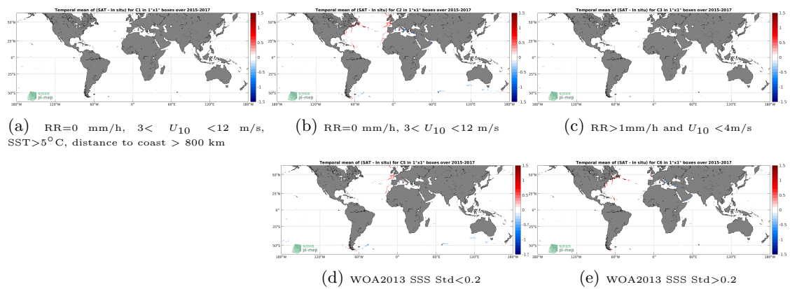
Figure 12: Temporal mean gridded over spatial boxes of size 1°x1° of \Delta SSS (SMAP SSS L3 v4 - Monthly (RSS) - TSG (GOSUD-Sailing-ship)) for 5 different subdatasets corresponding to:RR=0 mm/h, 3 < U_{10} < 12 m/s, SST > 5°C, distance to coast > 800 km (a), RR=0 mm/h, 3 < U_{10} < 12 m/s (b), RR > 1mm/h and U_{10} < 4 m/s (c), WOA2013 SSS Std < 0.2 (d), WOA2013 SSS Std > 0.2 (e).
