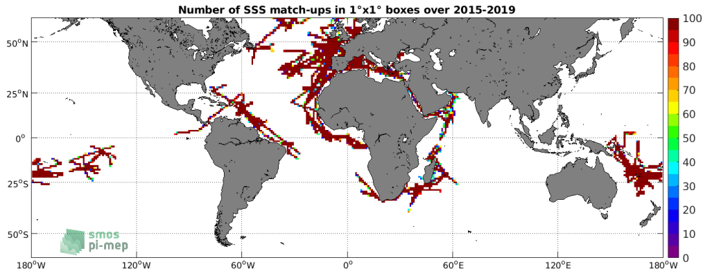
Figure 4: Number of SSS match-ups between TSG (GOSUD-Research-vessel) SSS and the SMAP SSS L3 v4 - Monthly (RSS) SSS product for the SMOS coastal zone (<800km) 60N-60S Pi-MEP region over 1^\circ \times 1^\circ boxes and for the full satellite product period.
