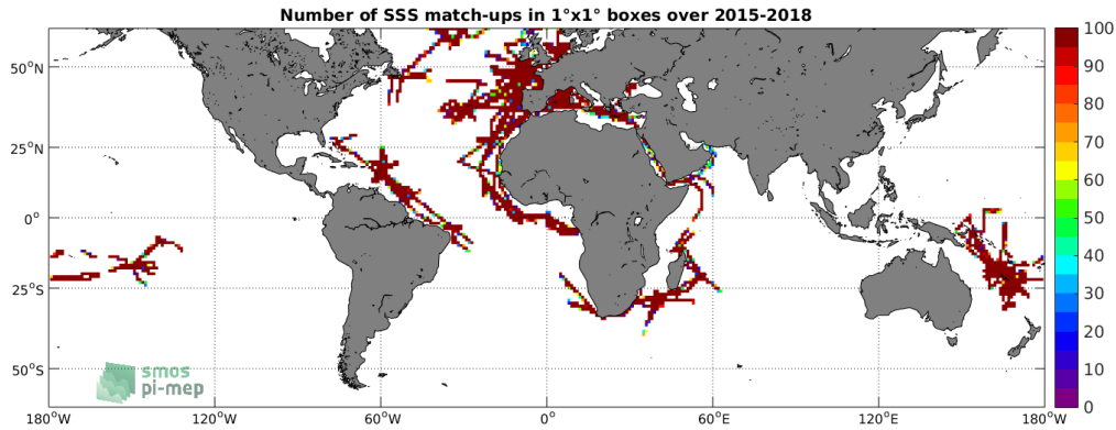
Figure 4: Number of SSS match-ups between TSG-GOSUD-Research-vessel SSS and the SMAP-L3-RSS-V4-MONTHLY SSS product for the SMOS coastal zone (<800km) 60N-60S Pi-MEP region over 1°x1° boxes and for the full satellite product period.
