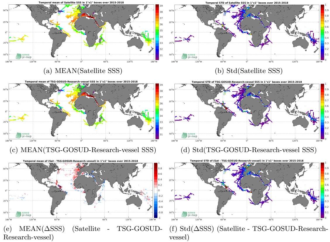
Figure 6: Temporal mean (left) and Std (right) of SSS from SMAP-L3-RSS-V4-MONTHLY (top), TSG-GOSUD-Research-vessel (middle), and of \Delta SSS (Satellite - TSG-GOSUD-Research-vessel). Only match-up pairs are used to generate these maps.
