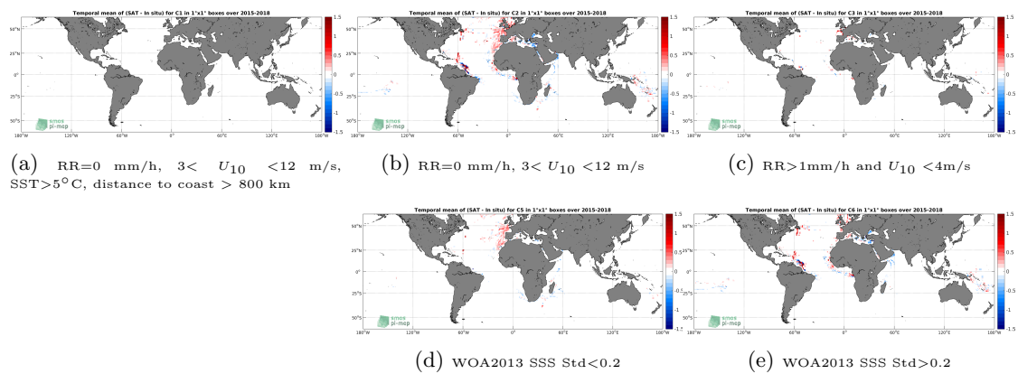
Figure 12: Temporal mean gridded over spatial boxes of size 1^\circ \times 1^\circ of \Delta SSS (SMAP-L3-RSS-V4-MONTHLY - TSG-GOSUD-Research-vessel) for 5 different subdatasets corresponding to:RR=0 mm/h, 3 < U_{10} < 12 m/s, SST >5^\circ C, distance to coast > 800 km (a), RR=0 mm/h, 3 < U_{10} < 12 m/s (b), RR >1 mm/h and U_{10} < 4 m/s (c), WOA2013 SSS Std <0.2 (d), WOA2013 SSS Std >0.2 (e).
