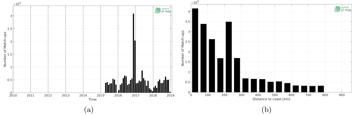
Figure 1: Number of match-ups between TSG-GOSUD-Research-vessel and SMAP-L3-RSS-V4-MONTHLY SSS as a function of time (a) and as function of the distance to coast (b) over the SMOS coastal zone (<800km) 60N-60S Pi-MEP region and for the full satellite product period.
