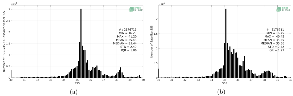
Figure 2: Histograms of SSS from TSG-GOSUD-Research-vessel (a) and SMAP-L3-RSS-V4-MONTHLY (b) considering all match-up pairs per bins of 0.1 over the SMOS coastal zone (<800km) 60N-60S Pi-MEP region and for the full satellite product period.
