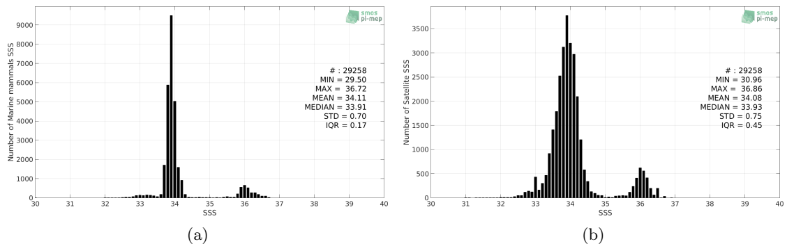
Figure 2: Histograms of SSS from Marine mammals (a) and SMAP SSS L3 v4 - Monthly (RSS) (b) considering all match-up pairs per bins of 0.1 over the SMOS coastal zone (<800km) 60N-60S Pi-MEP region and for the full satellite product period.
