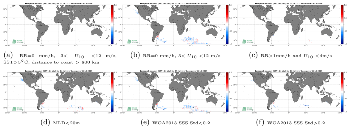
Figure 12: Temporal mean gridded over spatial boxes of size 1^\circ \times 1^\circ of \Delta SSS (SMAP SSS L3 v4 - Monthly (RSS) - Marine mammals) for 6 different subdatasets corresponding to:RR=0 mm/h, 3 < U_{10} < 12 m/s, SST > 5^\circ C , distance to coast > 800 km (a), RR=0 mm/h, 3 < U_{10} < 12 m/s (b), RR>1mm/h and U_{10} < 4 m/s (c),MLD<20m (d),WOA2013 SSS Std<0.2 (e),WOA2013 SSS Std>0.2 (f).
