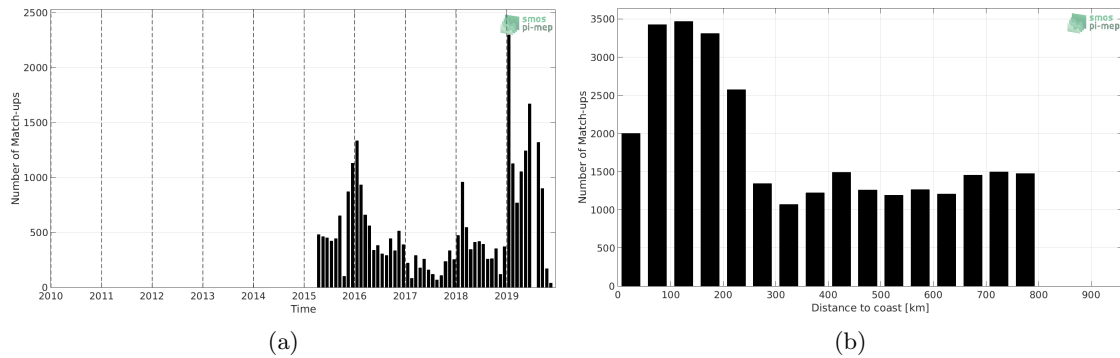
Figure 1: Number of match-ups between Marine mammals and SMAP SSS L3 v4 - Monthly (RSS) SSS as a function of time (a) and as function of the distance to coast (b) over the SMOS coastal zone (<800km) 60N-60S Pi-MEP region and for the full satellite product period.
