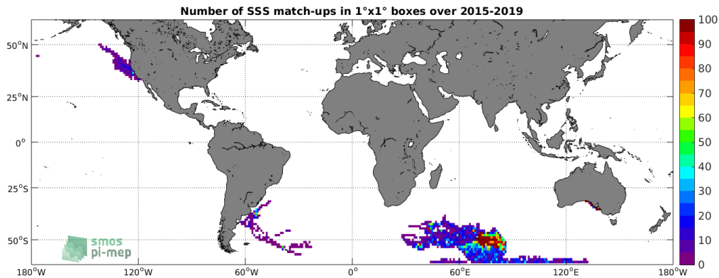
Figure 4: Number of SSS match-ups between Marine mammals SSS and the SMAP SSS L3 v4 - Monthly (RSS) SSS product for the SMOS coastal zone (<800km) 60N-60S Pi-MEP region over 1^\circ \times 1^\circ boxes and for the full satellite product period.
