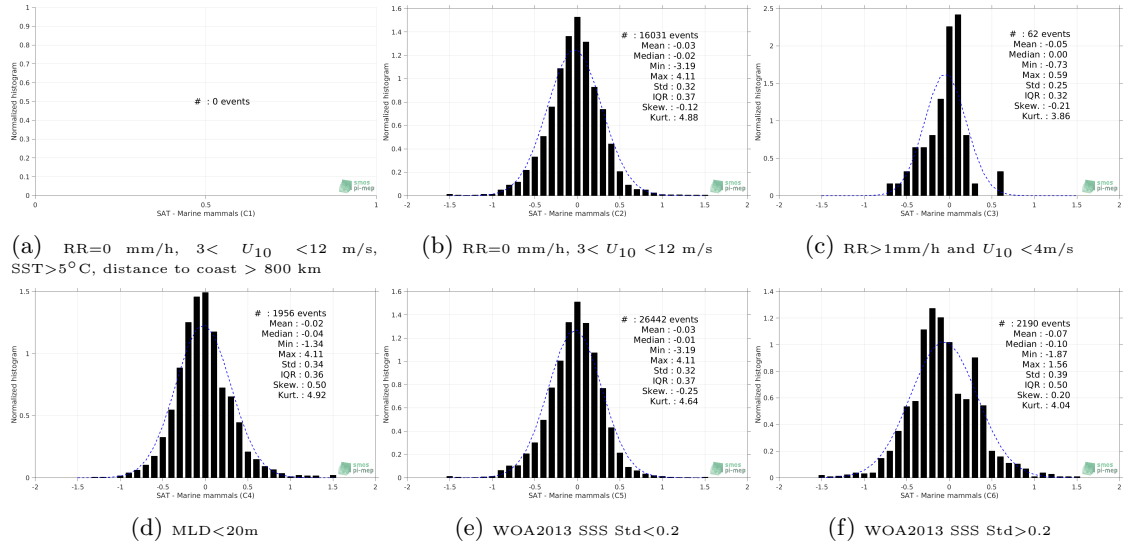
Figure 13: Normalized histogram of \Delta SSS (SMAP SSS L3 v4 - Monthly (RSS) - Marine mammals) for 6 different subdatasets corresponding to: RR=0 mm/h, 3 < U_{10} < 12 m/s, SST>5°C, distance to coast > 800 km (a), RR=0 mm/h, 3 < U_{10} < 12 m/s (b), RR>1mm/h and U_{10} < 4 m/s (c), MLD<20m (d), WOA2013 SSS Std<0.2 (e), WOA2013 SSS Std>0.2 (f).
