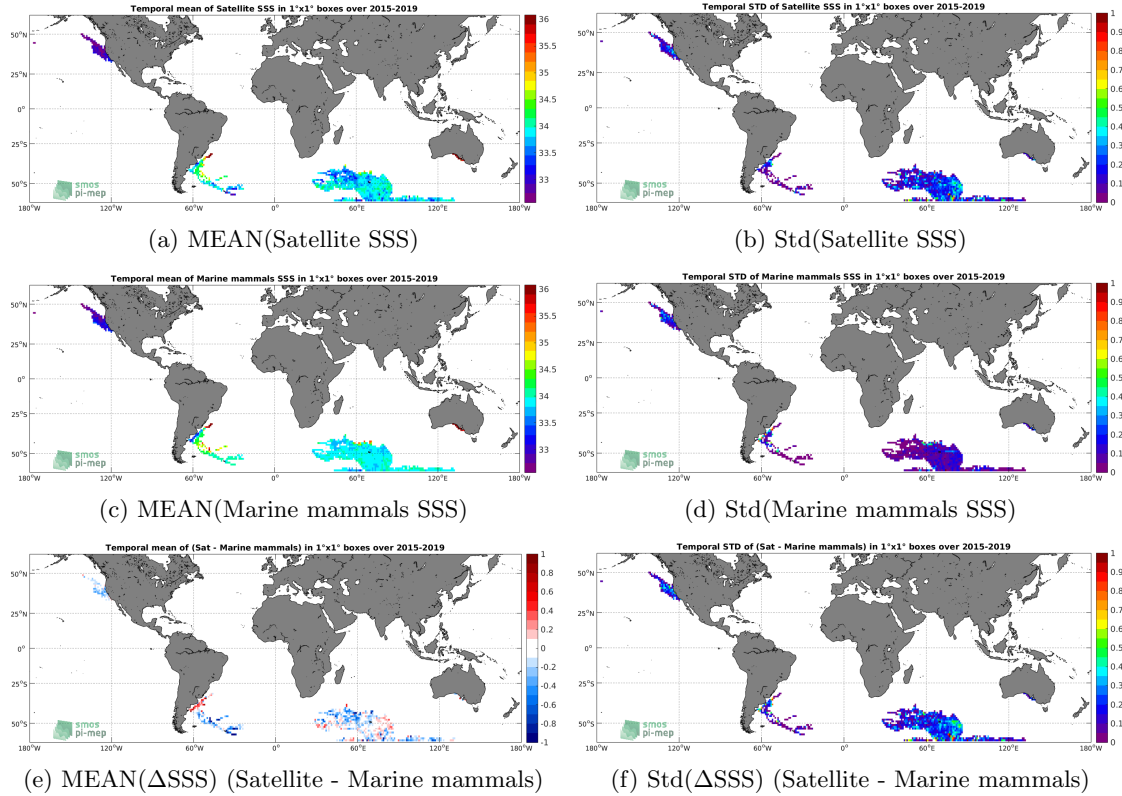
Figure 6: Temporal mean (left) and Std (right) of SSS from SMAP SSS L3 v4 - Monthly (RSS) (top), Marine mammals (middle), and of \Delta SSS (Satellite - Marine mammals). Only match-up pairs are used to generate these maps.
