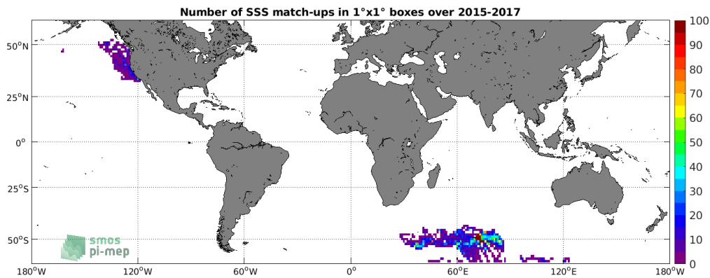
Figure 4: Number of SSS match-ups between Sea mammals SSS and the SMAP SSS L3 v4 - Monthly (RSS) SSS product for the SMOS coastal zone (<800km) 60N-60S Pi-MEP region over 1°x1° boxes and for the full satellite product period.
