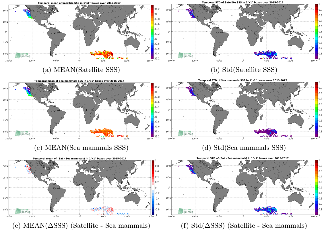
Figure 6: Temporal mean (left) and Std (right) of SSS from SMAP SSS L3 v4 - Monthly (RSS) (top), Sea mammals (middle), and of \Delta SSS (Satellite - Sea mammals). Only match-up pairs are used to generate these maps.
