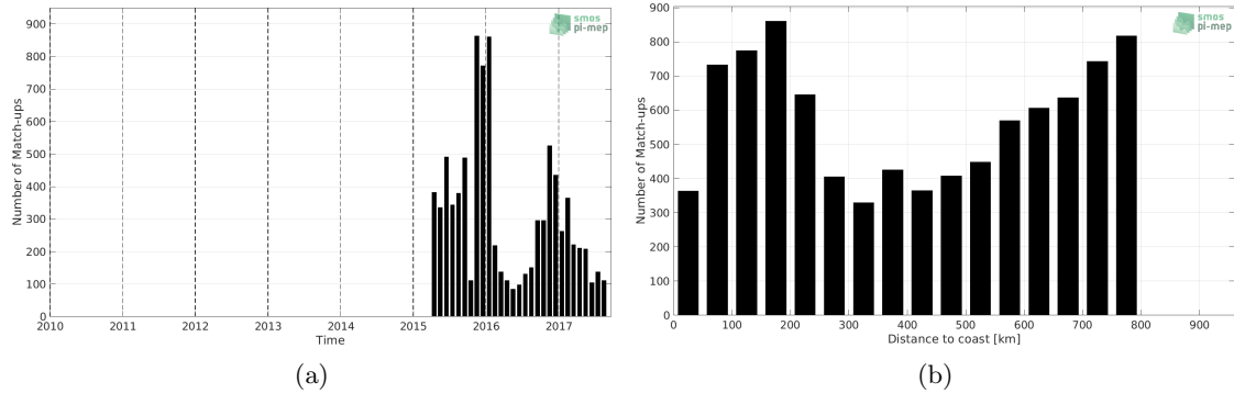
Figure 1: Number of match-ups between Sea mammals and SMAP SSS L3 v4 - Monthly (RSS) SSS as a function of time (a) and as function of the distance to coast (b) over the SMOS coastal zone (<800km) 60N-60S Pi-MEP region and for the full satellite product period.
