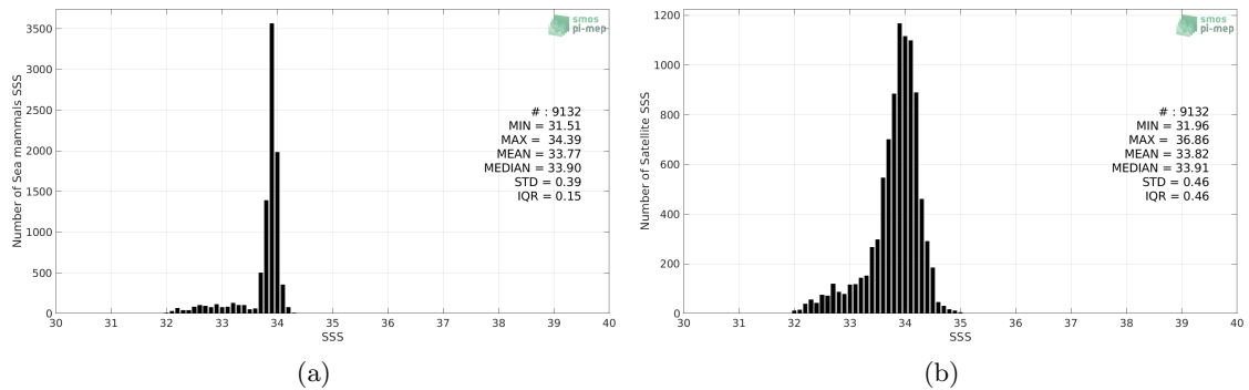
Figure 2: Histograms of SSS from Sea mammals (a) and SMAP SSS L3 v4 - Monthly (RSS) (b) considering all match-up pairs per bins of 0.1 over the SMOS coastal zone (<800km) 60N-60S Pi-MEP region and for the full satellite product period.
