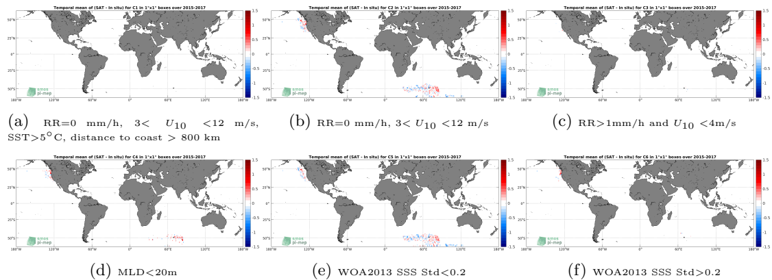
Figure 12: Temporal mean gridded over spatial boxes of size 1^\circ \times 1^\circ of \Delta SSS (SMAP SSS L3 v4 - Monthly (RSS) - Sea mammals) for 6 different subdatasets corresponding to:RR=0 mm/h, 3 < U_{10} < 12 m/s, SST > 5^\circ\text{C} , distance to coast > 800 km (a), RR=0 mm/h, 3 < U_{10} < 12 m/s (b), RR > 1 mm/h and U_{10} < 4 m/s (c),MLD < 20 m (d),WOA2013 SSS Std < 0.2 (e),WOA2013 SSS Std > 0.2 (f).
