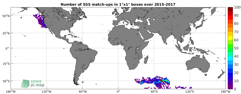
Figure 4: Number of SSS match-ups between Sea mammals SSS and the SMAP-L3-RSS-V4-MONTHLY SSS product for the SMOS coastal zone (<800km) 60N-60S Pi-MEP region over 1°x1° boxes and for the full satellite product period.
