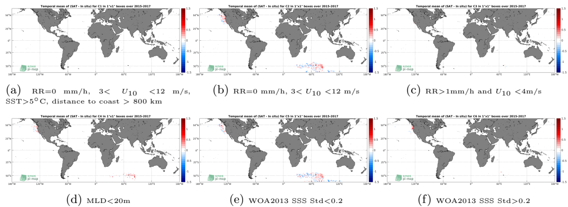
Figure 12: Temporal mean gridded over spatial boxes of size 1^\circ \times 1^\circ of \Delta SSS (SMAP-L3-RSS-V4-MONTHLY - Sea mammals) for 6 different subdatasets corresponding to:RR=0 mm/h, 3 < U_{10} < 12 m/s, SST >5^\circ\text{C} , distance to coast > 800 km (a), RR=0 mm/h, 3 < U_{10} < 12 m/s (b), RR >1 mm/h and U_{10} < 4 m/s (c),MLD <20 m (d),WOA2013 SSS Std <0.2 (e),WOA2013 SSS Std >0.2 (f).
