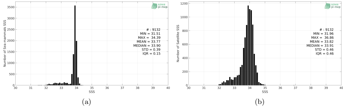
Figure 2: Histograms of SSS from Sea mammals (a) and SMAP-L3-RSS-V4-MONTHLY (b) considering all match-up pairs per bins of 0.1 over the SMOS coastal zone (<800km) 60N-60S Pi-MEP region and for the full satellite product period.
