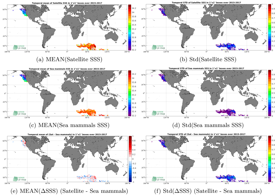
Figure 6: Temporal mean (left) and Std (right) of SSS from SMAP-L3-RSS-V4-MONTHLY (top), Sea mammals (middle), and of \Delta SSS (Satellite - Sea mammals). Only match-up pairs are used to generate these maps.
