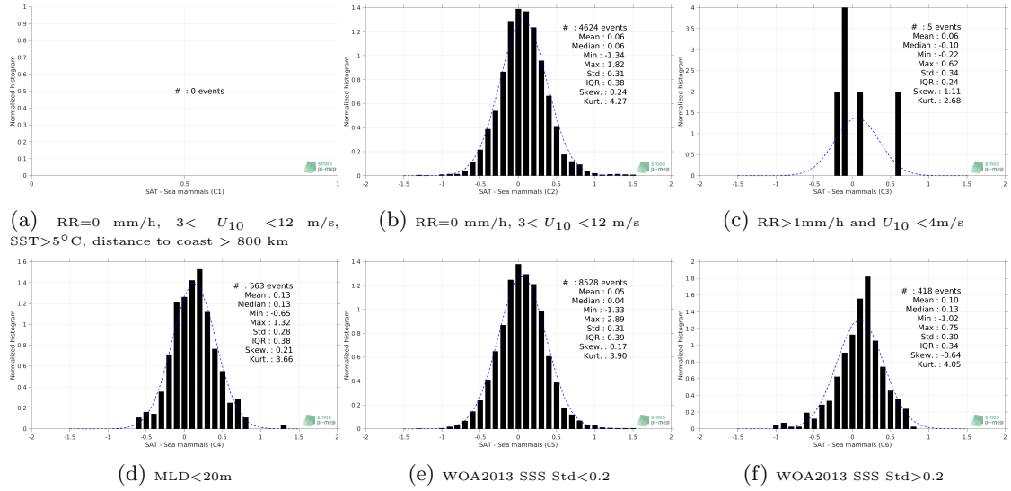
Figure 13: Normalized histogram of \Delta SSS (SMAP-L3-RSS-V4-MONTHLY - Sea mammals) for 6 different subdatasets corresponding to: RR=0 mm/h, 3 < U_{10} < 12 m/s, SST>5°C, distance to coast > 800 km (a), RR=0 mm/h, 3 < U_{10} < 12 m/s (b), RR>1mm/h and U_{10} < 4 m/s (c), MLD<20m (d), WOA2013 SSS Std<0.2 (e), WOA2013 SSS Std>0.2 (f).
