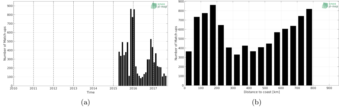
Figure 1: Number of match-ups between Sea mammals and SMAP-L3-RSS-V4-MONTHLY SSS as a function of time (a) and as function of the distance to coast (b) over the SMOS coastal zone (<800km) 60N-60S Pi-MEP region and for the full satellite product period.
