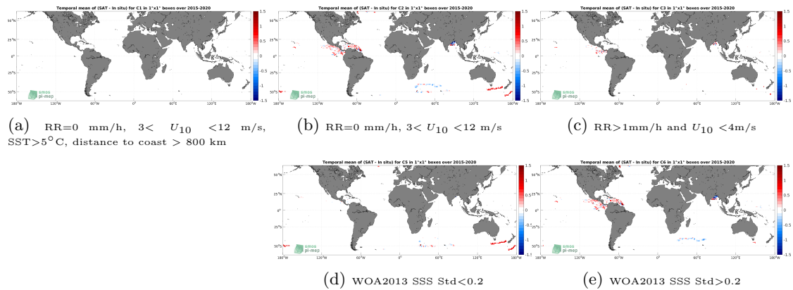
Figure 11: Temporal mean gridded over spatial boxes of size 1^\circ \times 1^\circ of \Delta\text{SSS} (SMAP SSS L3 v4 - Monthly (RSS) - Surface drifters) for 5 different subdatasets corresponding to:RR=0 mm/h, 3 < U_{10} < 12 m/s, SST >5^\circ\text{C} , distance to coast > 800 km (a), RR=0 mm/h, 3 < U_{10} < 12 m/s (b), RR >1 mm/h and U_{10} < 4 m/s (c), WOA2013 SSS Std <0.2 (d), WOA2013 SSS Std >0.2 (e).
