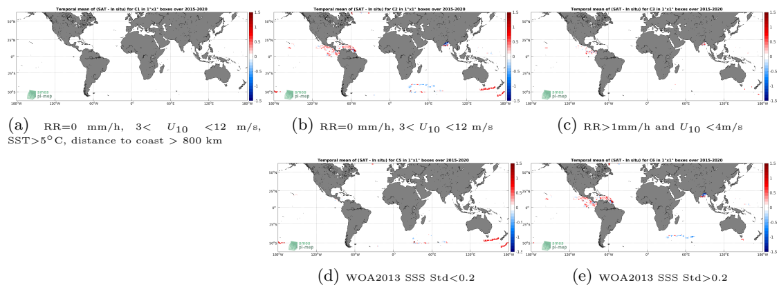
Figure 11: Temporal mean gridded over spatial boxes of size 1^\circ \times 1^\circ of \Delta SSS (SMAP SSS L3 v4 - Monthly (RSS) - Surface drifters) for 5 different subdatasets corresponding to: RR=0 mm/h, 3 < U_{10} < 12 m/s, SST > 5°C, distance to coast > 800 km (a), RR=0 mm/h, 3 < U_{10} < 12 m/s (b), RR > 1mm/h and U_{10} < 4 m/s (c), WOA2013 SSS Std < 0.2 (d), WOA2013 SSS Std > 0.2 (e).
