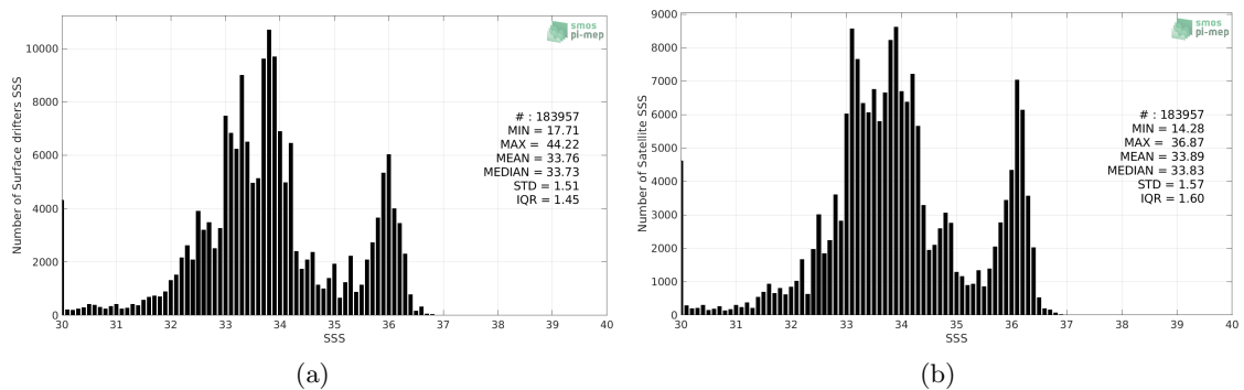
Figure 2: Histograms of SSS from Surface drifters (a) and SMAP SSS L3 v4 - Monthly (RSS) (b) considering all match-up pairs per bins of 0.1 over the SMOS coastal zone (<800km) 60N-60S Pi-MEP region and for the full satellite product period.
