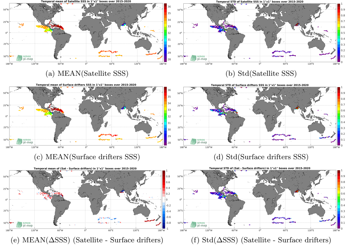
Figure 5: Temporal mean (left) and Std (right) of SSS from SMAP SSS L3 v4 - Monthly (RSS) (top), Surface drifters (middle), and of \Delta SSS (Satellite - Surface drifters). Only match-up pairs are used to generate these maps.
