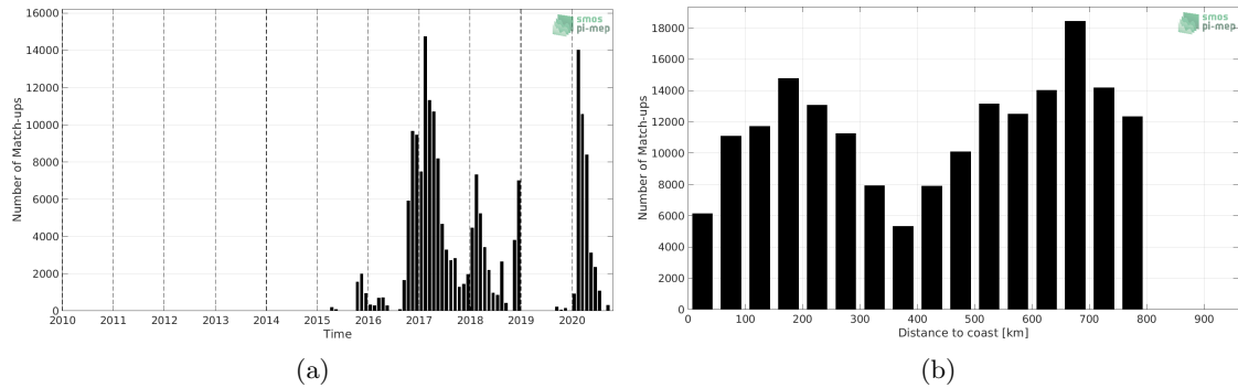
Figure 1: Number of match-ups between Surface drifters and SMAP SSS L3 v4 - Monthly (RSS) SSS as a function of time (a) and as function of the distance to coast (b) over the SMOS coastal zone (<800km) 60N-60S Pi-MEP region and for the full satellite product period.
