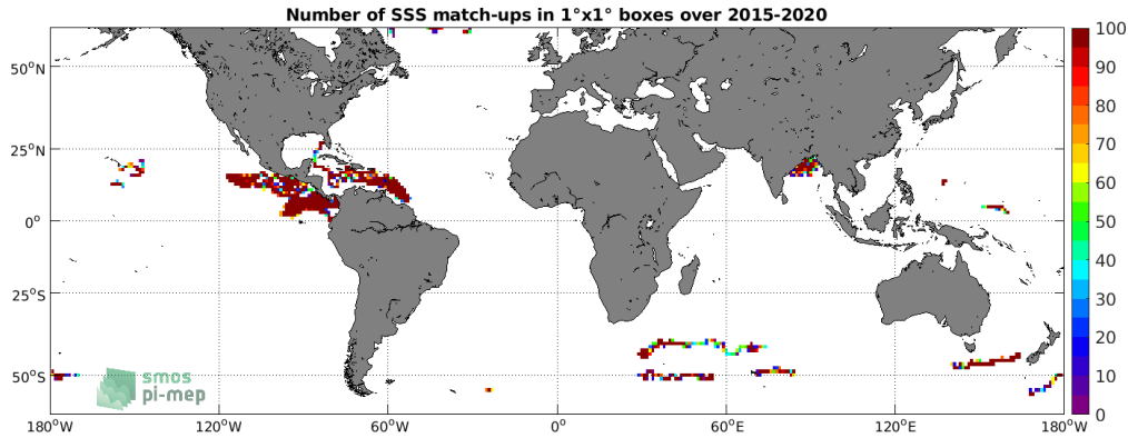
Figure 3: Number of SSS match-ups between Surface drifters SSS and the SMAP SSS L3 v4 - Monthly (RSS) SSS product for the SMOS coastal zone (<800km) 60N-60S Pi-MEP region over 1^\circ \times 1^\circ boxes and for the full satellite product period.
