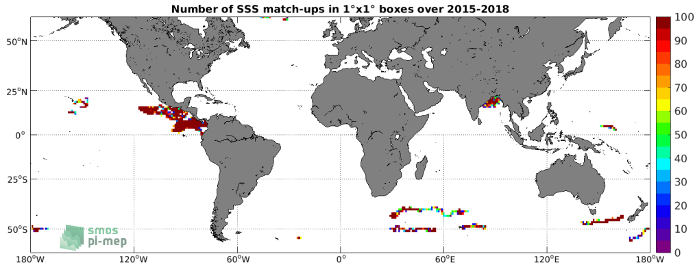
Figure 3: Number of SSS match-ups between Surface drifters SSS and the SMAP SSS L3 v4 - Monthly (RSS) SSS product for the SMOS coastal zone (<800km) 60N-60S Pi-MEP region over 1°x1° boxes and for the full satellite product period.
