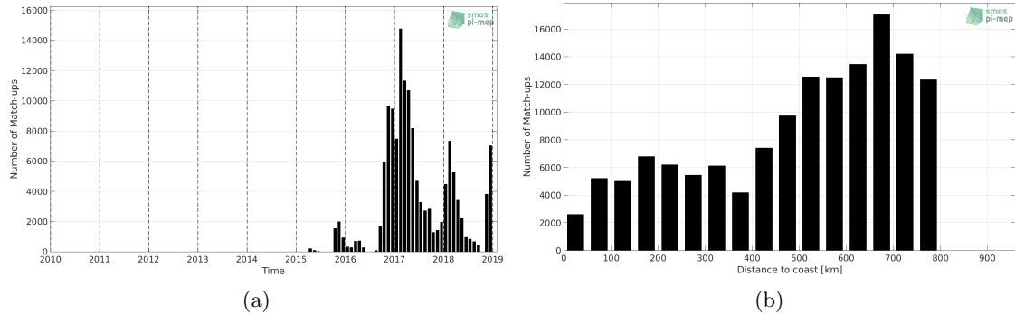
Figure 1: Number of match-ups between Surface drifters and SMAP-L3-RSS-V4-MONTHLY SSS as a function of time (a) and as function of the distance to coast (b) over the SMOS coastal zone (<800km) 60N-60S Pi-MEP region and for the full satellite product period.
