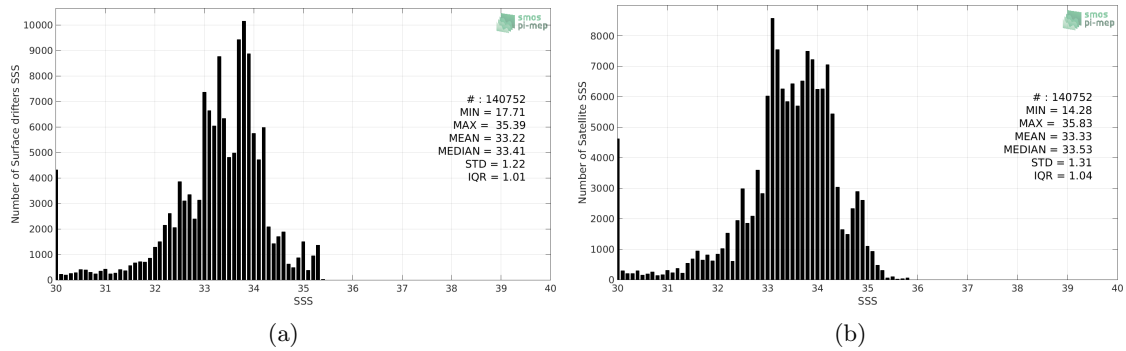
Figure 2: Histograms of SSS from Surface drifters (a) and SMAP-L3-RSS-V4-MONTHLY (b) considering all match-up pairs per bins of 0.1 over the SMOS coastal zone (<800km) 60N-60S Pi-MEP region and for the full satellite product period.
