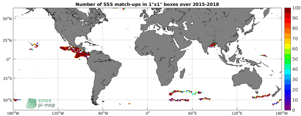
Figure 3: Number of SSS match-ups between Surface drifters SSS and the SMAP-L3-RSS-V4-MONTHLY SSS product for the SMOS coastal zone (<800km) 60N-60S Pi-MEP region over 1°x1° boxes and for the full satellite product period.
