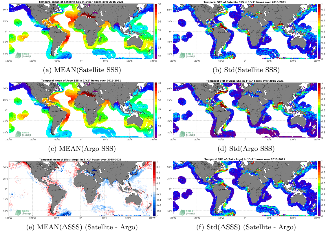
Figure 6: Temporal mean (left) and Std (right) of SSS from SMAP SSS L3 v4 - Monthly (RSS) (top), Argo (middle), and of \Delta SSS (Satellite - Argo). Only match-up pairs are used to generate these maps.
