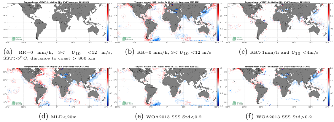
Figure 12: Temporal mean gridded over spatial boxes of size 1^\circ \times 1^\circ of \Delta SSS (SMAP SSS L3 v4 - Monthly (RSS) - Argo) for 6 different subdatasets corresponding to: RR=0 mm/h, 3 < U_{10} < 12 m/s, SST > 5^\circ\text{C} , distance to coast > 800 km (a), RR=0 mm/h, 3 < U_{10} < 12 m/s (b), RR > 1 mm/h and U_{10} < 4 m/s (c), MLD < 20 m (d), WOA2013 SSS Std < 0.2 (e), WOA2013 SSS Std > 0.2 (f).
