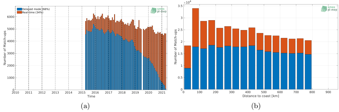
Figure 1: Number of match-ups between Argo and SMAP SSS L3 v4 - Monthly (RSS) SSS as a function of time (a) and as function of the distance to coast (b) over the SMOS coastal zone (<800km) 60N-60S Pi-MEP region and for the full satellite product period.
