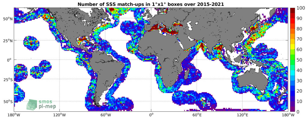
Figure 4: Number of SSS match-ups between Argo SSS and the SMAP SSS L3 v4 - Monthly (RSS) SSS product for the SMOS coastal zone (<800km) 60N-60S Pi-MEP region over 1^\circ \times 1^\circ boxes and for the full satellite product period.
