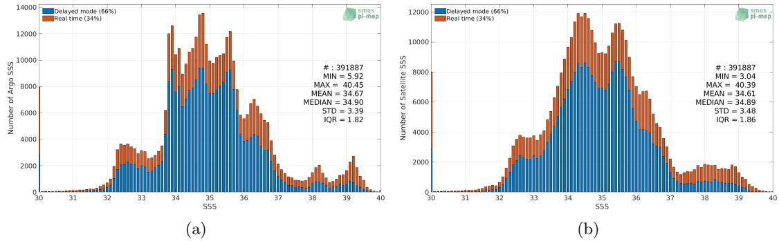
Figure 2: Histograms of SSS from Argo (a) and SMAP SSS L3 v4 - Monthly (RSS) (b) considering all match-up pairs per bins of 0.1 over the SMOS coastal zone (<800km) 60N-60S Pi-MEP region and for the full satellite product period.
