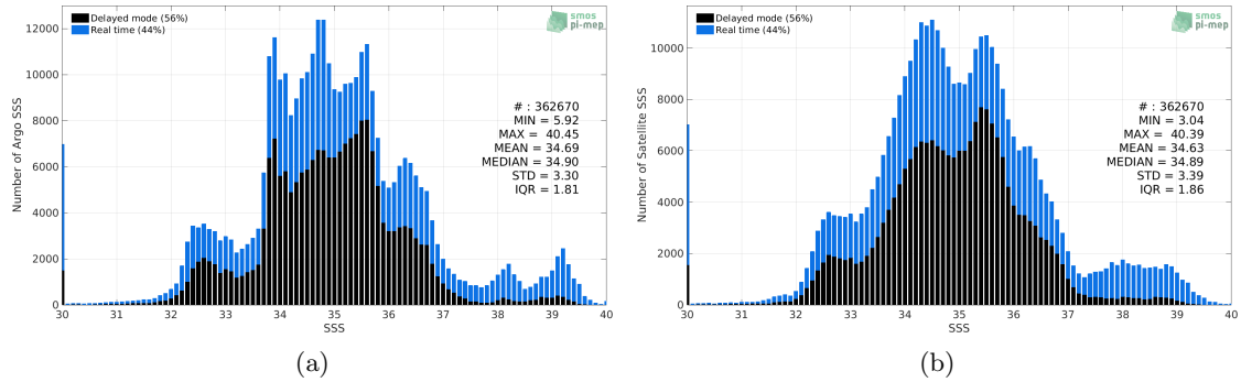
Figure 2: Histograms of SSS from Argo (a) and SMAP SSS L3 v4 - Monthly (RSS) (b) considering all match-up pairs per bins of 0.1 over the SMOS coastal zone (<800km) 60N-60S Pi-MEP region and for the full satellite product period.
