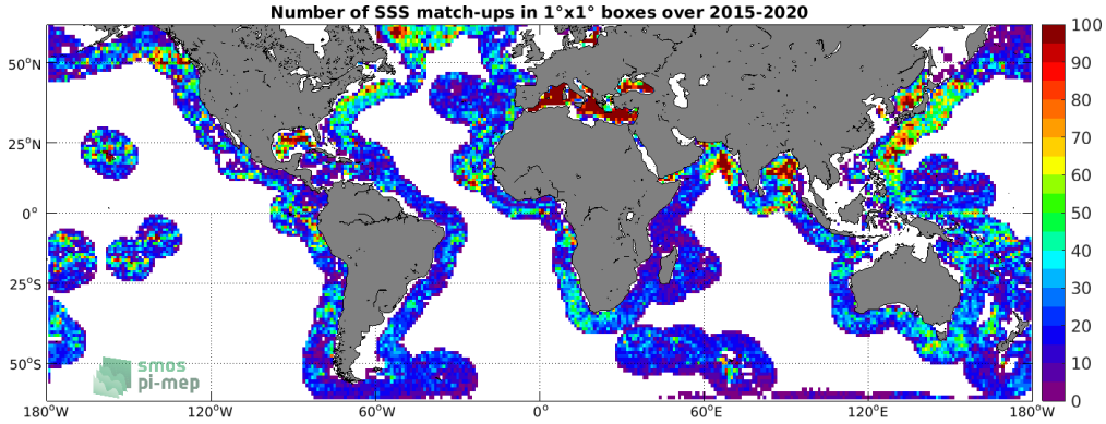
Figure 4: Number of SSS match-ups between Argo SSS and the SMAP SSS L3 v4 - Monthly (RSS) SSS product for the SMOS coastal zone (<800km) 60N-60S Pi-MEP region over 1°x1° boxes and for the full satellite product period.
