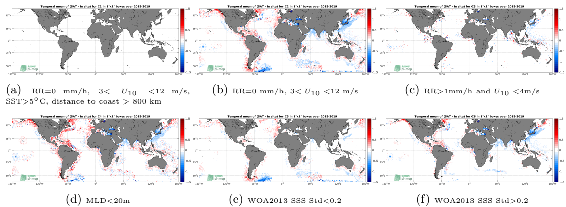
Figure 12: Temporal mean gridded over spatial boxes of size 1^\circ \times 1^\circ of \Delta SSS (SMAP-L3-RSS-V4-MONTHLY - Argo) for 6 different subdatasets corresponding to:RR=0 mm/h, 3 < U_{10} < 12 m/s, SST >5^\circ C, distance to coast > 800 km (a), RR=0 mm/h, 3 < U_{10} < 12 m/s (b), RR >1 mm/h and U_{10} < 4 m/s (c),MLD <20 m (d),WOA2013 SSS Std <0.2 (e),WOA2013 SSS Std >0.2 (f).
