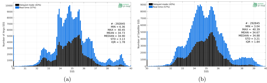
Figure 2: Histograms of SSS from Argo (a) and SMAP-L3-RSS-V4-MONTHLY (b) considering all match-up pairs per bins of 0.1 over the SMOS coastal zone ( \pm 800 km) 60N-60S Pi-MEP region and for the full satellite product period.
