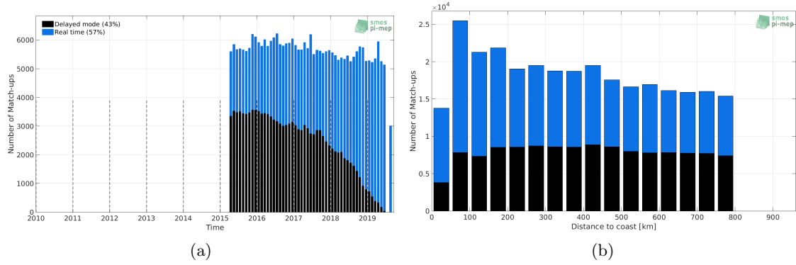
Figure 1: Number of match-ups between Argo and SMAP-L3-RSS-V4-MONTHLY SSS as a function of time (a) and as function of the distance to coast (b) over the SMOS coastal zone ( \pm 800 km) 60N-60S Pi-MEP region and for the full satellite product period.
