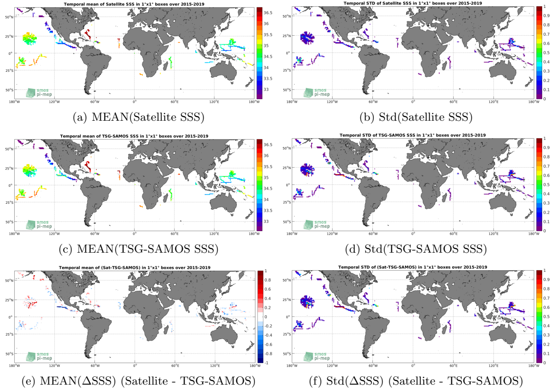
Figure 6: Temporal mean (left) and Std (right) of SSS from SMAP-L3-RSS-V3-8DAY-RUNNING-70KM (top), TSG-SAMOS (middle), and of \Delta SSS (Satellite - TSG-SAMOS). Only match-up pairs are used to generate these maps.
