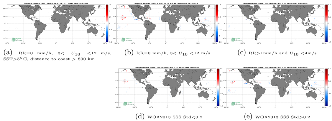
Figure 12: Temporal mean gridded over spatial boxes of size 1^\circ \times 1^\circ of \Delta SSS (SMAP-L3-RSS-V3-8DAY-RUNNING-70KM - TSG-SAMOS) for 5 different subdatasets corresponding to:RR=0 mm/h, 3 < U_{10} < 12 m/s, SST >5^\circ C, distance to coast > 800 km (a), RR=0 mm/h, 3 < U_{10} < 12 m/s (b), RR >1 mm/h and U_{10} < 4 m/s (c), WOA2013 SSS Std <0.2 (d), WOA2013 SSS Std >0.2 (e).
