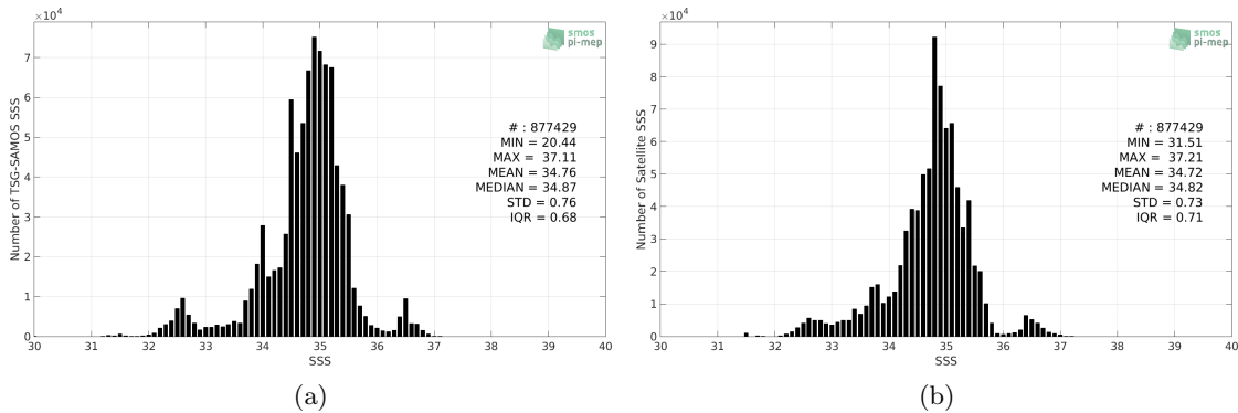
Figure 2: Histograms of SSS from TSG-SAMOS (a) and SMAP-L3-RSS-V3-8DAY-RUNNING-70KM (b) considering all match-up pairs per bins of 0.1 over the SMOS coastal zone ( \geq 800 km) 60N-60S Pi-MEP region and for the full satellite product period.
