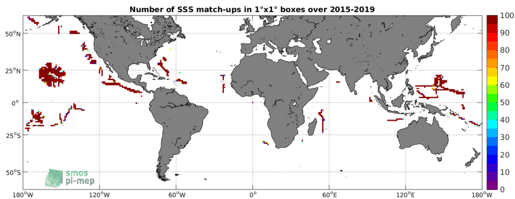
Figure 4: Number of SSS match-ups between TSG-SAMOS SSS and the SMAP-L3-RSS-V3-8DAY-RUNNING-70KM SSS product for the SMOS coastal zone ( \pm 800\text{km} ) 60N-60S Pi-MEP region over 1^\circ \times 1^\circ boxes and for the full satellite product period.
