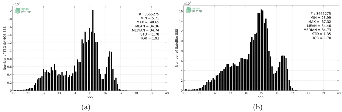
Figure 2: Histograms of SSS from TSG-SAMOS (a) and SMAP-L3-RSS-V3-8DAY-RUNNING-70KM (b) considering all match-up pairs per bins of 0.1 over the SMOS coastal zone ( \approx 800\text{km} ) 60N-60S Pi-MEP region and for the full satellite product period.
