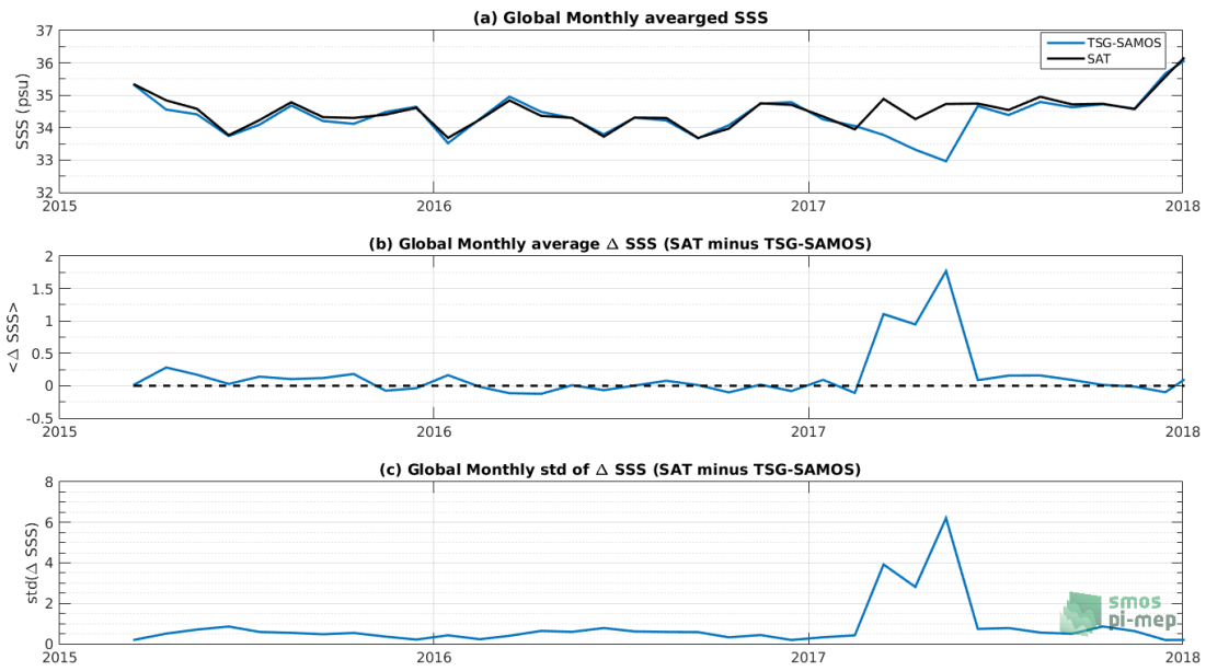
Figure 7: Time series of the monthly averaged mean SSS (top), mean \Delta SSS (Satellite - TSG-SAMOS) and STD of \Delta SSS (Satellite - TSG-SAMOS) over the SMOS coastal zone ( \approx 800 km) 60N-60S Pi-MEP region considering all match-ups collected by the Pi-MEP platform.
