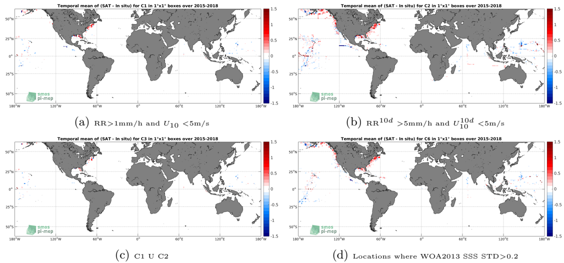
Figure 12: Temporal mean gridded over spatial boxes of size 1^\circ \times 1^\circ of \Delta SSS (SMAP-L3-RSS-V3-8DAY-RUNNING-70KM - TSG-SAMOS) for 4 different subdatasets corresponding to: RR > 1\text{mm/h} and U_{10} < 5\text{m/s} (a), RR^{10d} > 5\text{mm/h} and U_{10}^{10d} < 5\text{m/s} (b), C1 U C2 (c), Locations where WOA2013 SSS STD > 0.2 (d).
