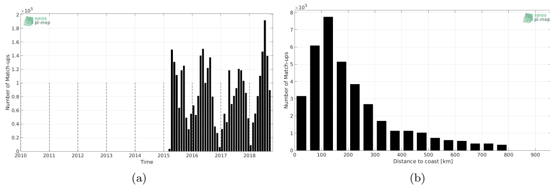
Figure 1: Number of match-ups between TSG-SAMOS and SMAP-L3-RSS-V3-8DAY-RUNNING-70KM SSS as a function of time (a) and as function of the distance to coast (b) over the SMOS coastal zone ( \approx 800 km) 60N-60S Pi-MEP region and for the full satellite product period.
