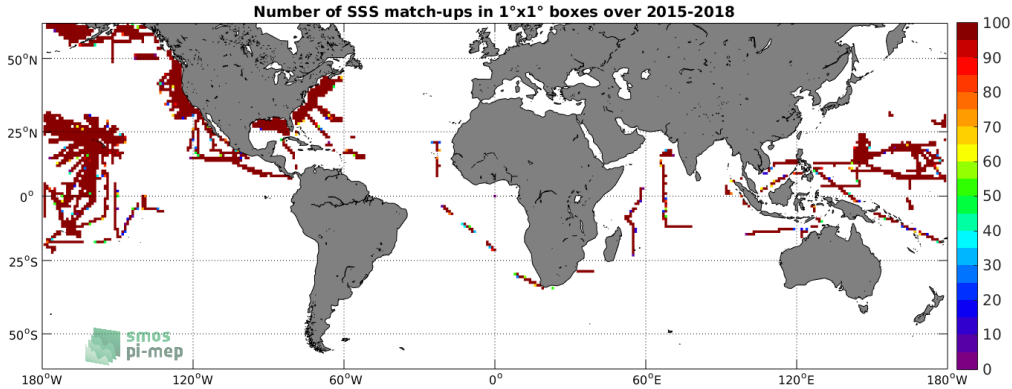
Figure 4: Number of SSS match-ups between TSG-SAMOS SSS and the SMAP-L3-RSS-V3-8DAY-RUNNING-70KM SSS product for the SMOS coastal zone ( \approx 800\text{km} ) 60N-60S Pi-MEP region over 1°x1° boxes and for the full satellite product period.
