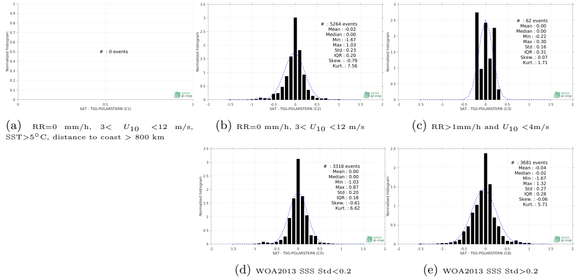
Figure 13: Normalized histogram of \Delta SSS (SMAP-L3-RSS-V3-8DAY-RUNNING-70KM - TSG-POLARSTERN) for 5 different subdatasets corresponding to: RR=0 mm/h, 3 < U_{10} < 12 m/s, SST > 5°C, distance to coast > 800 km (a), RR=0 mm/h, 3 < U_{10} < 12 m/s (b), RR > 1mm/h and U_{10} < 4 m/s (c), WOA2013 SSS Std < 0.2 (d), WOA2013 SSS Std > 0.2 (e).
