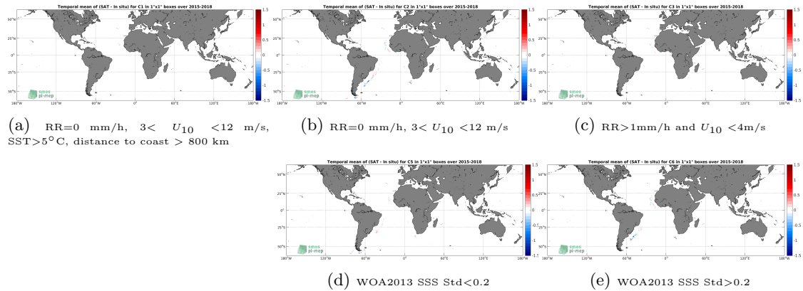
Figure 12: Temporal mean gridded over spatial boxes of size 1^\circ \times 1^\circ of \Delta SSS (SMAP-L3-RSS-V3-8DAY-RUNNING-70KM - TSG-POLARSTERN) for 5 different subdatasets corresponding to:RR=0 mm/h, 3 < U_{10} < 12 m/s, SST >5^\circ C, distance to coast > 800 km (a), RR=0 mm/h, 3 < U_{10} < 12 m/s (b), RR >1 mm/h and U_{10} < 4 m/s (c), WOA2013 SSS Std <0.2 (d), WOA2013 SSS Std >0.2 (e).
