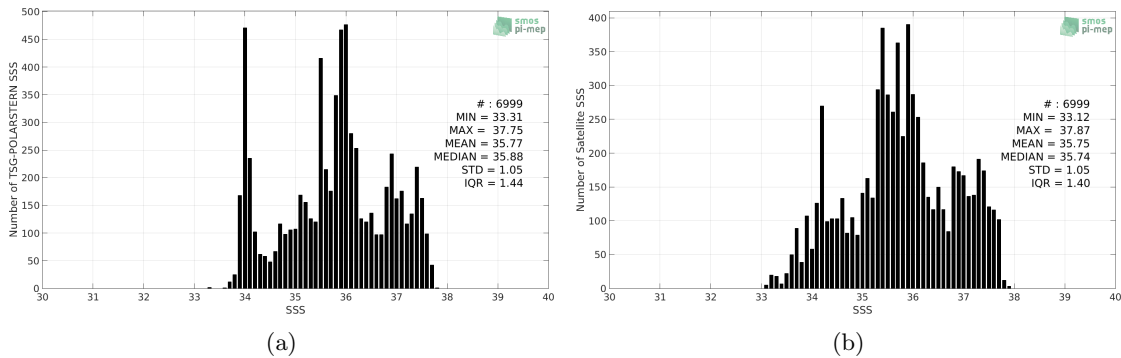
Figure 2: Histograms of SSS from TSG-POLARSTERN (a) and SMAP-L3-RSS-V3-8DAY-RUNNING-70KM (b) considering all match-up pairs per bins of 0.1 over the SMOS coastal zone ( \approx 800\text{km} ) 60N-60S Pi-MEP region and for the full satellite product period.
