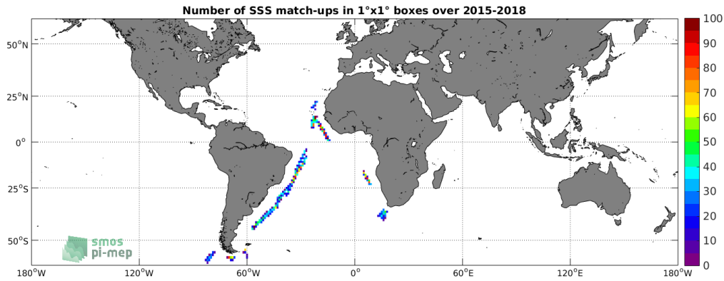
Figure 4: Number of SSS match-ups between TSG-POLARSTERN SSS and the SMAP-L3-RSS-V3-8DAY-RUNNING-70KM SSS product for the SMOS coastal zone ( \pm 800\text{km} ) 60N-60S Pi-MEP region over 1^\circ \times 1^\circ boxes and for the full satellite product period.
