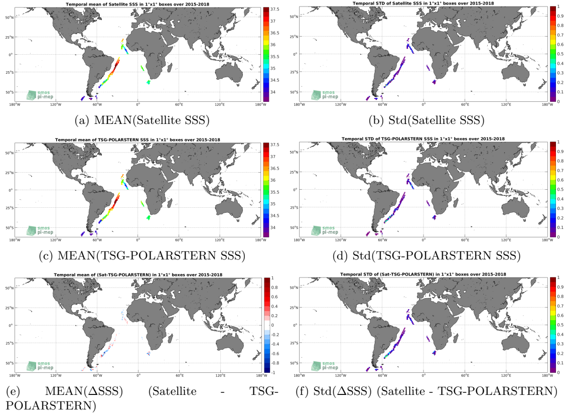
Figure 6: Temporal mean (left) and Std (right) of SSS from SMAP-L3-RSS-V3-8DAY-RUNNING-70KM (top), TSG-POLARSTERN (middle), and of \Delta SSS (Satellite - TSG-POLARSTERN). Only match-up pairs are used to generate these maps.
