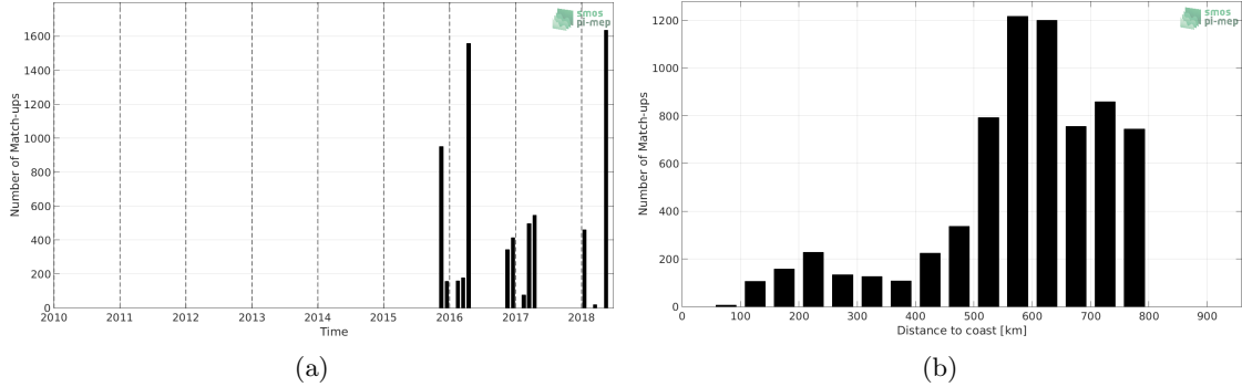
Figure 1: Number of match-ups between TSG-POLARSTERN and SMAP-L3-RSS-V3-8DAY-RUNNING-70KM SSS as a function of time (a) and as function of the distance to coast (b) over the SMOS coastal zone ( \approx 800\text{km} ) 60N-60S Pi-MEP region and for the full satellite product period.
