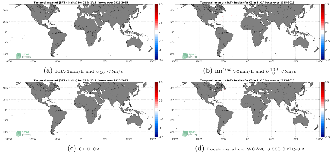
Figure 12: Temporal mean gridded over spatial boxes of size 1^\circ \times 1^\circ of \Delta SSS (SMAP-L3-RSS-V3-8DAY-RUNNING-70KM - TSG-GOSUD-Sailing-ship) for 4 different subdatasets corresponding to: RR > 1mm/h and U_{10} < 5\text{m/s} (a), RR^{10d} > 5\text{mm/h} and U_{10}^{10d} < 5\text{m/s} (b), C1 U C2 (c), Locations where WOA2013 SSS STD > 0.2 (d).
