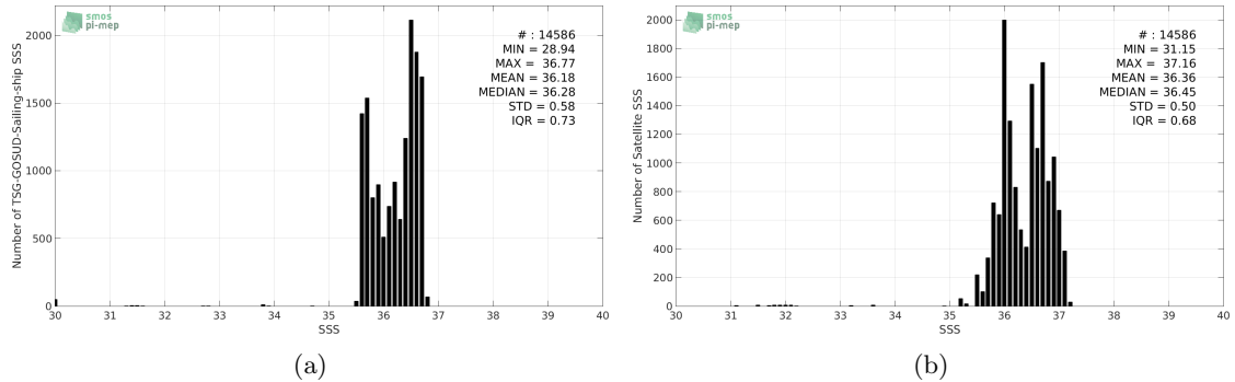
Figure 2: Histograms of SSS from TSG-GOSUD-Sailing-ship (a) and SMAP-L3-RSS-V3-8DAY-RUNNING-70KM (b) considering all match-up pairs per bins of 0.1 over the SMOS coastal zone ( \pm 800\text{km} ) 60N-60S Pi-MEP region and for the full satellite product period.
