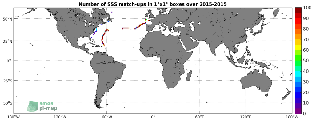
Figure 4: Number of SSS match-ups between TSG-GOSUD-Sailing-ship SSS and the SMAP-L3-RSS-V3-8DAY-RUNNING-70KM SSS product for the SMOS coastal zone ( \approx 800\text{km} ) 60\text{N}-60\text{S} Pi-MEP region over 1^\circ \times 1^\circ boxes and for the full satellite product period.
