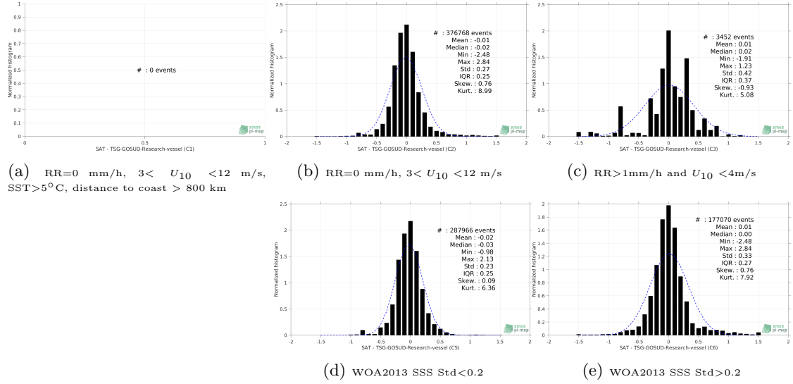
Figure 13: Normalized histogram of \Delta SSS (SMAP-L3-RSS-V3-8DAY-RUNNING-70KM - TSG-GOSUD-Research-vessel) for 5 different subdatasets corresponding to: RR=0 mm/h, 3 < U_{10} < 12 m/s, SST>5°C, distance to coast > 800 km (a), RR=0 mm/h, 3 < U_{10} < 12 m/s (b), RR>1mm/h and U_{10} < 4 m/s (c), WOA2013 SSS Std<0.2 (d), WOA2013 SSS Std>0.2 (e).
