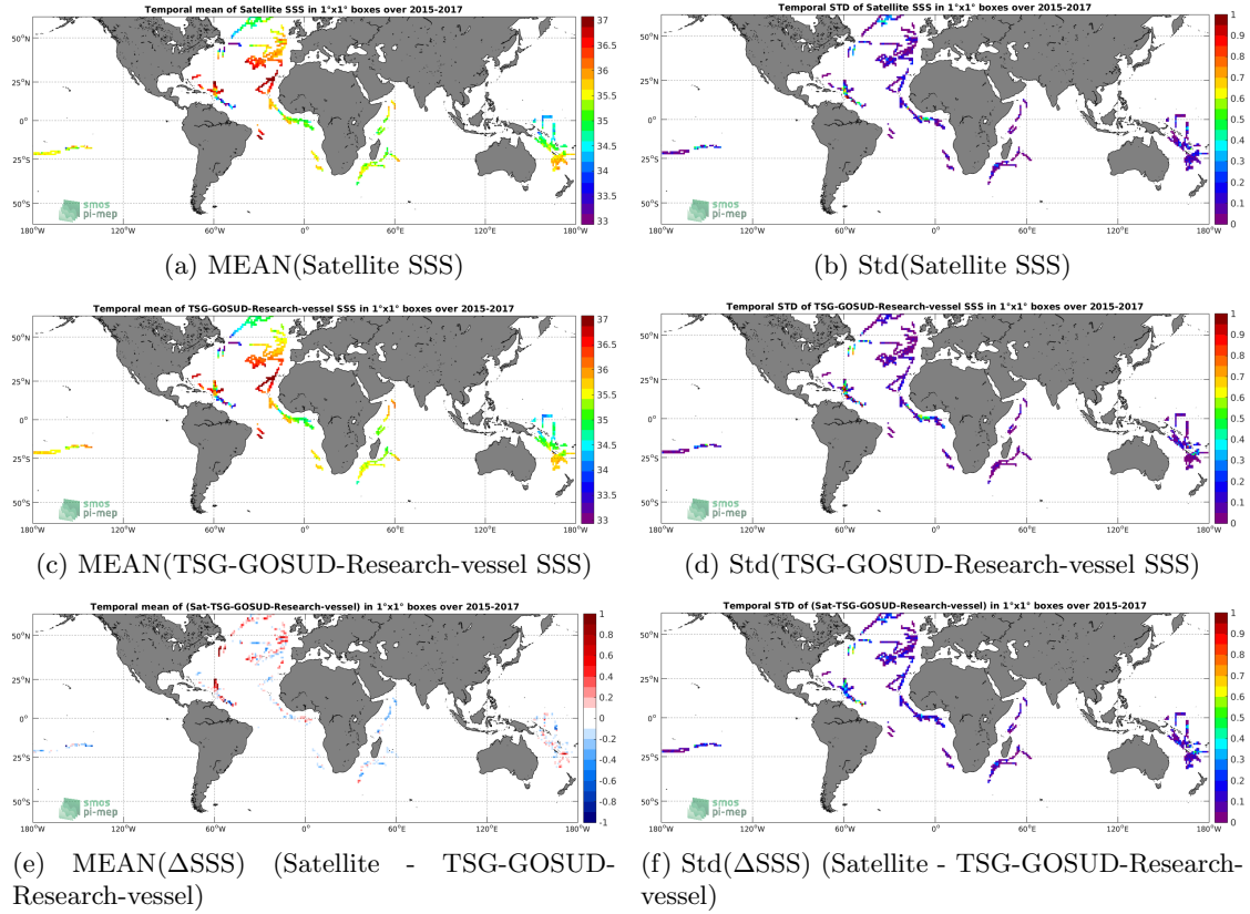
Figure 6: Temporal mean (left) and Std (right) of SSS from SMAP-L3-RSS-V3-8DAY-RUNNING-70KM (top), TSG-GOSUD-Research-vessel (middle), and of \Delta SSS (Satellite - TSG-GOSUD-Research-vessel). Only match-up pairs are used to generate these maps.
