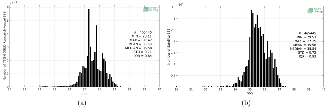
Figure 2: Histograms of SSS from TSG-GOSUD-Research-vessel (a) and SMAP-L3-RSS-V3-8DAY-RUNNING-70KM (b) considering all match-up pairs per bins of 0.1 over the SMOS coastal zone ( \approx 800\text{km} ) 60N-60S Pi-MEP region and for the full satellite product period.
