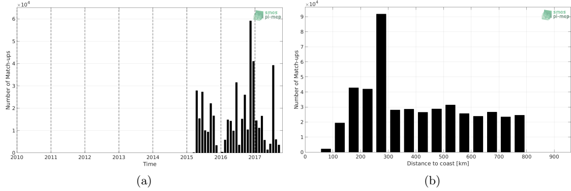
Figure 1: Number of match-ups between TSG-GOSUD-Research-vessel and SMAP-L3-RSS-V3-8DAY-RUNNING-70KM SSS as a function of time (a) and as function of the distance to coast (b) over the SMOS coastal zone ( \approx 800\text{km} ) 60N-60S Pi-MEP region and for the full satellite product period.
