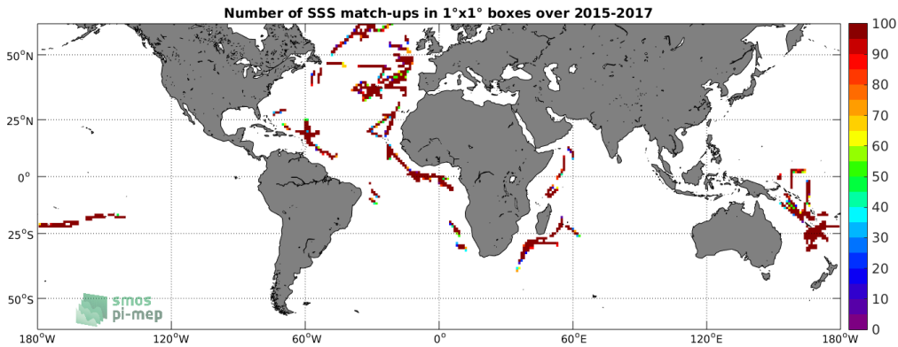
Figure 4: Number of SSS match-ups between TSG-GOSUD-Research-vessel SSS and the SMAP-L3-RSS-V3-8DAY-RUNNING-70KM SSS product for the SMOS coastal zone ( \approx 800 km) 60N-60S Pi-MEP region over 1^\circ \times 1^\circ boxes and for the full satellite product period.
