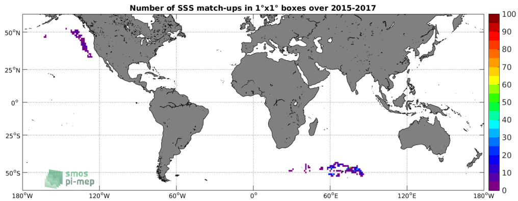
Figure 4: Number of SSS match-ups between Sea mammals SSS and the SMAP-L3-RSS-V3-8DAY-RUNNING-70KM SSS product for the SMOS coastal zone ( \approx 800\text{km} ) 60N-60S Pi-MEP region over 1^\circ \times 1^\circ boxes and for the full satellite product period.
