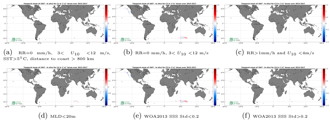
Figure 12: Temporal mean gridded over spatial boxes of size 1^\circ \times 1^\circ of \Delta SSS (SMAP-L3-RSS-V3-8DAY-RUNNING-70KM - Sea mammals) for 6 different subdatasets corresponding to:RR=0 mm/h, 3 < U_{10} < 12 m/s, SST >5^\circ C, distance to coast > 800 km (a), RR=0 mm/h, 3 < U_{10} < 12 m/s (b), RR >1 mm/h and U_{10} < 4 m/s (c),MLD <20 m (d),WOA2013 SSS Std <0.2 (e),WOA2013 SSS Std >0.2 (f).
