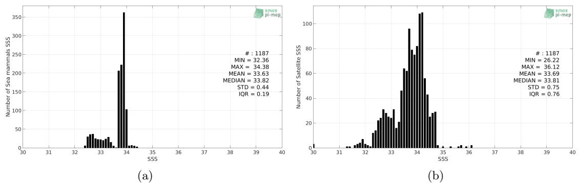
Figure 2: Histograms of SSS from Sea mammals (a) and SMAP-L3-RSS-V3-8DAY-RUNNING-70KM (b) considering all match-up pairs per bins of 0.1 over the SMOS coastal zone ( \approx 800\text{km} ) 60N-60S Pi-MEP region and for the full satellite product period.
