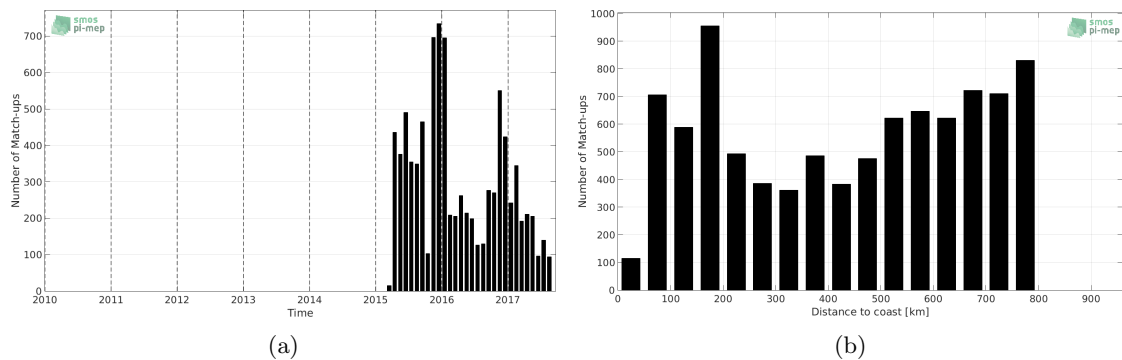
Figure 1: Number of match-ups between Sea mammals and SMAP-L3-RSS-V3-8DAY-RUNNING-70KM SSS as a function of time (a) and as function of the distance to coast (b) over the SMOS coastal zone ( \approx 800 km) 60N-60S Pi-MEP region and for the full satellite product period.
