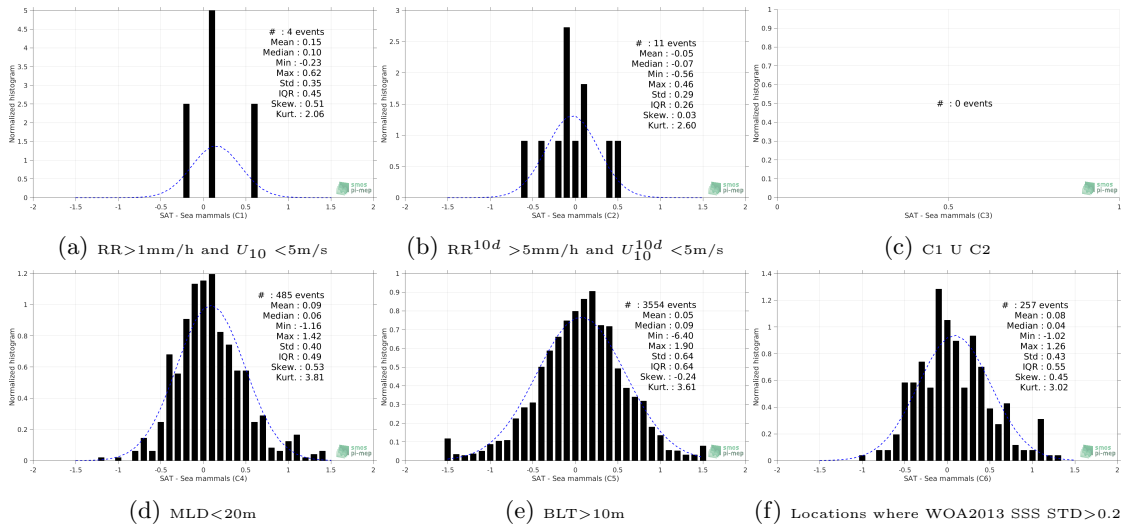
Figure 13: Normalized histogram of \Delta SSS (SMAP-L3-RSS-V3-8DAY-RUNNING-70KM - Sea mammals) for 6 different subdatasets corresponding to: RR>1mm/h and U_{10} < 5m/s (a), RR^{10d} > 5mm/h and U_{10}^{10d} < 5m/s (b), C1 U C2 (c),MLD<20m (d),BLT>10m (e),Locations where WOA2013 SSS STD>0.2 (f).
