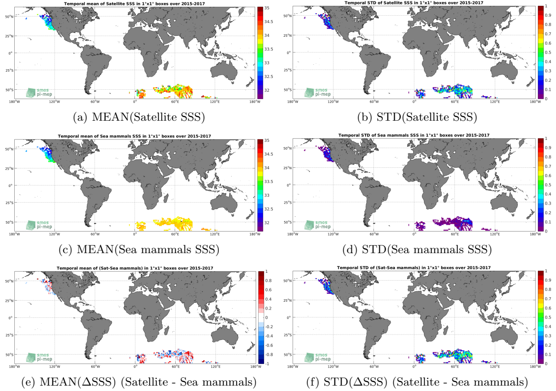
Figure 6: Temporal mean (left) and STD (right) of SSS from SMAP-L3-RSS-V3-8DAY-RUNNING-70KM (top), Sea mammals (middle), and of \Delta SSS (Satellite - Sea mammals). Only match-up pairs are used to generate these maps.
