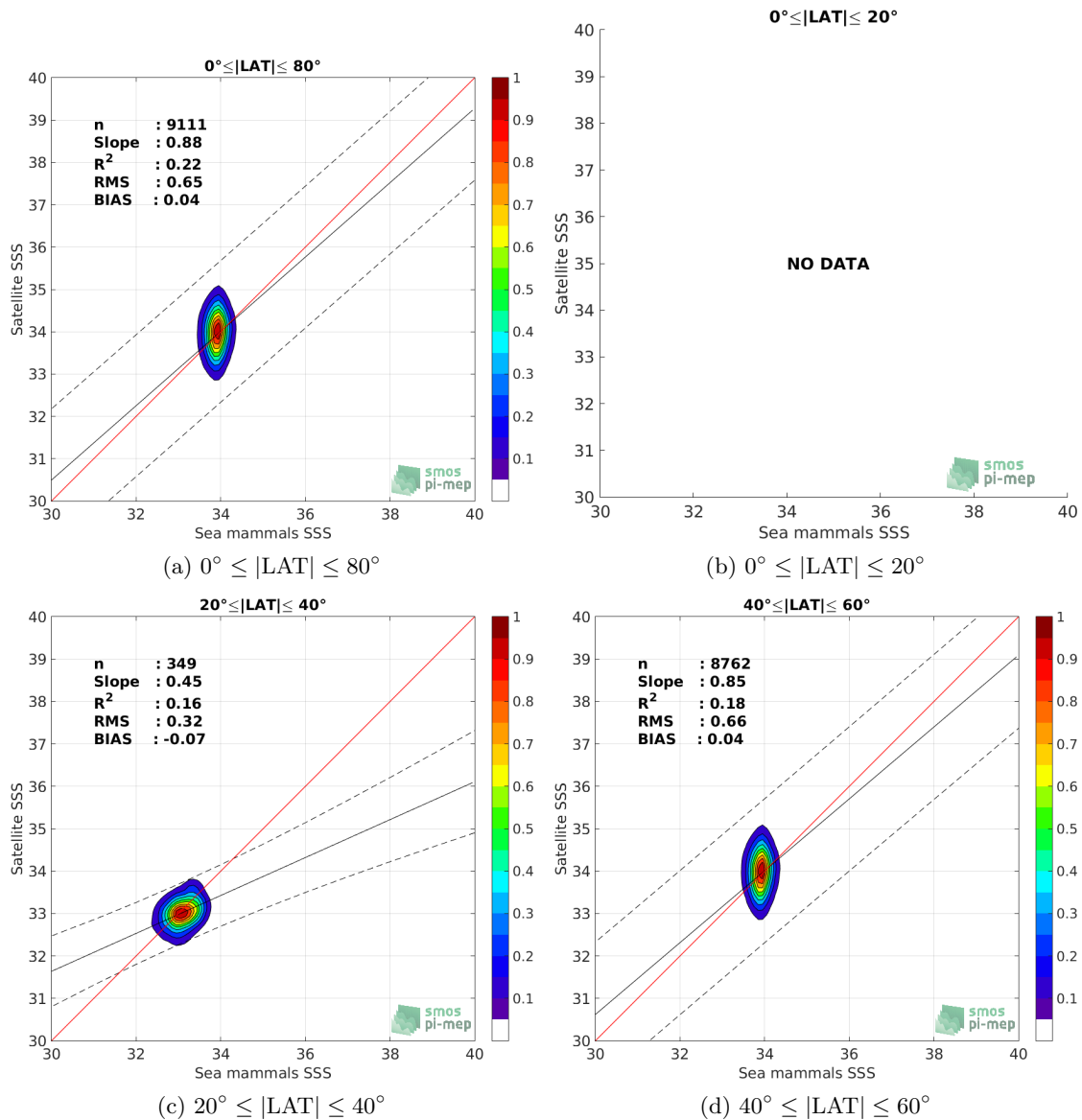
Figure 9: Contour maps of the concentration of SMAP-L3-RSS-V3-8DAY-RUNNING-70KM SSS (y-axis) versus Sea mammals SSS (x-axis) at match-up pairs for different latitudinal bands. For each plot, the red line shows x=y . The black thin and dashed lines indicate a linear fit through the data cloud and the \pm 95\% confidence levels, respectively. The number match-up pairs n , the slope and R^2 coefficient of the linear fit, the root mean square (RMS) and the mean bias between satellite and in situ data are indicated for each latitude band in each plots.
