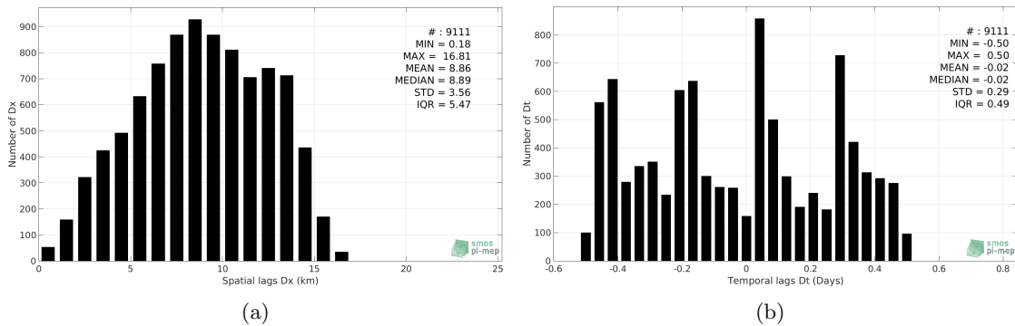
Figure 5: Histograms of the spatial (a) and temporal (b) lags between the time of the Sea mammals measurements and the date of the corresponding SMAP-L3-RSS-V3-8DAY-RUNNING-70KM SSS product.
