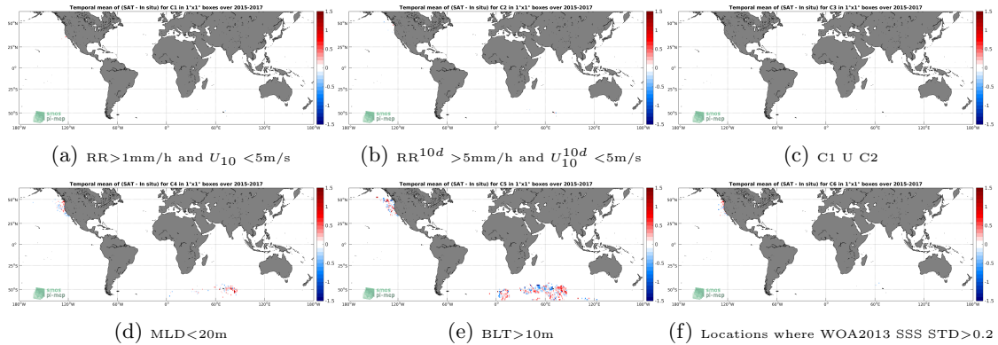
Figure 12: Temporal mean gridded over spatial boxes of size 1^\circ \times 1^\circ of \Delta SSS (SMAP-L3-RSS-V3-8DAY-RUNNING-70KM - Sea mammals) for 6 different subdatasets corresponding to: RR>1mm/h and U_{10} < 5m/s (a), RR^{10d} > 5mm/h and U_{10}^{10d} < 5m/s (b), C1 U C2 (c),MLD<20m (d),BLT>10m (e),Locations where WOA2013 SSS STD>0.2 (f).
