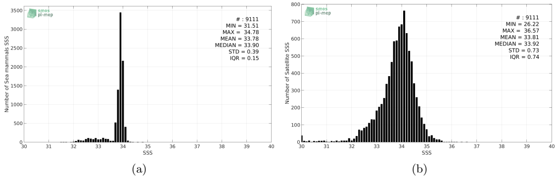
Figure 2: Histograms of SSS from Sea mammals (a) and SMAP-L3-RSS-V3-8DAY-RUNNING-70KM (b) considering all match-up pairs per bins of 0.1 over the SMOS coastal zone ( \pm 800\text{km} ) 60N-60S Pi-MEP region and for the full satellite product period.
