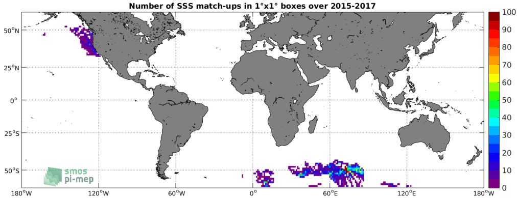
Figure 4: Number of SSS match-ups between Sea mammals SSS and the SMAP-L3-RSS-V3-8DAY-RUNNING-70KM SSS product for the SMOS coastal zone (1800km) 60N-60S Pi-MEP region over 1°x1° boxes and for the full satellite product period.
