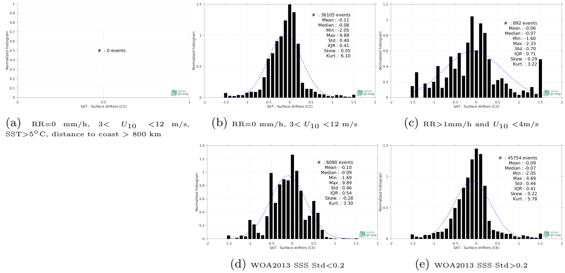
Figure 12: Normalized histogram of \Delta SSS (SMAP-L3-RSS-V3-8DAY-RUNNING-70KM - Surface drifters) for 5 different subdatasets corresponding to: RR=0 mm/h, 3 < U_{10} < 12 m/s, SST>5°C, distance to coast > 800 km (a), RR=0 mm/h, 3 < U_{10} < 12 m/s (b), RR>1mm/h and U_{10} < 4 m/s (c), WOA2013 SSS Std<0.2 (d), WOA2013 SSS Std>0.2 (e).
