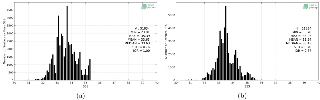
Figure 2: Histograms of SSS from Surface drifters (a) and SMAP-L3-RSS-V3-8DAY-RUNNING-70KM (b) considering all match-up pairs per bins of 0.1 over the SMOS coastal zone ( \approx 800\text{km} ) 60N-60S Pi-MEP region and for the full satellite product period.
