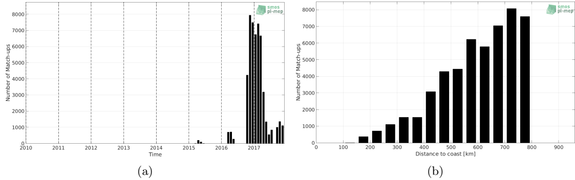
Figure 1: Number of match-ups between Surface drifters and SMAP-L3-RSS-V3-8DAY-RUNNING-70KM SSS as a function of time (a) and as function of the distance to coast (b) over the SMOS coastal zone ( \approx 800\text{km} ) 60N-60S Pi-MEP region and for the full satellite product period.
