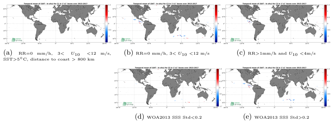
Figure 11: Temporal mean gridded over spatial boxes of size 1^\circ \times 1^\circ of \Delta SSS (SMAP-L3-RSS-V3-8DAY-RUNNING-70KM - Surface drifters) for 5 different subdatasets corresponding to:RR=0 mm/h, 3 < U_{10} < 12 m/s, SST >5^\circ C, distance to coast > 800 km (a), RR=0 mm/h, 3 < U_{10} < 12 m/s (b), RR >1 mm/h and U_{10} < 4 m/s (c), WOA2013 SSS Std <0.2 (d), WOA2013 SSS Std >0.2 (e).
