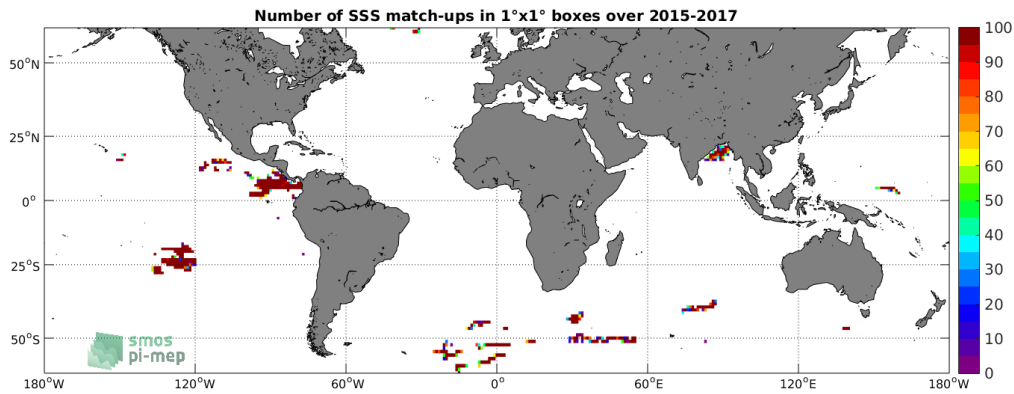
Figure 3: Number of SSS match-ups between Surface drifters SSS and the SMAP-L3-RSS-V3-8DAY-RUNNING-70KM SSS product for the SMOS coastal zone ( \geq 800\text{km} ) 60N-60S Pi-MEP region over 1^\circ \times 1^\circ boxes and for the full satellite product period.
