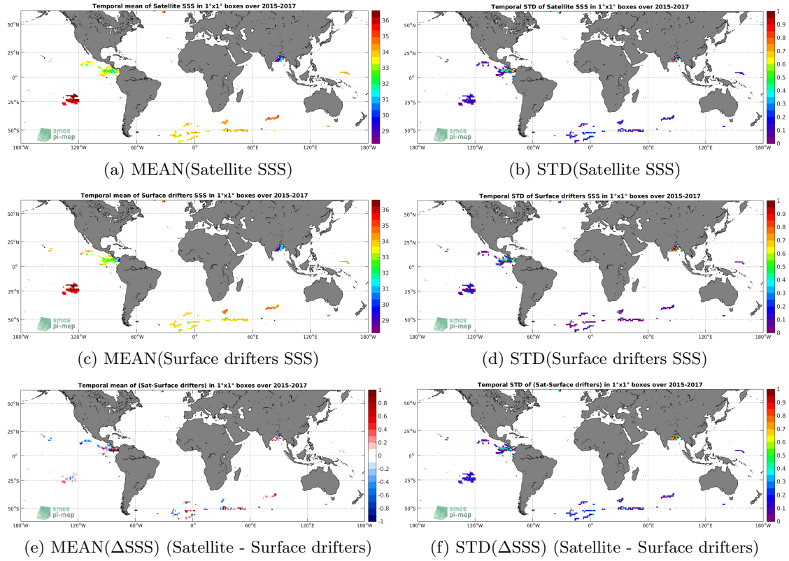
Figure 5: Temporal mean (left) and STD (right) of SSS from SMAP-L3-RSS-V3-8DAY-RUNNING-70KM (top), Surface drifters (middle), and of \Delta SSS (Satellite - Surface drifters). Only match-up pairs are used to generate these maps.
