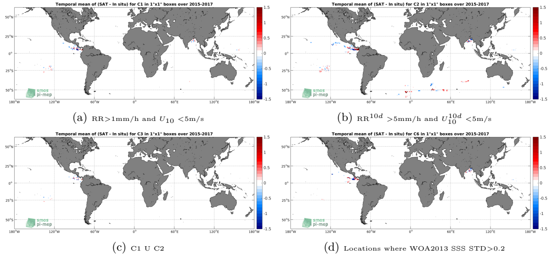
Figure 11: Temporal mean gridded over spatial boxes of size 1^\circ \times 1^\circ of \Delta SSS (SMAP-L3-RSS-V3-8DAY-RUNNING-70KM - Surface drifters) for 4 different subdatasets corresponding to: RR > 1\text{mm/h} and U_{10} < 5\text{m/s} (a), RR^{10d} > 5\text{mm/h} and U_{10}^{10d} < 5\text{m/s} (b), C1 U C2 (c), Locations where WOA2013 SSS STD > 0.2 (d).
