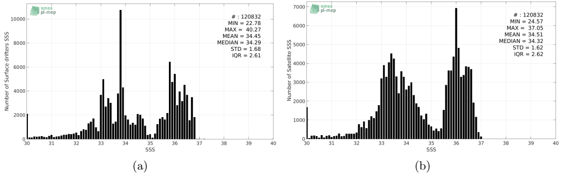
Figure 2: Histograms of SSS from Surface drifters (a) and SMAP-L3-RSS-V3-8DAY-RUNNING-70KM (b) considering all match-up pairs per bins of 0.1 over the SMOS coastal zone ( \geq 800\text{km} ) 60N-60S Pi-MEP region and for the full satellite product period.
