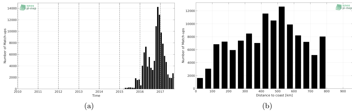
Figure 1: Number of match-ups between Surface drifters and SMAP-L3-RSS-V3-8DAY-RUNNING-70KM SSS as a function of time (a) and as function of the distance to coast (b) over the SMOS coastal zone ( \pm 800 km) 60N-60S Pi-MEP region and for the full satellite product period.
