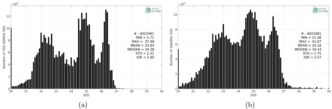
Figure 2: Histograms of SSS from TSG-SAMOS (a) and SMAP-L3-RSS-V3-8DAY-RUNNING-40KM (b) considering all match-up pairs per bins of 0.1 over the SMOS coastal zone ( \approx 800 km) 60N-60S Pi-MEP region and for the full satellite product period.
