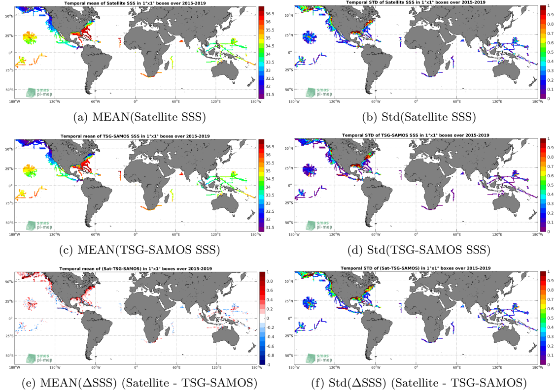
Figure 6: Temporal mean (left) and Std (right) of SSS from SMAP-L3-RSS-V3-8DAY-RUNNING-40KM (top), TSG-SAMOS (middle), and of \Delta SSS (Satellite - TSG-SAMOS). Only match-up pairs are used to generate these maps.
