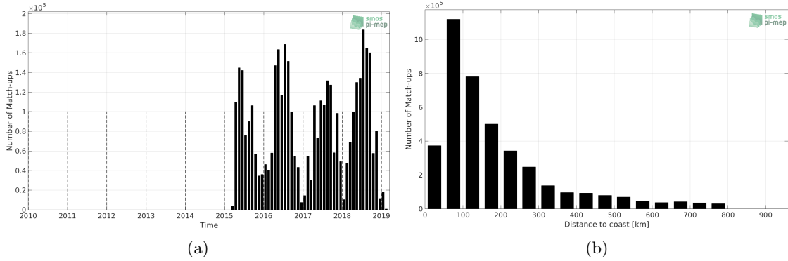
Figure 1: Number of match-ups between TSG-SAMOS and SMAP-L3-RSS-V3-8DAY-RUNNING-40KM SSS as a function of time (a) and as function of the distance to coast (b) over the SMOS coastal zone ( \approx 800 km) 60N-60S Pi-MEP region and for the full satellite product period.
