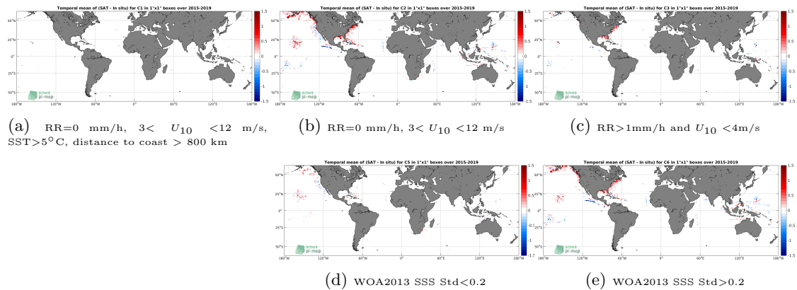
Figure 12: Temporal mean gridded over spatial boxes of size 1^\circ \times 1^\circ of \Delta SSS (SMAP-L3-RSS-V3-8DAY-RUNNING-40KM - TSG-SAMOS) for 5 different subdatasets corresponding to:RR=0 mm/h, 3 < U_{10} < 12 m/s, SST >5^\circ\text{C} , distance to coast > 800 km (a), RR=0 mm/h, 3 < U_{10} < 12 m/s (b), RR >1 mm/h and U_{10} < 4 m/s (c), WOA2013 SSS Std <0.2 (d), WOA2013 SSS Std >0.2 (e).
