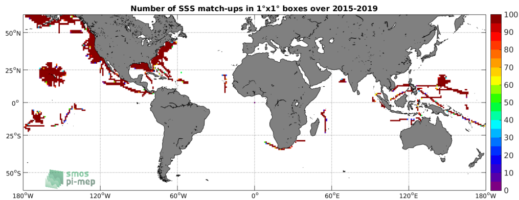
Figure 4: Number of SSS match-ups between TSG-SAMOS SSS and the SMAP-L3-RSS-V3-8DAY-RUNNING-40KM SSS product for the SMOS coastal zone ( \pm 800\text{km} ) 60N-60S Pi-MEP region over 1^\circ \times 1^\circ boxes and for the full satellite product period.
