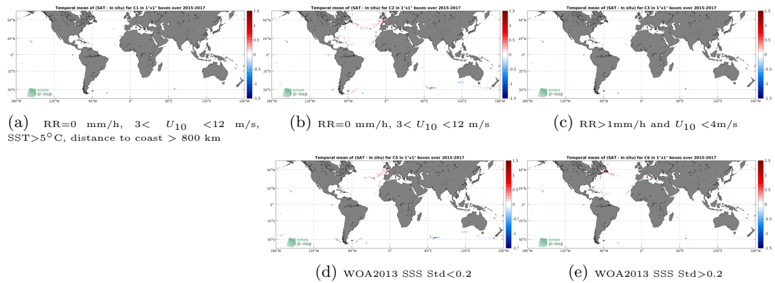
Figure 12: Temporal mean gridded over spatial boxes of size 1^\circ \times 1^\circ of \Delta SSS (SMAP-L3-RSS-V3-8DAY-RUNNING-40KM - TSG-GOSUD-Sailing-ship) for 5 different subdatasets corresponding to:RR=0 mm/h, 3 < U_{10} < 12 m/s, SST > 5^\circ\text{C} , distance to coast > 800 km (a), RR=0 mm/h, 3 < U_{10} < 12 m/s (b), RR > 1 mm/h and U_{10} < 4 m/s (c), WOA2013 SSS Std < 0.2 (d), WOA2013 SSS Std > 0.2 (e).
