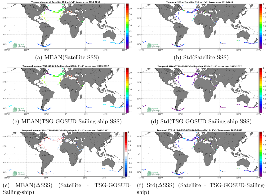
Figure 6: Temporal mean (left) and Std (right) of SSS from SMAP-L3-RSS-V3-8DAY-RUNNING-40KM (top), TSG-GOSUD-Sailing-ship (middle), and of \Delta SSS (Satellite - TSG-GOSUD-Sailing-ship). Only match-up pairs are used to generate these maps.
