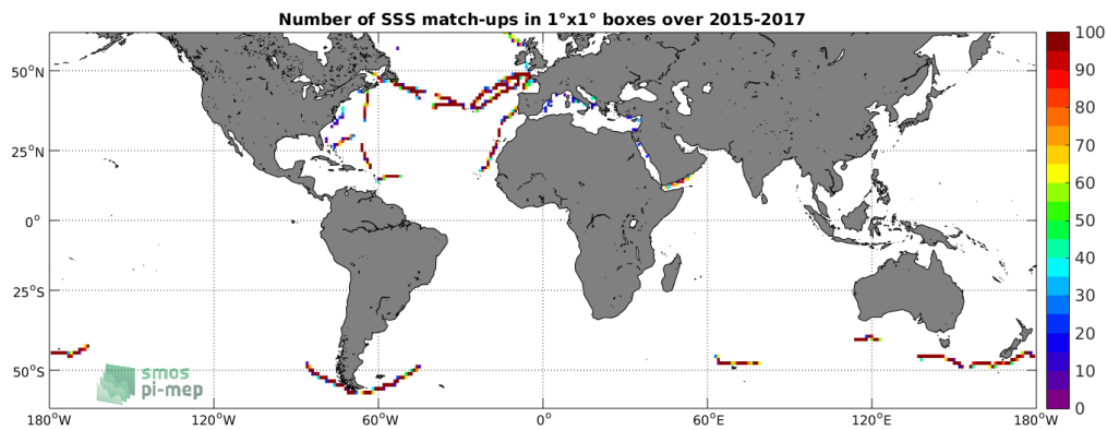
Figure 4: Number of SSS match-ups between TSG-GOSUD-Sailing-ship SSS and the SMAP-L3-RSS-V3-8DAY-RUNNING-40KM SSS product for the SMOS coastal zone ( \approx 800\text{km} ) 60N-60S Pi-MEP region over 1^\circ \times 1^\circ boxes and for the full satellite product period.
