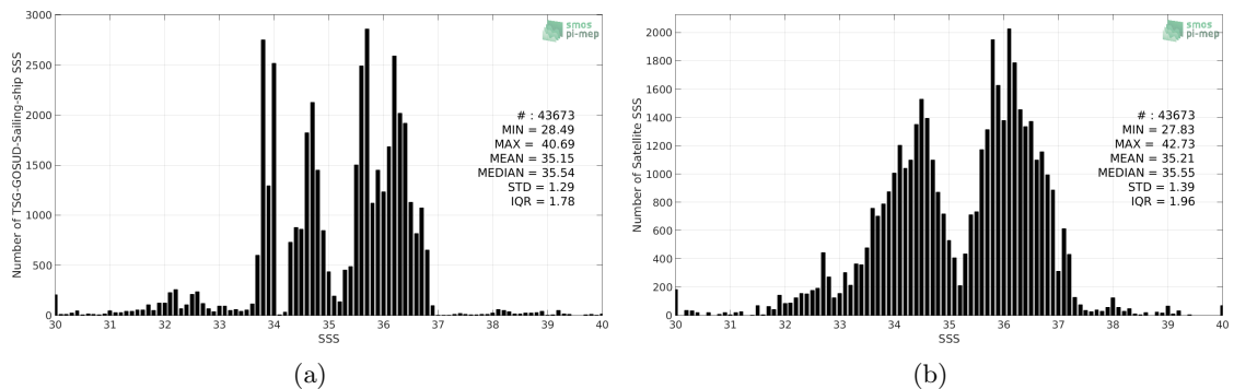
Figure 2: Histograms of SSS from TSG-GOSUD-Sailing-ship (a) and SMAP-L3-RSS-V3-8DAY-RUNNING-40KM (b) considering all match-up pairs per bins of 0.1 over the SMOS coastal zone ( \approx 800\text{km} ) 60N-60S Pi-MEP region and for the full satellite product period.
