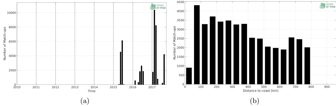
Figure 1: Number of match-ups between TSG-GOSUD-Sailing-ship and SMAP-L3-RSS-V3-8DAY-RUNNING-40KM SSS as a function of time (a) and as function of the distance to coast (b) over the SMOS coastal zone ( \approx 800\text{km} ) 60N-60S Pi-MEP region and for the full satellite product period.
