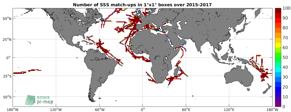
Figure 4: Number of SSS match-ups between TSG-GOSUD-Research-vessel SSS and the SMAP-L3-RSS-V3-8DAY-RUNNING-40KM SSS product for the SMOS coastal zone ( \pm 800\text{km} ) 60N-60S Pi-MEP region over 1^\circ \times 1^\circ boxes and for the full satellite product period.
