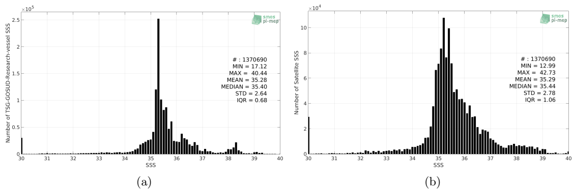
Figure 2: Histograms of SSS from TSG-GOSUD-Research-vessel (a) and SMAP-L3-RSS-V3-8DAY-RUNNING-40KM (b) considering all match-up pairs per bins of 0.1 over the SMOS coastal zone ( \approx 800 km) 60N-60S Pi-MEP region and for the full satellite product period.
