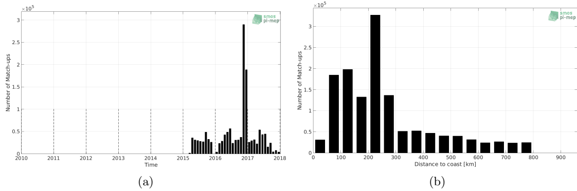
Figure 1: Number of match-ups between TSG-GOSUD-Research-vessel and SMAP-L3-RSS-V3-8DAY-RUNNING-40KM SSS as a function of time (a) and as function of the distance to coast (b) over the SMOS coastal zone ( \approx 800 km) 60N-60S Pi-MEP region and for the full satellite product period.
