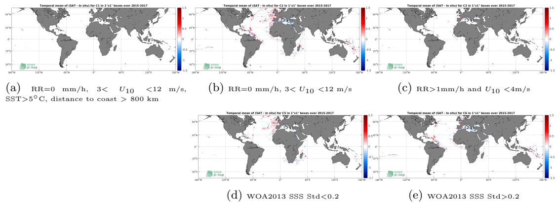
Figure 12: Temporal mean gridded over spatial boxes of size 1^\circ \times 1^\circ of \Delta SSS (SMAP-L3-RSS-V3-8DAY-RUNNING-40KM - TSG-GOSUD-Research-vessel) for 5 different subdatasets corresponding to:RR=0 mm/h, 3 < U_{10} < 12 m/s, SST >5^\circ C, distance to coast > 800 km (a), RR=0 mm/h, 3 < U_{10} < 12 m/s (b), RR >1 mm/h and U_{10} < 4 m/s (c), WOA2013 SSS Std <0.2 (d), WOA2013 SSS Std >0.2 (e).
