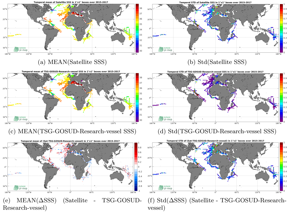
Figure 6: Temporal mean (left) and Std (right) of SSS from SMAP-L3-RSS-V3-8DAY-RUNNING-40KM (top), TSG-GOSUD-Research-vessel (middle), and of \Delta SSS (Satellite - TSG-GOSUD-Research-vessel). Only match-up pairs are used to generate these maps.
