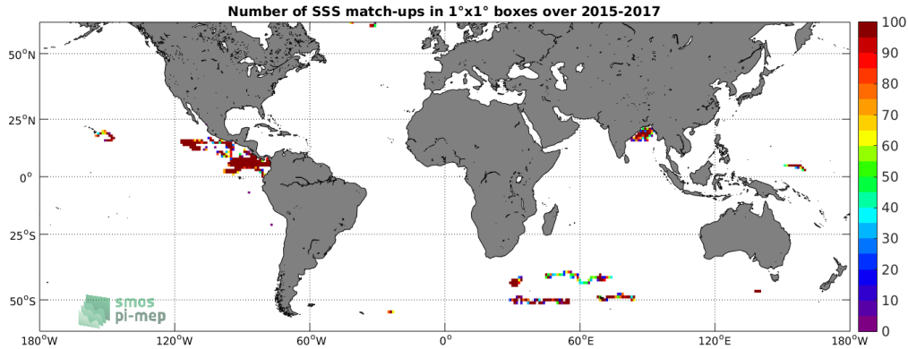
Figure 3: Number of SSS match-ups between Surface drifters SSS and the SMAP-L3-RSS-V3-8DAY-RUNNING-40KM SSS product for the SMOS coastal zone ( \geq 800\text{km} ) 60N-60S Pi-MEP region over 1^\circ \times 1^\circ boxes and for the full satellite product period.
