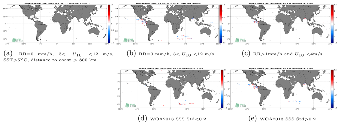
Figure 11: Temporal mean gridded over spatial boxes of size 1^\circ \times 1^\circ of \Delta SSS (SMAP-L3-RSS-V3-8DAY-RUNNING-40KM - Surface drifters) for 5 different subdatasets corresponding to:RR=0 mm/h, 3 < U_{10} < 12 m/s, SST >5^\circ C, distance to coast > 800 km (a), RR=0 mm/h, 3 < U_{10} < 12 m/s (b), RR >1 mm/h and U_{10} < 4 m/s (c), WOA2013 SSS Std <0.2 (d), WOA2013 SSS Std >0.2 (e).
