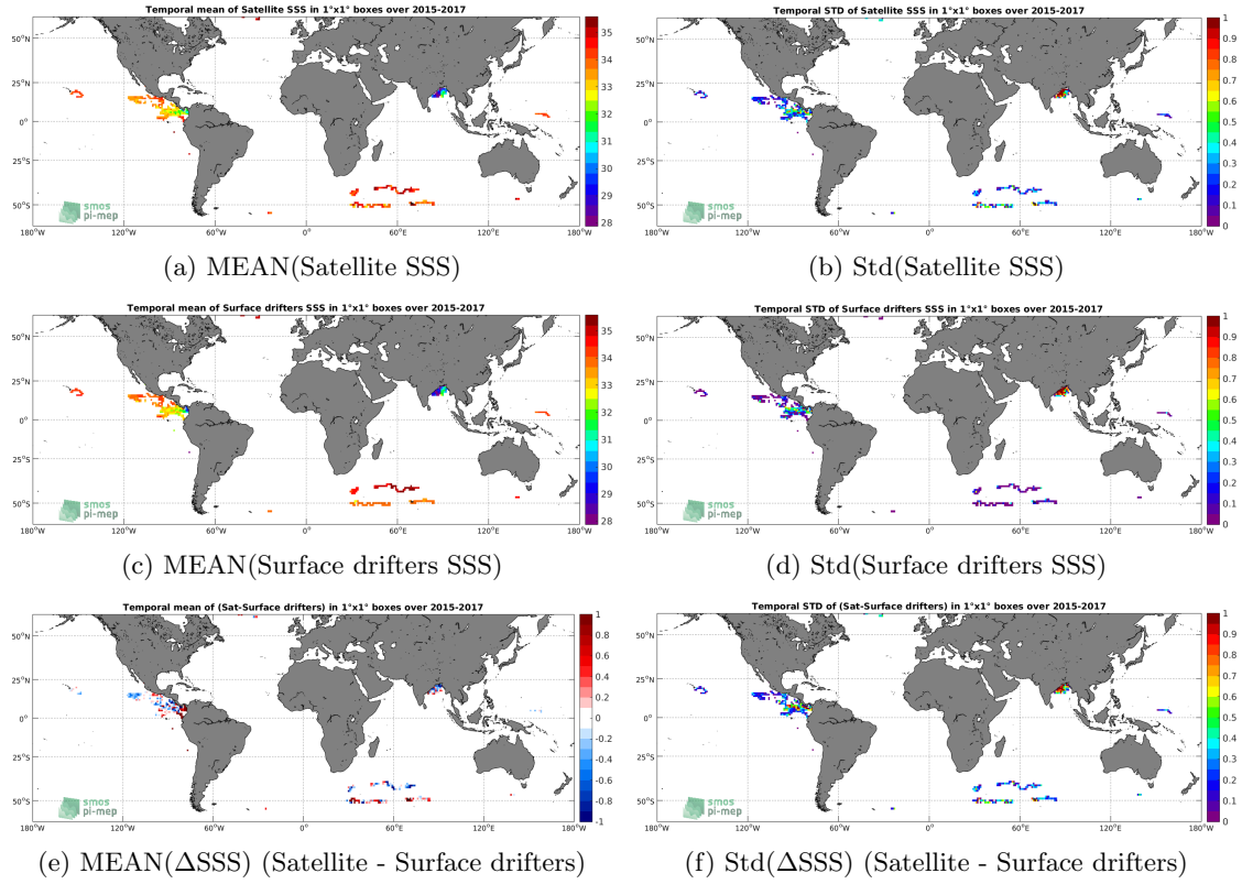
Figure 5: Temporal mean (left) and Std (right) of SSS from SMAP-L3-RSS-V3-8DAY-RUNNING-40KM (top), Surface drifters (middle), and of \Delta SSS (Satellite - Surface drifters). Only match-up pairs are used to generate these maps.
