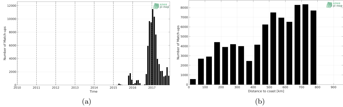
Figure 1: Number of match-ups between Surface drifters and SMAP-L3-RSS-V3-8DAY-RUNNING-40KM SSS as a function of time (a) and as function of the distance to coast (b) over the SMOS coastal zone ( \approx 800\text{km} ) 60N-60S Pi-MEP region and for the full satellite product period.
