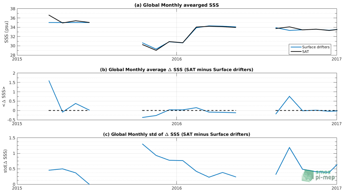
Figure 6: Time series of the monthly averaged mean SSS (top), mean \Delta \text{SSS} (Satellite - Surface drifters) and Std of \Delta \text{SSS} (Satellite - Surface drifters) over the SMOS coastal zone ( \geq 800\text{km} ) 60N-60S Pi-MEP region considering all match-ups collected by the Pi-MEP platform.
