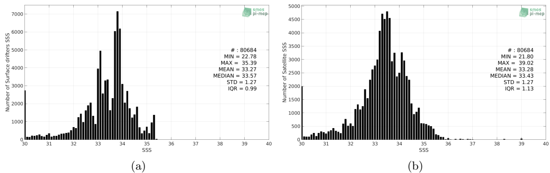
Figure 2: Histograms of SSS from Surface drifters (a) and SMAP-L3-RSS-V3-8DAY-RUNNING-40KM (b) considering all match-up pairs per bins of 0.1 over the SMOS coastal zone ( \approx 800\text{km} ) 60N-60S Pi-MEP region and for the full satellite product period.
