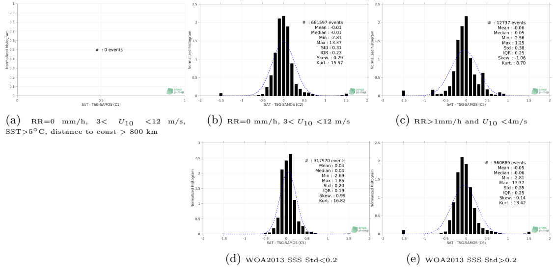
Figure 13: Normalized histogram of \Delta SSS (SMAP-L3-RSS-V3-MONTHLY-70KM - TSG-SAMOS) for 5 different subdatasets corresponding to: RR=0 mm/h, 3 < U_{10} < 12 m/s, SST > 5°C, distance to coast > 800 km (a), RR=0 mm/h, 3 < U_{10} < 12 m/s (b), RR > 1mm/h and U_{10} < 4 m/s (c), WOA2013 SSS Std < 0.2 (d), WOA2013 SSS Std > 0.2 (e).
