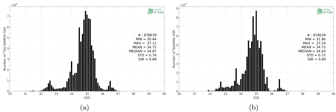
Figure 2: Histograms of SSS from TSG-SAMOS (a) and SMAP-L3-RSS-V3-MONTHLY-70KM (b) considering all match-up pairs per bins of 0.1 over the SMOS coastal zone ( \geq 800 km) 60N-60S Pi-MEP region and for the full satellite product period.
