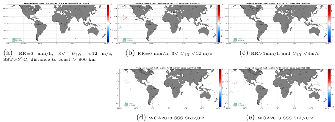
Figure 12: Temporal mean gridded over spatial boxes of size 1^\circ \times 1^\circ of \Delta SSS (SMAP-L3-RSS-V3-MONTHLY-70KM - TSG-SAMOS) for 5 different subdatasets corresponding to:RR=0 mm/h, 3 < U_{10} < 12 m/s, SST >5^\circ\text{C} , distance to coast > 800 km (a), RR=0 mm/h, 3 < U_{10} < 12 m/s (b), RR >1 mm/h and U_{10} < 4 m/s (c), WOA2013 SSS Std <0.2 (d), WOA2013 SSS Std >0.2 (e).
