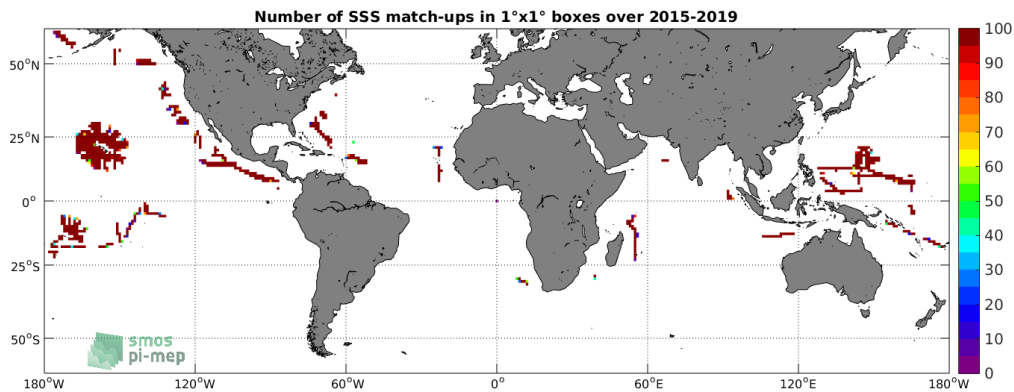
Figure 4: Number of SSS match-ups between TSG-SAMOS SSS and the SMAP-L3-RSS-V3-MONTHLY-70KM SSS product for the SMOS coastal zone ( \approx 800\text{km} ) 60N-60S Pi-MEP region over 1^\circ \times 1^\circ boxes and for the full satellite product period.
