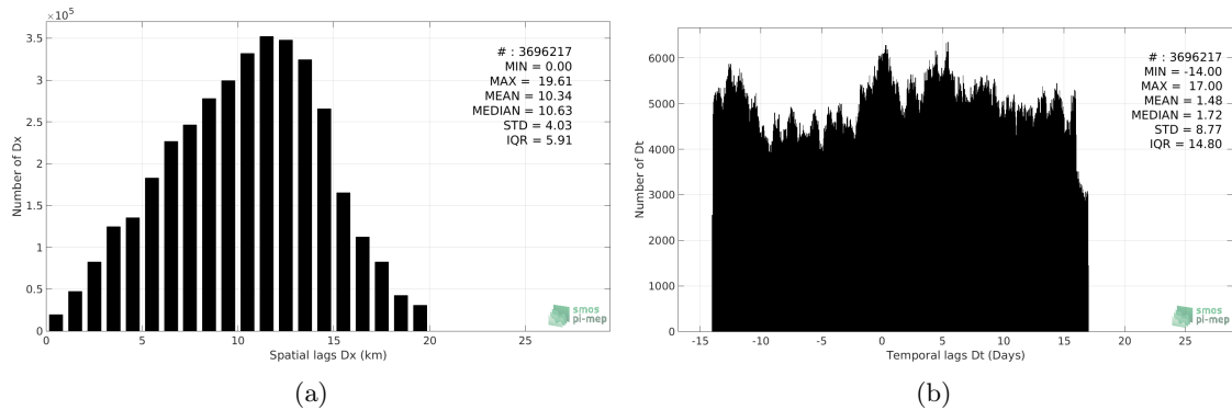
Figure 5: Histograms of the spatial (a) and temporal (b) lags between the time of the TSG-SAMOS measurements and the date of the corresponding SMAP-L3-RSS-V3-MONTHLY-70KM SSS product.
