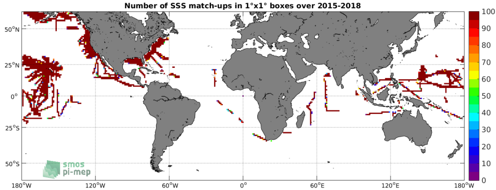
Figure 4: Number of SSS match-ups between TSG-SAMOS SSS and the SMAP-L3-RSS-V3-MONTHLY-70KM SSS product for the SMOS coastal zone ( \approx 800\text{km} ) 60\text{N} - 60\text{S} Pi-MEP region over 1^\circ \times 1^\circ boxes and for the full satellite product period.
