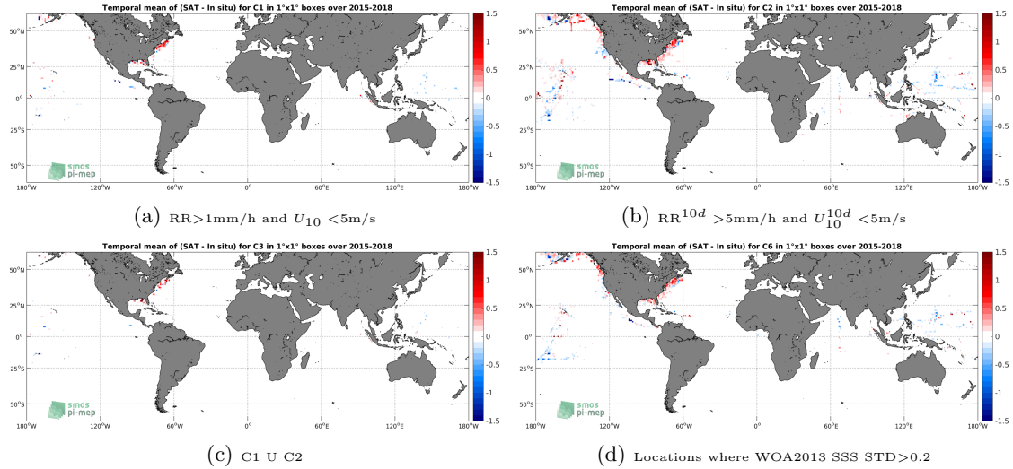
Figure 12: Temporal mean gridded over spatial boxes of size 1^\circ \times 1^\circ of \Delta SSS (SMAP-L3-RSS-V3-MONTHLY-70KM - TSG-SAMOS) for 4 different subdatasets corresponding to: RR > 1\text{mm/h} and U_{10} < 5\text{m/s} (a), RR^{10d} > 5\text{mm/h} and U_{10}^{10d} < 5\text{m/s} (b), C1 U C2 (c), Locations where WOA2013 SSS STD > 0.2 (d).
