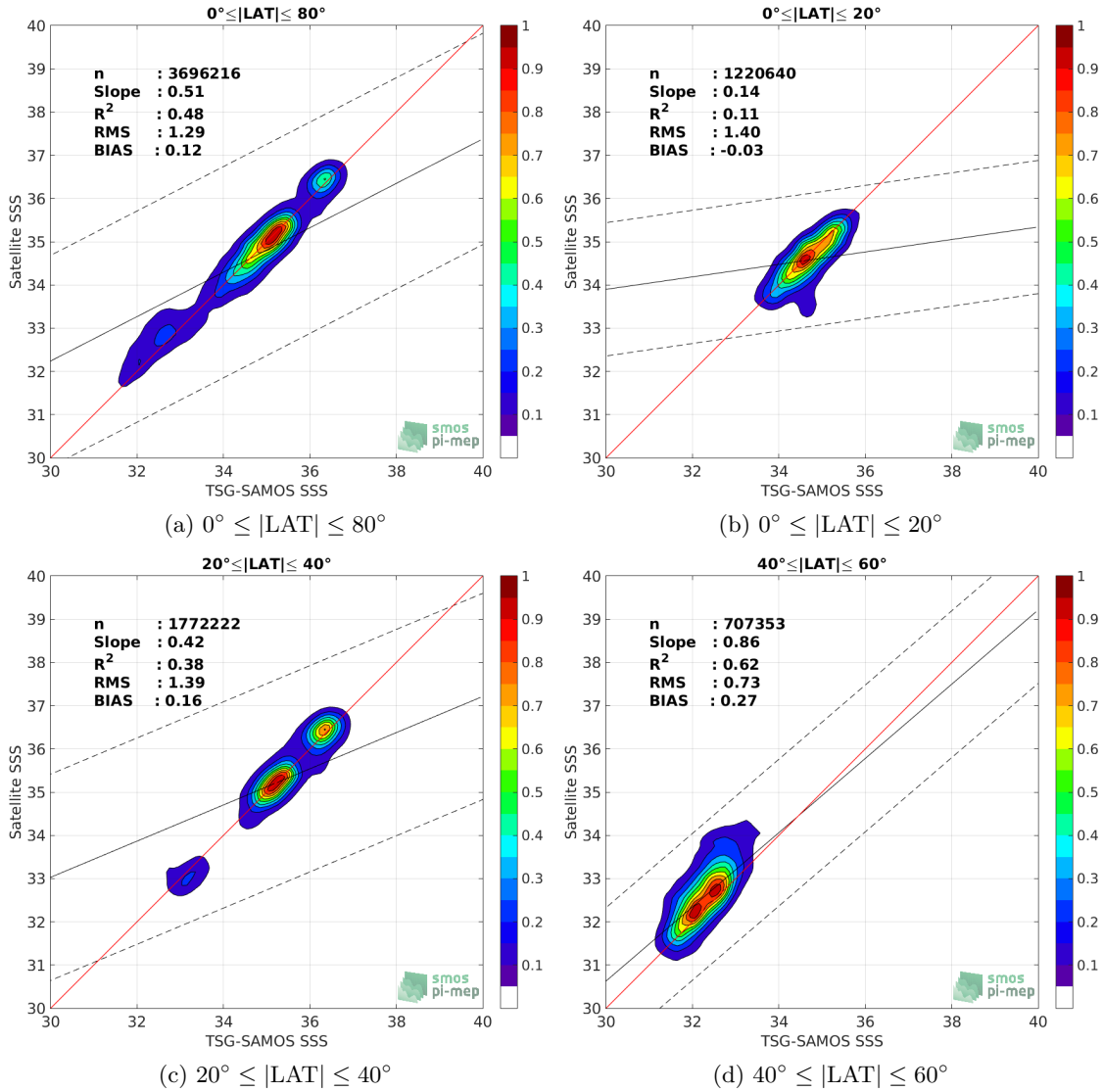
Figure 9: Contour maps of the concentration of SMAP-L3-RSS-V3-MONTHLY-70KM SSS (y-axis) versus TSG-SAMOS SSS (x-axis) at match-up pairs for different latitude bands. For each plot, the red line shows x=y . The black thin and dashed lines indicate a linear fit through the data cloud and the \pm 95\% confidence levels, respectively. The number match-up pairs n , the slope and R^2 coefficient of the linear fit, the root mean square (RMS) and the mean bias between satellite and in situ data are indicated for each latitude band in each plots.
