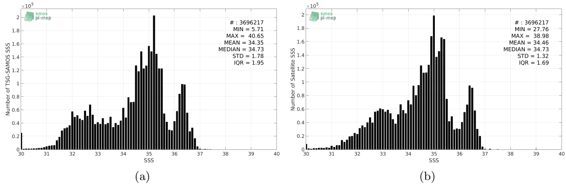
Figure 2: Histograms of SSS from TSG-SAMOS (a) and SMAP-L3-RSS-V3-MONTHLY-70KM (b) considering all match-up pairs per bins of 0.1 over the SMOS coastal zone ( \approx 800\text{km} ) 60N-60S Pi-MEP region and for the full satellite product period.
