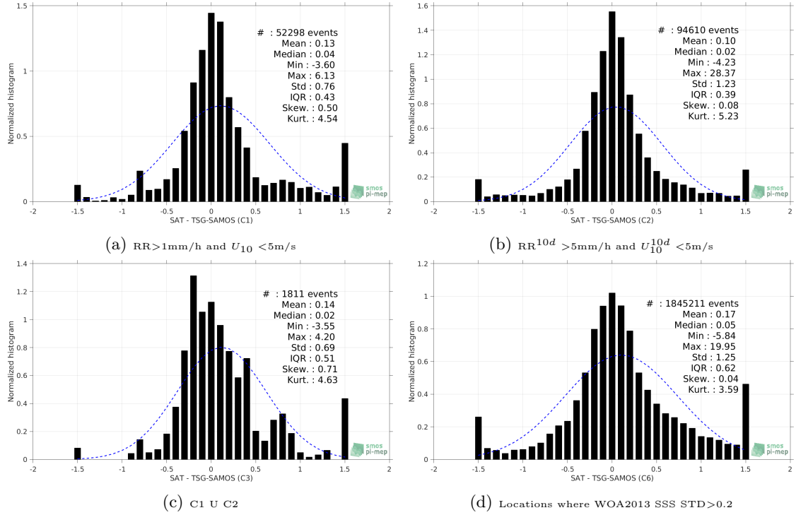
Figure 13: Normalized histogram of \Delta\text{SSS} (SMAP-L3-RSS-V3-MONTHLY-70KM - TSG-SAMOS) for 6 different subdatasets corresponding to: RR > 1\text{mm/h} and U_{10} < 5\text{m/s} (a), RR^{10d} > 5\text{mm/h} and U_{10}^{10d} < 5\text{m/s} (b), C1 U C2 (c), Locations where WOA2013 SSS STD > 0.2 (d).
