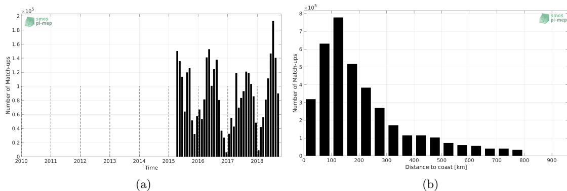
Figure 1: Number of match-ups between TSG-SAMOS and SMAP-L3-RSS-V3-MONTHLY-70KM SSS as a function of time (a) and as function of the distance to coast (b) over the SMOS coastal zone ( \approx 800 km) 60N-60S Pi-MEP region and for the full satellite product period.
