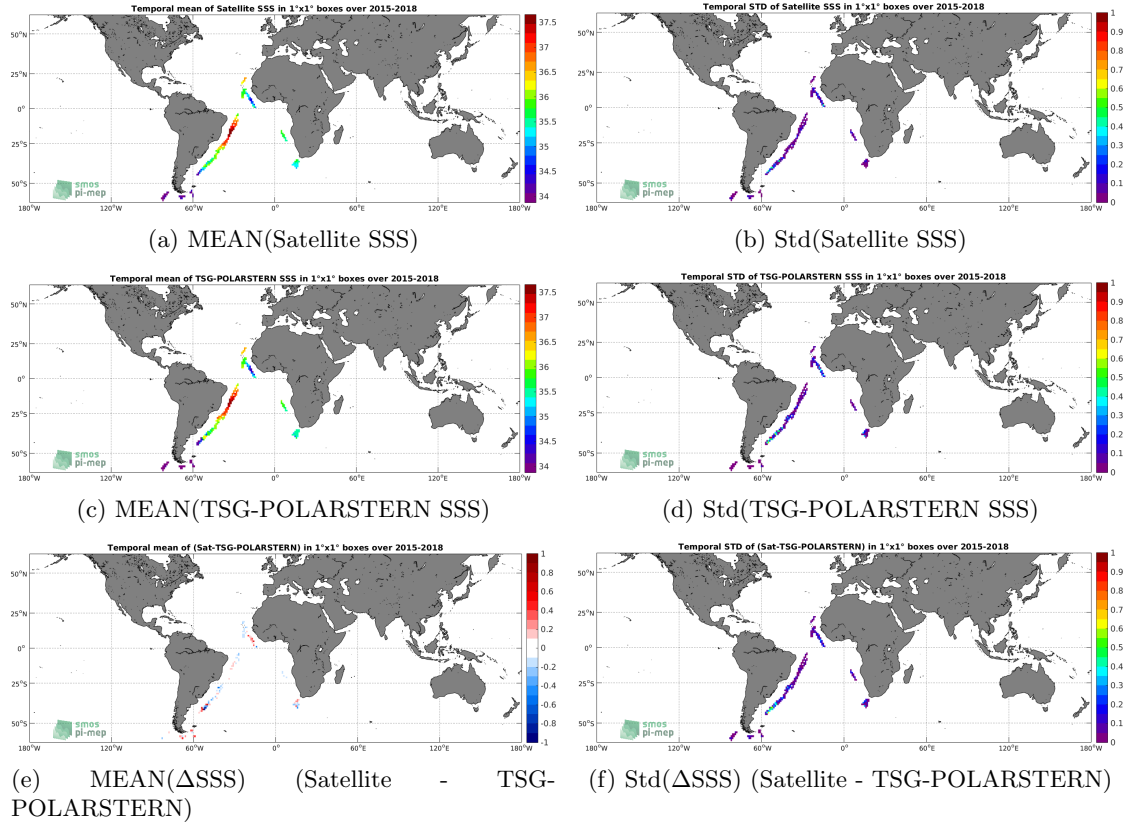
Figure 6: Temporal mean (left) and Std (right) of SSS from SMAP-L3-RSS-V3-MONTHLY-70KM (top), TSG-POLARSTERN (middle), and of \Delta SSS (Satellite - TSG-POLARSTERN). Only match-up pairs are used to generate these maps.
