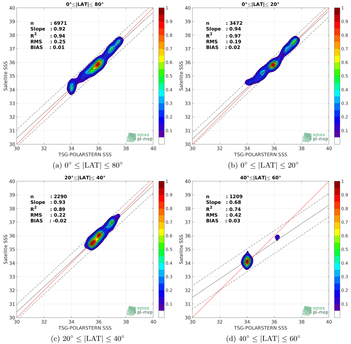
Figure 9: Contour maps of the concentration of SMAP-L3-RSS-V3-MONTHLY-70KM SSS (y-axis) versus TSG-POLARSTERN SSS (x-axis) at match-up pairs for different latitude bands. For each plot, the red line shows x=y . The black thin and dashed lines indicate a linear fit through the data cloud and the \pm 95\% confidence levels, respectively. The number match-up pairs n , the slope and R^2 coefficient of the linear fit, the root mean square (RMS) and the mean bias between satellite and in situ data are indicated for each latitude band in each plots.
