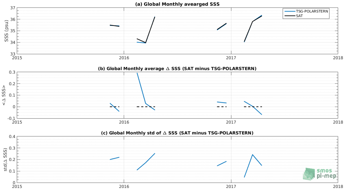
Figure 7: Time series of the monthly averaged mean SSS (top), mean \Delta SSS (Satellite - TSG-POLARSTERN) and Std of \Delta SSS (Satellite - TSG-POLARSTERN) over the SMOS coastal zone ( \approx 800 km) 60N-60S Pi-MEP region considering all match-ups collected by the Pi-MEP platform.
