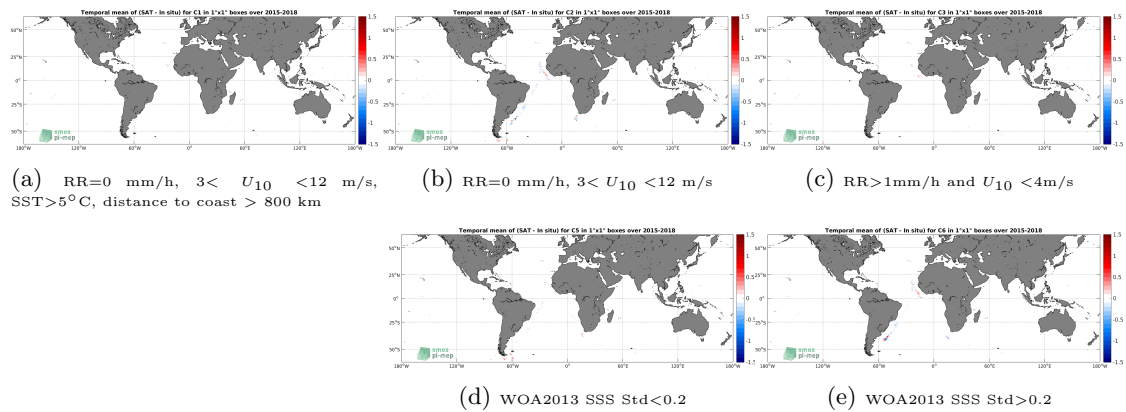
Figure 12: Temporal mean gridded over spatial boxes of size 1^\circ \times 1^\circ of \Delta SSS (SMAP-L3-RSS-V3-MONTHLY-70KM - TSG-POLARSTERN) for 5 different subdatasets corresponding to:RR=0 mm/h, 3 < U_{10} < 12 m/s, SST >5^\circ C, distance to coast > 800 km (a), RR=0 mm/h, 3 < U_{10} < 12 m/s (b), RR >1 mm/h and U_{10} < 4 m/s (c), WOA2013 SSS Std <0.2 (d), WOA2013 SSS Std >0.2 (e).
