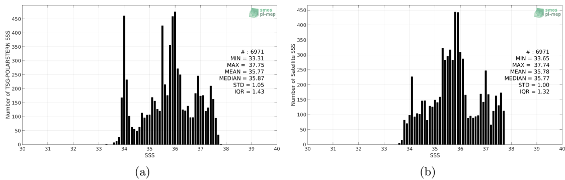
Figure 2: Histograms of SSS from TSG-POLARSTERN (a) and SMAP-L3-RSS-V3-MONTHLY-70KM (b) considering all match-up pairs per bins of 0.1 over the SMOS coastal zone ( \approx 800 km) 60N-60S Pi-MEP region and for the full satellite product period.
