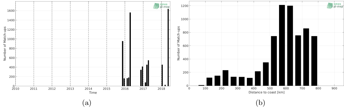
Figure 1: Number of match-ups between TSG-POLARSTERN and SMAP-L3-RSS-V3-MONTHLY-70KM SSS as a function of time (a) and as function of the distance to coast (b) over the SMOS coastal zone ( \approx 800 km) 60N-60S Pi-MEP region and for the full satellite product period.
