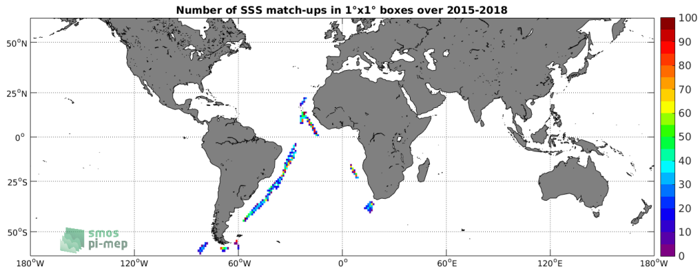
Figure 4: Number of SSS match-ups between TSG-POLARSTERN SSS and the SMAP-L3-RSS-V3-MONTHLY-70KM SSS product for the SMOS coastal zone ( \approx 800\text{km} ) 60N-60S Pi-MEP region over 1^\circ \times 1^\circ boxes and for the full satellite product period.
