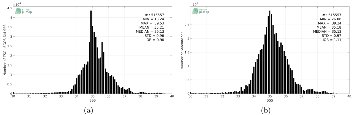
Figure 2: Histograms of SSS from TSG-LEGOS-DM (a) and SMAP-L3-RSS-V3-MONTHLY-70KM (b) considering all match-up pairs per bins of 0.1 over the SMOS coastal zone ( \geq 800\text{km} ) 60N-60S Pi-MEP region and for the full satellite product period.
