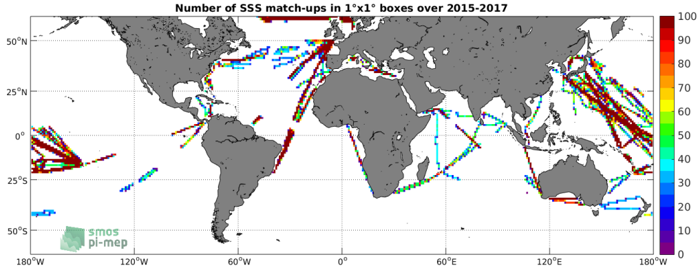
Figure 4: Number of SSS match-ups between TSG-LEGOS-DM SSS and the SMAP-L3-RSS-V3-MONTHLY-70KM SSS product for the SMOS coastal zone ( \approx 800\text{km} ) 60N-60S Pi-MEP region over 1^\circ \times 1^\circ boxes and for the full satellite product period.
