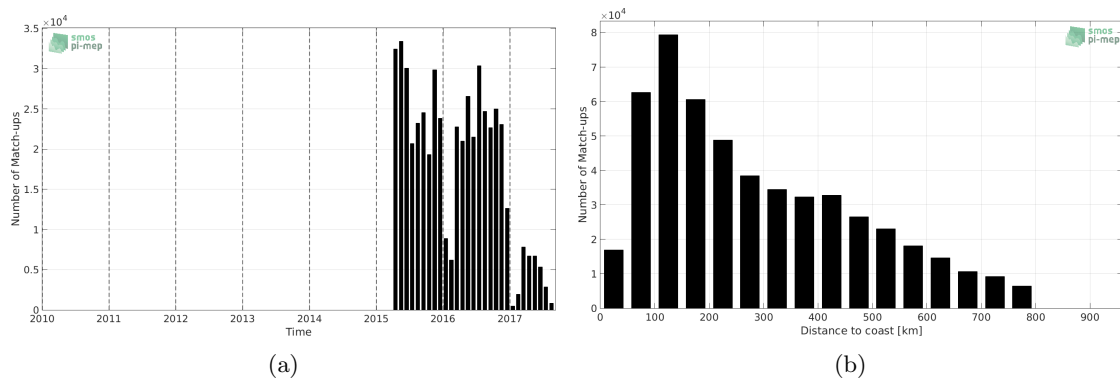
Figure 1: Number of match-ups between TSG-LEGOS-DM and SMAP-L3-RSS-V3-MONTHLY-70KM SSS as a function of time (a) and as function of the distance to coast (b) over the SMOS coastal zone ( \pm 800 km) 60N-60S Pi-MEP region and for the full satellite product period.
