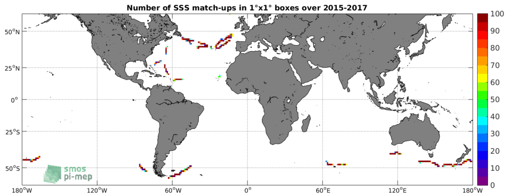
Figure 4: Number of SSS match-ups between TSG-GOSUD-Sailing-ship SSS and the SMAP-L3-RSS-V3-MONTHLY-70KM SSS product for the SMOS coastal zone ( \pm 800\text{km} ) 60N-60S Pi-MEP region over 1^\circ \times 1^\circ boxes and for the full satellite product period.
