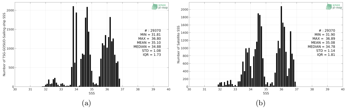
Figure 2: Histograms of SSS from TSG-GOSUD-Sailing-ship (a) and SMAP-L3-RSS-V3-MONTHLY-70KM (b) considering all match-up pairs per bins of 0.1 over the SMOS coastal zone ( \approx 800 km) 60N-60S Pi-MEP region and for the full satellite product period.
