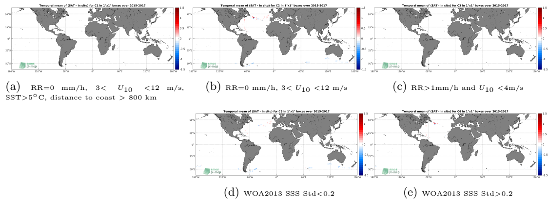
Figure 12: Temporal mean gridded over spatial boxes of size 1^\circ \times 1^\circ of \Delta SSS (SMAP-L3-RSS-V3-MONTHLY-70KM - TSG-GOSUD-Sailing-ship) for 5 different subdatasets corresponding to:RR=0 mm/h, 3 < U_{10} < 12 m/s, SST >5^\circ C, distance to coast > 800 km (a), RR=0 mm/h, 3 < U_{10} < 12 m/s (b), RR >1 mm/h and U_{10} < 4 m/s (c), WOA2013 SSS Std <0.2 (d), WOA2013 SSS Std >0.2 (e).
