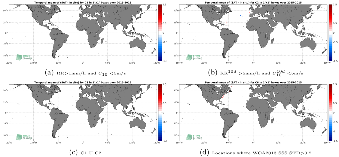
Figure 12: Temporal mean gridded over spatial boxes of size 1^\circ \times 1^\circ of \Delta SSS (SMAP-L3-RSS-V3-MONTHLY-70KM - TSG-GOSUD-Sailing-ship) for 4 different subdatasets corresponding to: RR > 1\text{mm/h} and U_{10} < 5\text{m/s} (a), RR^{10d} > 5\text{mm/h} and U_{10}^{10d} < 5\text{m/s} (b), C1 U C2 (c), Locations where WOA2013 SSS STD > 0.2 (d).
