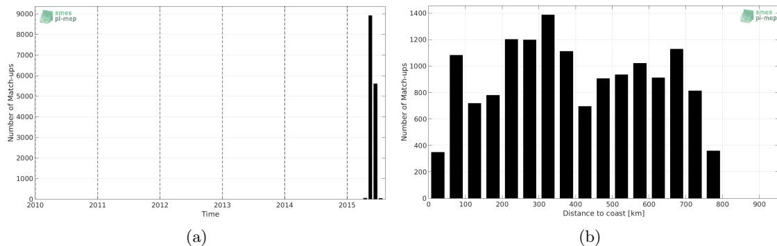
Figure 1: Number of match-ups between TSG-GOSUD-Sailing-ship and SMAP-L3-RSS-V3-MONTHLY-70KM SSS as a function of time (a) and as function of the distance to coast (b) over the SMOS coastal zone ( \approx 800 km) 60N-60S Pi-MEP region and for the full satellite product period.
