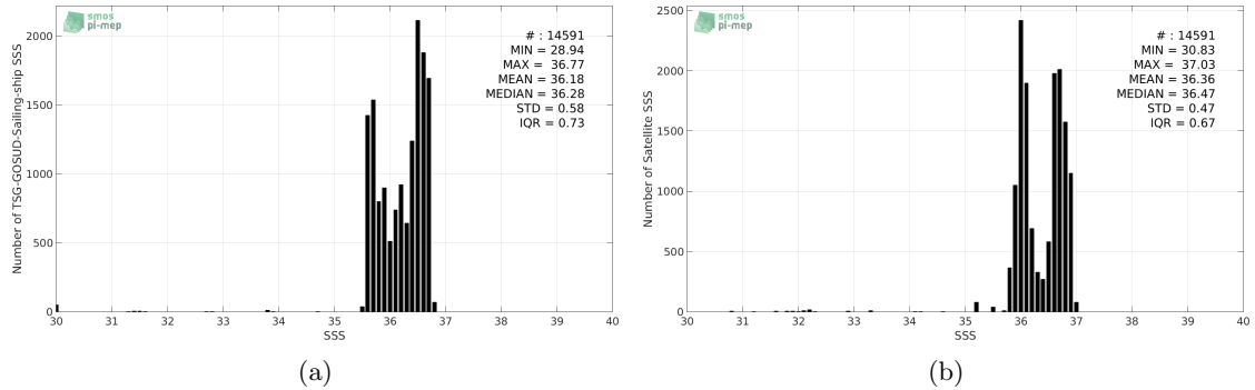
Figure 2: Histograms of SSS from TSG-GOSUD-Sailing-ship (a) and SMAP-L3-RSS-V3-MONTHLY-70KM (b) considering all match-up pairs per bins of 0.1 over the SMOS coastal zone ( \approx 800\text{km} ) 60N-60S Pi-MEP region and for the full satellite product period.
