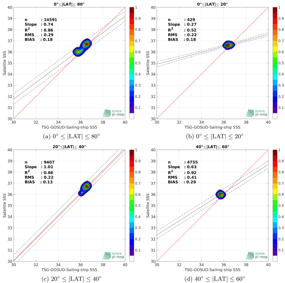
Figure 9: Contour maps of the concentration of SMAP-L3-RSS-V3-MONTHLY-70KM SSS (y-axis) versus TSG-GOSUD-Sailing-ship SSS (x-axis) at match-up pairs for different latitude bands. For each plot, the red line shows x=y . The black thin and dashed lines indicate a linear fit through the data cloud and the \pm 95\% confidence levels, respectively. The number match-up pairs n , the slope and R^2 coefficient of the linear fit, the root mean square (RMS) and the mean bias between satellite and in situ data are indicated for each latitude band in each plots.
