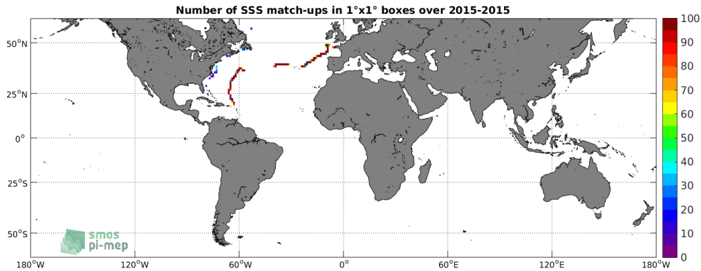
Figure 4: Number of SSS match-ups between TSG-GOSUD-Sailing-ship SSS and the SMAP-L3-RSS-V3-MONTHLY-70KM SSS product for the SMOS coastal zone ( \approx 800\text{km} ) 60N-60S Pi-MEP region over 1^\circ \times 1^\circ boxes and for the full satellite product period.
