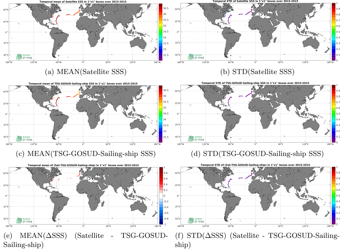
Figure 6: Temporal mean (left) and STD (right) of SSS from SMAP-L3-RSS-V3-MONTHLY-70KM (top), TSG-GOSUD-Sailing-ship (middle), and of \Delta SSS (Satellite - TSG-GOSUD-Sailing-ship). Only match-up pairs are used to generate these maps.
