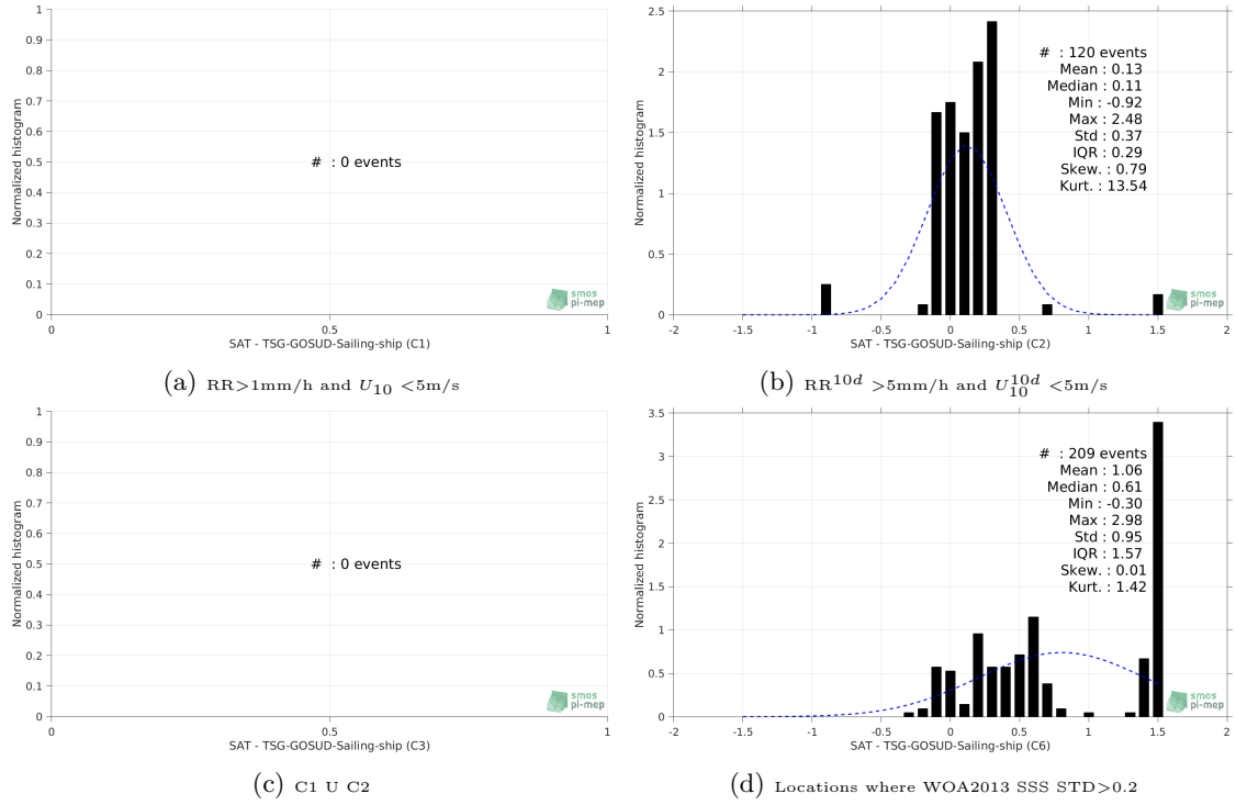
Figure 13: Normalized histogram of \Delta\text{SSS} (SMAP-L3-RSS-V3-MONTHLY-70KM - TSG-GOSUD-Sailing-ship) for 6 different subdatasets corresponding to: RR > 1\text{mm/h} and U_{10} < 5\text{m/s} (a), RR^{10d} > 5\text{mm/h} and U_{10}^{10d} < 5\text{m/s} (b), C1 \cup C2 (c), Locations where WOA2013 SSS STD > 0.2 (d).
