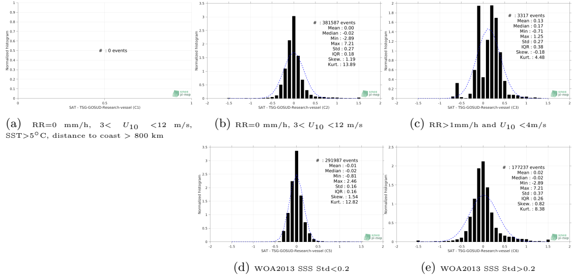
Figure 13: Normalized histogram of \Delta SSS (SMAP-L3-RSS-V3-MONTHLY-70KM - TSG-GOSUD-Research-vessel) for 5 different subdatasets corresponding to: RR=0 mm/h, 3 < U_{10} < 12 m/s, SST>5°C, distance to coast > 800 km (a), RR=0 mm/h, 3 < U_{10} < 12 m/s (b), RR>1mm/h and U_{10} < 4 m/s (c), WOA2013 SSS Std<0.2 (d), WOA2013 SSS Std>0.2 (e).
