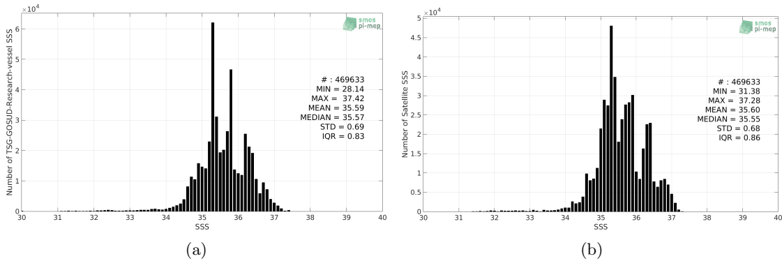
Figure 2: Histograms of SSS from TSG-GOSUD-Research-vessel (a) and SMAP-L3-RSS-V3-MONTHLY-70KM (b) considering all match-up pairs per bins of 0.1 over the SMOS coastal zone ( \geq 800 km) 60N-60S Pi-MEP region and for the full satellite product period.
