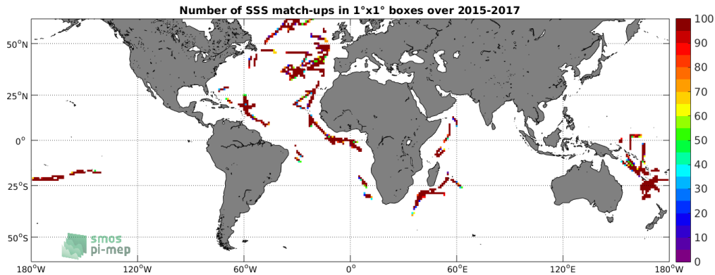
Figure 4: Number of SSS match-ups between TSG-GOSUD-Research-vessel SSS and the SMAP-L3-RSS-V3-MONTHLY-70KM SSS product for the SMOS coastal zone ( \pm 800\text{km} ) 60N-60S Pi-MEP region over 1^\circ \times 1^\circ boxes and for the full satellite product period.
