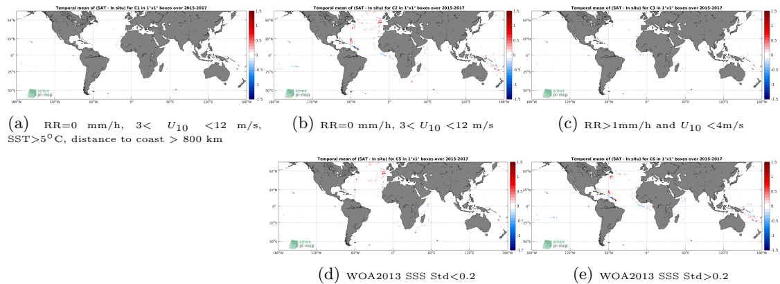
Figure 12: Temporal mean gridded over spatial boxes of size 1^\circ \times 1^\circ of \Delta SSS (SMAP-L3-RSS-V3-MONTHLY-70KM - TSG-GOSUD-Research-vessel) for 5 different subdatasets corresponding to:RR=0 mm/h, 3 < U_{10} < 12 m/s, SST >5^\circ C, distance to coast > 800 km (a), RR=0 mm/h, 3 < U_{10} < 12 m/s (b), RR >1 mm/h and U_{10} < 4 m/s (c), WOA2013 SSS Std <0.2 (d), WOA2013 SSS Std >0.2 (e).
