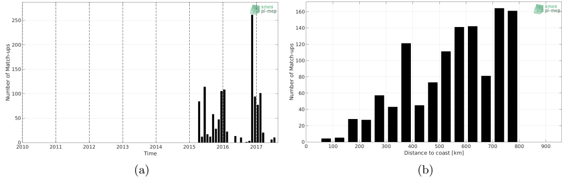
Figure 1: Number of match-ups between Sea mammals and SMAP-L3-RSS-V3-MONTHLY-70KM SSS as a function of time (a) and as function of the distance to coast (b) over the SMOS coastal zone ( \approx 800\text{km} ) 60N-60S Pi-MEP region and for the full satellite product period.
