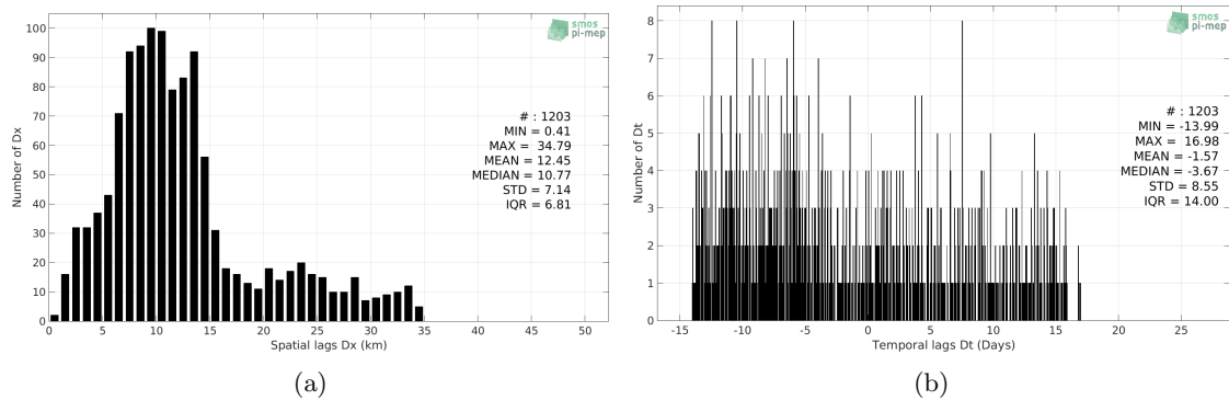
Figure 5: Histograms of the spatial (a) and temporal (b) lags between the time of the Sea mammals measurements and the date of the corresponding SMAP-L3-RSS-V3-MONTHLY-70KM SSS product.
