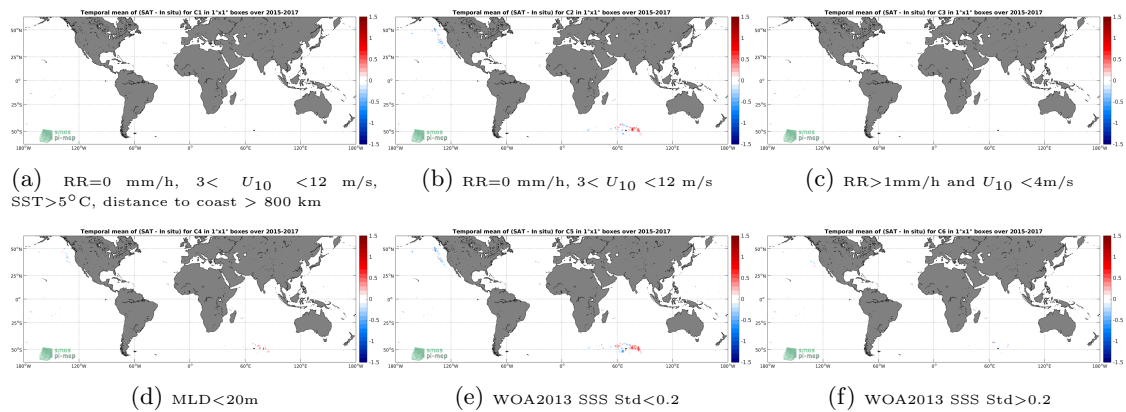
Figure 12: Temporal mean gridded over spatial boxes of size 1^\circ \times 1^\circ of \Delta SSS (SMAP-L3-RSS-V3-MONTHLY-70KM - Sea mammals) for 6 different subdatasets corresponding to:RR=0 mm/h, 3 < U_{10} < 12 m/s, SST >5^\circ C, distance to coast > 800 km (a), RR=0 mm/h, 3 < U_{10} < 12 m/s (b), RR >1 mm/h and U_{10} < 4 m/s (c),MLD <20 m (d),WOA2013 SSS Std <0.2 (e),WOA2013 SSS Std >0.2 (f).
