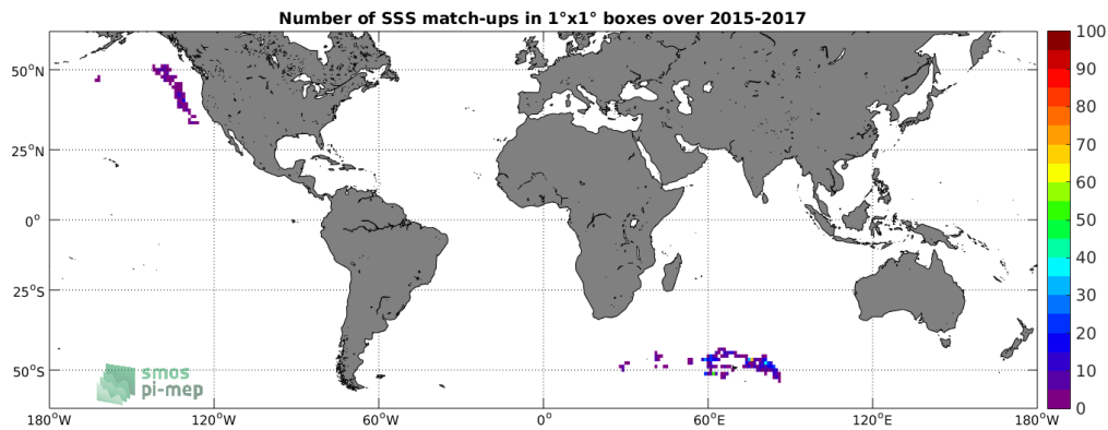
Figure 4: Number of SSS match-ups between Sea mammals SSS and the SMAP-L3-RSS-V3-MONTHLY-70KM SSS product for the SMOS coastal zone ( \approx 800\text{km} ) 60N-60S Pi-MEP region over 1^\circ \times 1^\circ boxes and for the full satellite product period.
