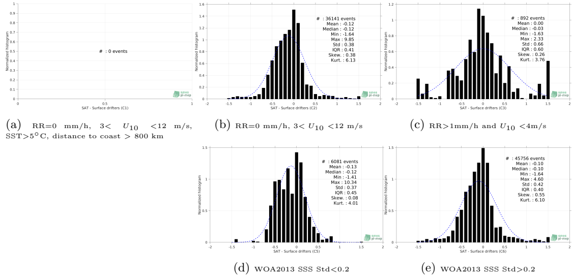
Figure 12: Normalized histogram of \Delta SSS (SMAP-L3-RSS-V3-MONTHLY-70KM - Surface drifters) for 5 different subdatasets corresponding to: RR=0 mm/h, 3 < U_{10} < 12 m/s, SST > 5°C, distance to coast > 800 km (a), RR=0 mm/h, 3 < U_{10} < 12 m/s (b), RR > 1mm/h and U_{10} < 4 m/s (c), WOA2013 SSS Std < 0.2 (d), WOA2013 SSS Std > 0.2 (e).
