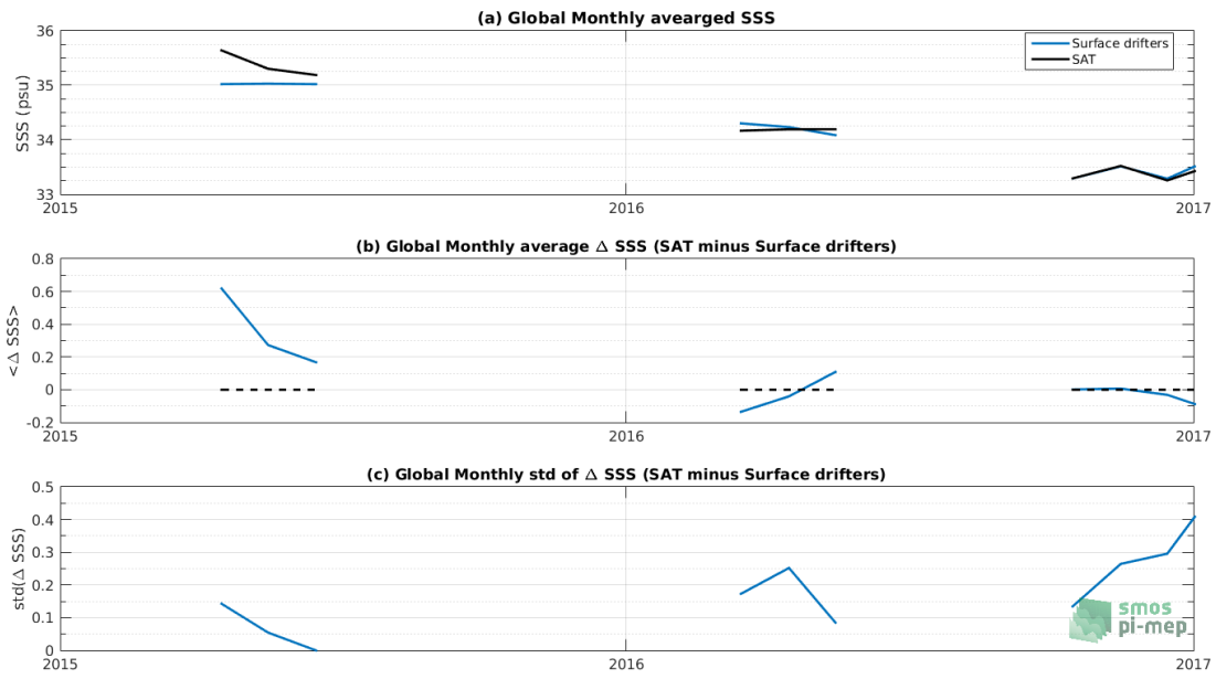
Figure 6: Time series of the monthly averaged mean SSS (top), mean \Delta\text{SSS} (Satellite - Surface drifters) and Std of \Delta\text{SSS} (Satellite - Surface drifters) over the SMOS coastal zone ( \approx 800\text{km} ) 60N-60S Pi-MEP region considering all match-ups collected by the Pi-MEP platform.
