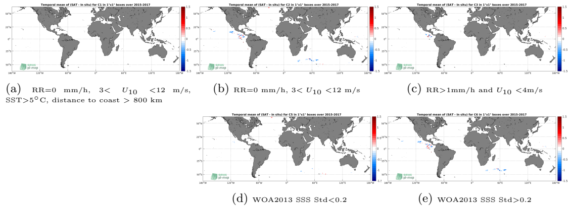
Figure 11: Temporal mean gridded over spatial boxes of size 1^\circ \times 1^\circ of \Delta SSS (SMAP-L3-RSS-V3-MONTHLY-70KM - Surface drifters) for 5 different subdatasets corresponding to: RR=0 mm/h, 3 < U_{10} < 12 m/s, SST > 5^\circ\text{C} , distance to coast > 800 km (a), RR=0 mm/h, 3 < U_{10} < 12 m/s (b), RR > 1 mm/h and U_{10} < 4 m/s (c), WOA2013 SSS Std < 0.2 (d), WOA2013 SSS Std > 0.2 (e).
