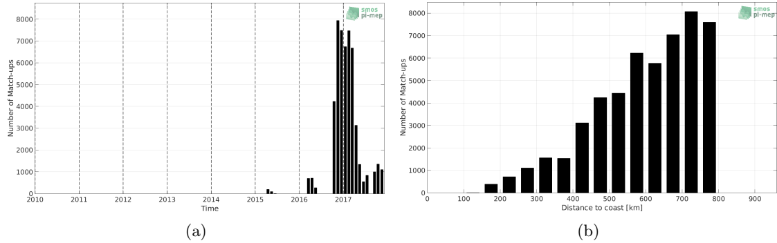
Figure 1: Number of match-ups between Surface drifters and SMAP-L3-RSS-V3-MONTHLY-70KM SSS as a function of time (a) and as function of the distance to coast (b) over the SMOS coastal zone ( \approx 800\text{km} ) 60N-60S Pi-MEP region and for the full satellite product period.
