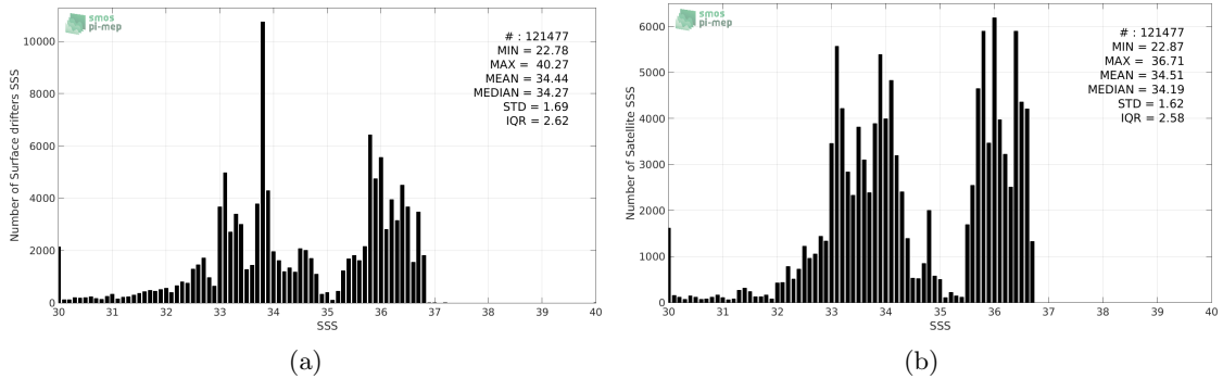
Figure 2: Histograms of SSS from Surface drifters (a) and SMAP-L3-RSS-V3-MONTHLY-70KM (b) considering all match-up pairs per bins of 0.1 over the SMOS coastal zone ( \approx 800\text{km} ) 60N-60S Pi-MEP region and for the full satellite product period.
