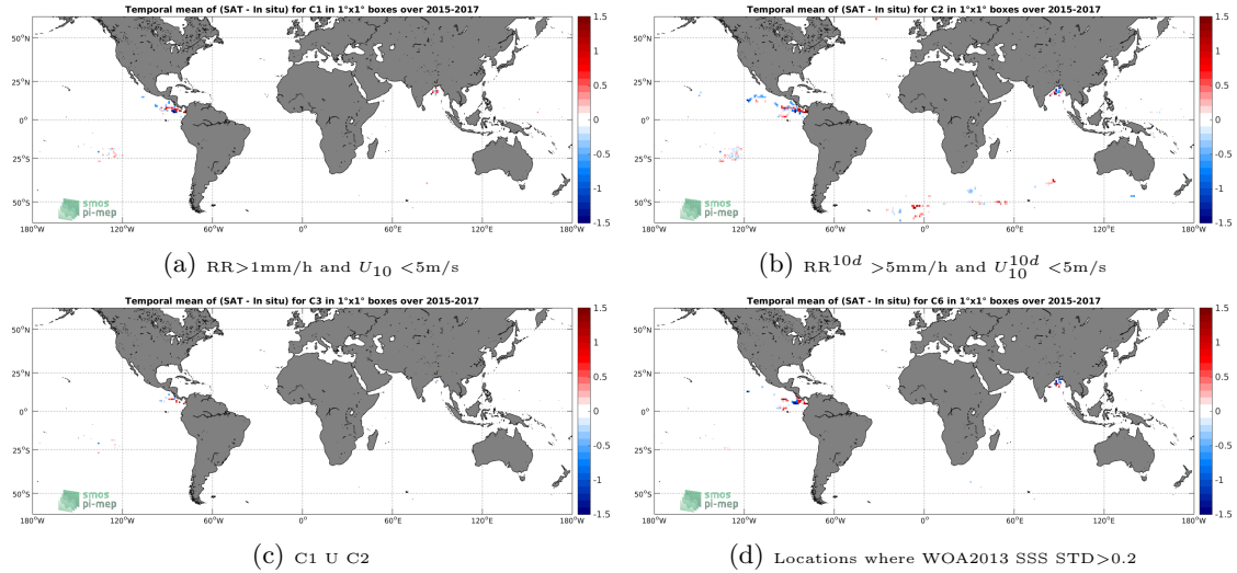
Figure 11: Temporal mean gridded over spatial boxes of size 1^\circ \times 1^\circ of \Delta SSS (SMAP-L3-RSS-V3-MONTHLY-70KM - Surface drifters) for 4 different subdatasets corresponding to: RR > 1\text{mm/h} and U_{10} < 5\text{m/s} (a), RR^{10d} > 5\text{mm/h} and U_{10}^{10d} < 5\text{m/s} (b), C1 U C2 (c), Locations where WOA2013 SSS STD > 0.2 (d).
