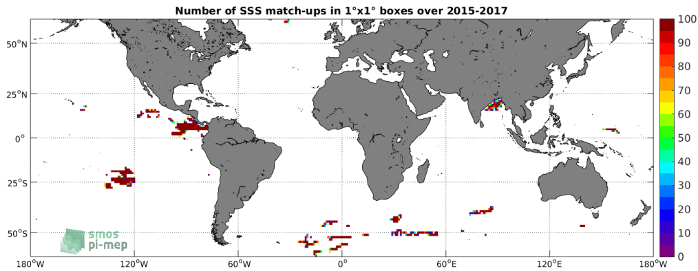
Figure 3: Number of SSS match-ups between Surface drifters SSS and the SMAP-L3-RSS-V3-MONTHLY-70KM SSS product for the SMOS coastal zone ( \approx 800\text{km} ) 60N-60S Pi-MEP region over 1^\circ \times 1^\circ boxes and for the full satellite product period.
