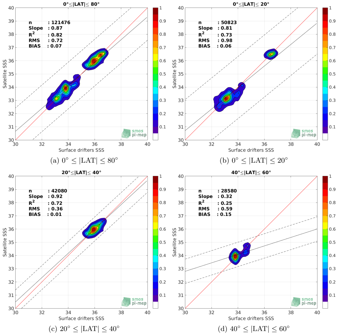
Figure 8: Contour maps of the concentration of SMAP-L3-RSS-V3-MONTHLY-70KM SSS (y-axis) versus Surface drifters SSS (x-axis) at match-up pairs for different latitude bands. For each plot, the red line shows x=y . The black thin and dashed lines indicate a linear fit through the data cloud and the \pm 95\% confidence levels, respectively. The number match-up pairs n , the slope and R^2 coefficient of the linear fit, the root mean square (RMS) and the mean bias between satellite and in situ data are indicated for each latitude band in each plots.
