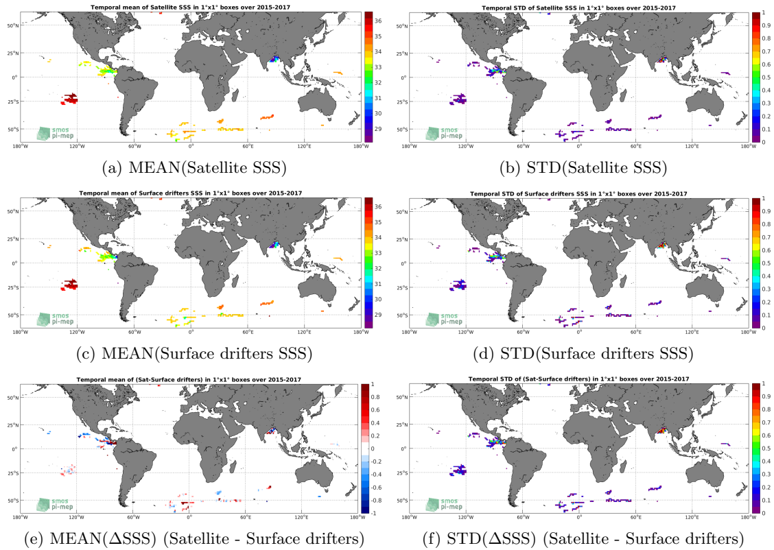
Figure 5: Temporal mean (left) and STD (right) of SSS from SMAP-L3-RSS-V3-MONTHLY-70KM (top), Surface drifters (middle), and of \Delta SSS (Satellite - Surface drifters). Only match-up pairs are used to generate these maps.
