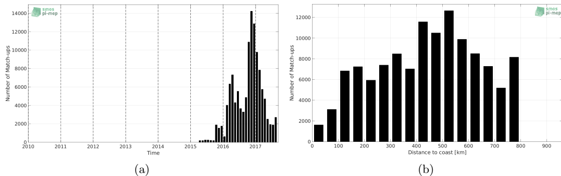
Figure 1: Number of match-ups between Surface drifters and SMAP-L3-RSS-V3-MONTHLY-70KM SSS as a function of time (a) and as function of the distance to coast (b) over the SMOS coastal zone ( \pm 800\text{km} ) 60\text{N} - 60\text{S} Pi-MEP region and for the full satellite product period.
