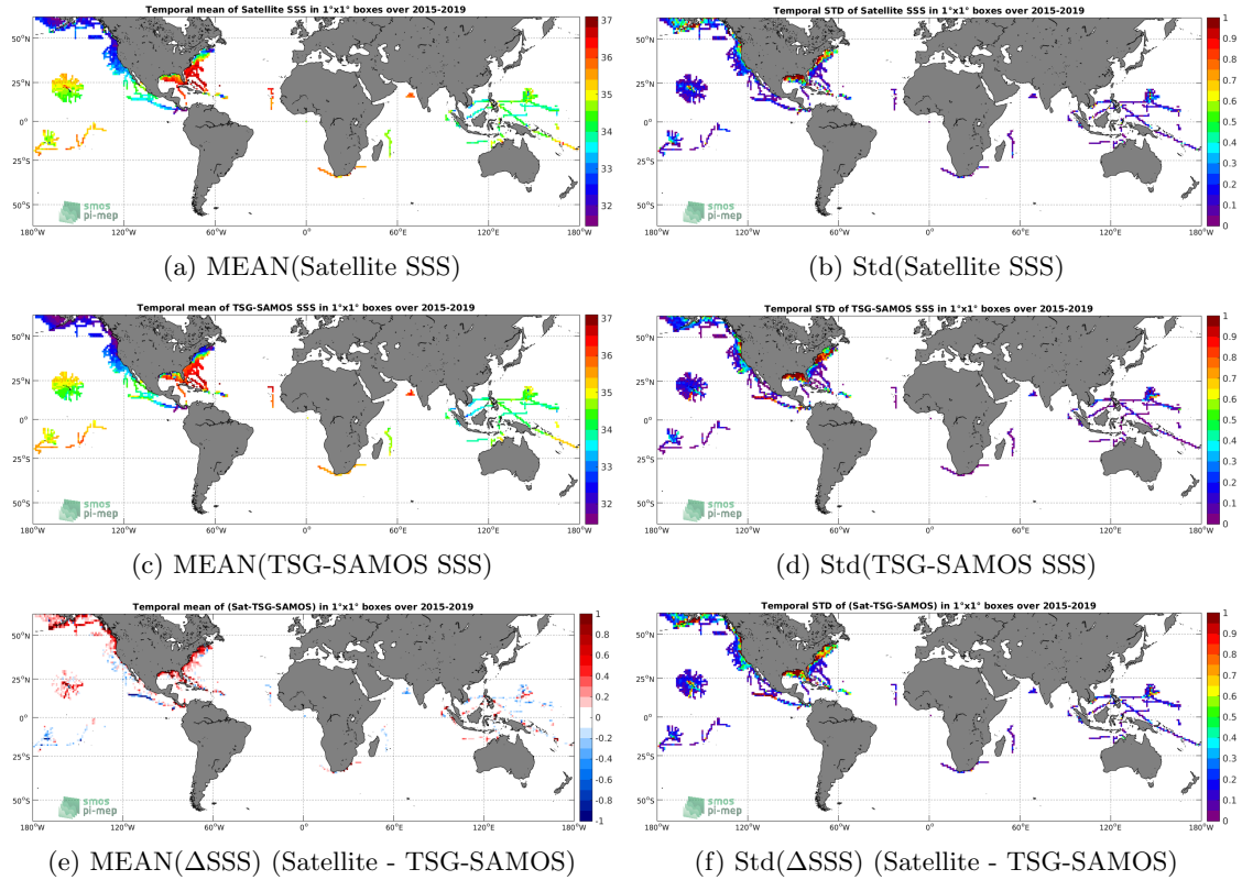
Figure 6: Temporal mean (left) and Std (right) of SSS from SMAP-L3-RSS-V3-MONTHLY-0.25DEG-40KM (top), TSG-SAMOS (middle), and of \Delta SSS (Satellite - TSG-SAMOS). Only match-up pairs are used to generate these maps.
