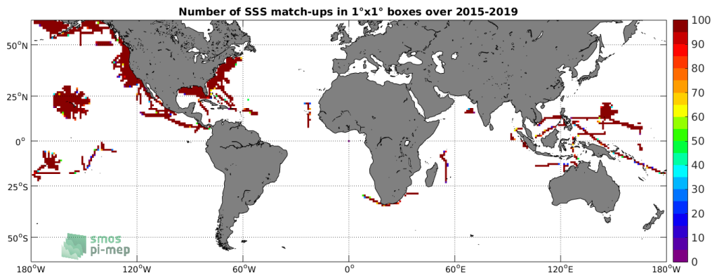
Figure 4: Number of SSS match-ups between TSG-SAMOS SSS and the SMAP-L3-RSS-V3-MONTHLY-0.25DEG-40KM SSS product for the SMOS coastal zone ( \approx 800\text{km} ) 60N-60S Pi-MEP region over 1^\circ \times 1^\circ boxes and for the full satellite product period.
