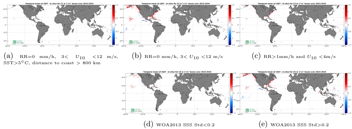
Figure 12: Temporal mean gridded over spatial boxes of size 1^\circ \times 1^\circ of \Delta SSS (SMAP-L3-RSS-V3-MONTHLY-0.25DEG-40KM - TSG-SAMOS) for 5 different subdatasets corresponding to:RR=0 mm/h, 3 < U_{10} < 12 m/s, SST >5^\circ\text{C} , distance to coast > 800 km (a), RR=0 mm/h, 3 < U_{10} < 12 m/s (b), RR >1 mm/h and U_{10} < 4 m/s (c), WOA2013 SSS Std <0.2 (d), WOA2013 SSS Std >0.2 (e).
