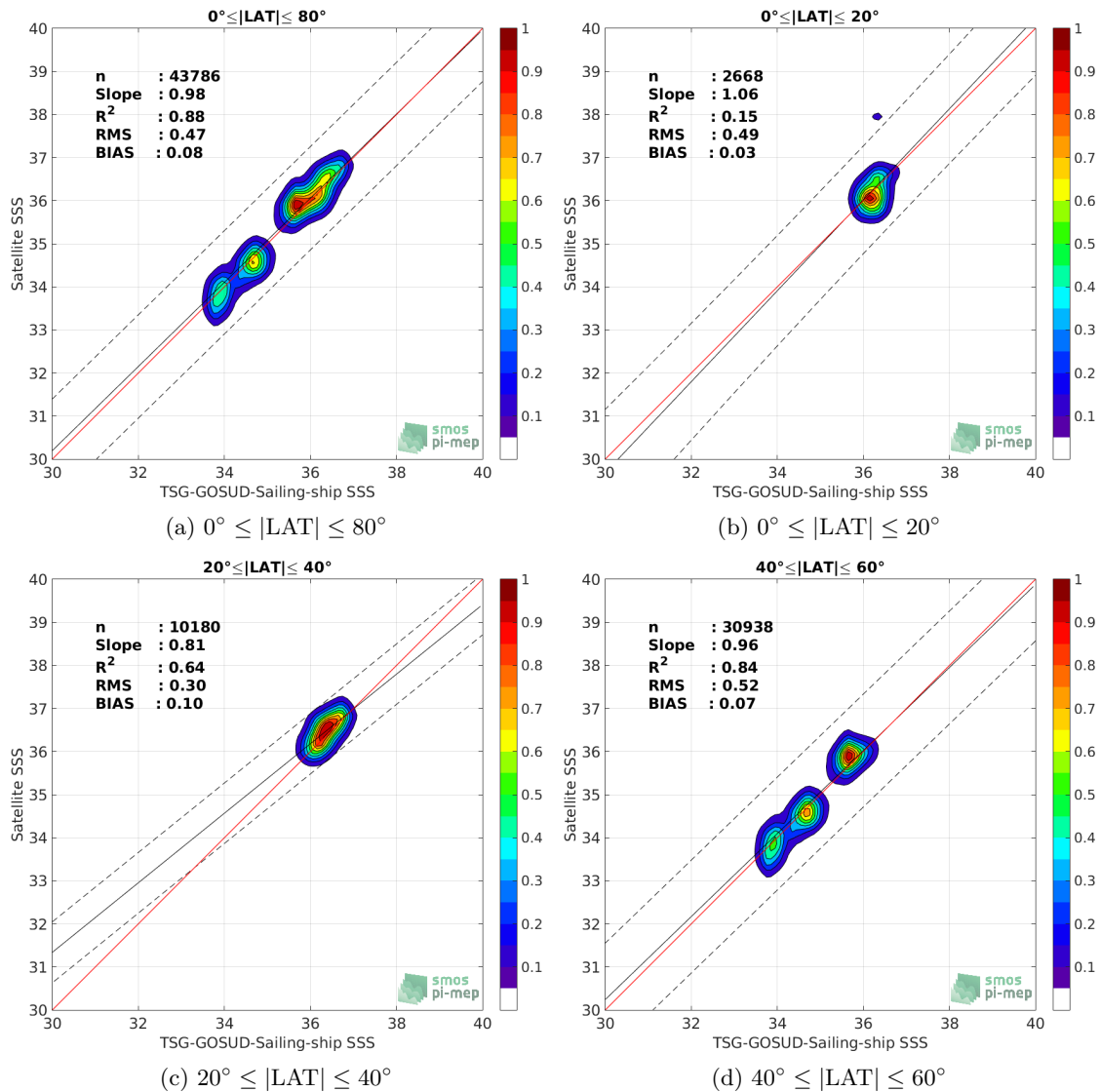
Figure 9: Contour maps of the concentration of SMAP-L3-RSS-V3-MONTHLY-0.25DEG-40KM SSS (y-axis) versus TSG-GOSUD-Sailing-ship SSS (x-axis) at match-up pairs for different latitude bands. For each plot, the red line shows x=y . The black thin and dashed lines indicate a linear fit through the data cloud and the \pm 95\% confidence levels, respectively. The number match-up pairs n , the slope and R^2 coefficient of the linear fit, the root mean square (RMS) and the mean bias between satellite and in situ data are indicated for each latitude band in each plots.
