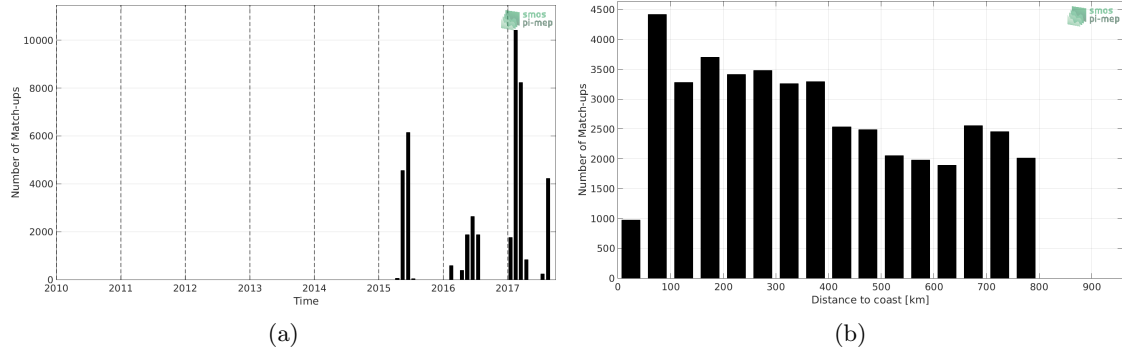
Figure 1: Number of match-ups between TSG-GOSUD-Sailing-ship and SMAP-L3-RSS-V3-MONTHLY-0.25DEG-40KM SSS as a function of time (a) and as function of the distance to coast (b) over the SMOS coastal zone ( \approx 800\text{km} ) 60N-60S Pi-MEP region and for the full satellite product period.
