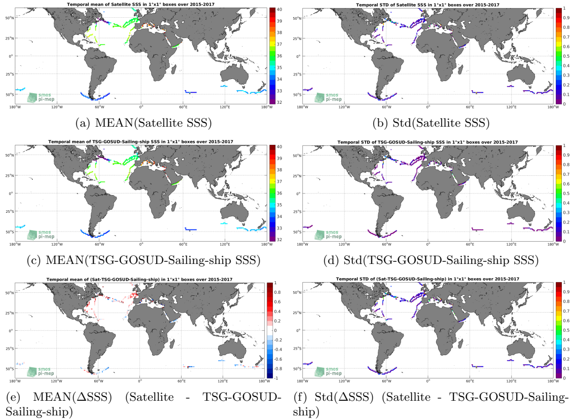
Figure 6: Temporal mean (left) and Std (right) of SSS from SMAP-L3-RSS-V3-MONTHLY-0.25DEG-40KM (top), TSG-GOSUD-Sailing-ship (middle), and of \Delta SSS (Satellite - TSG-GOSUD-Sailing-ship). Only match-up pairs are used to generate these maps.
