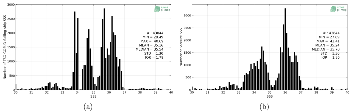
Figure 2: Histograms of SSS from TSG-GOSUD-Sailing-ship (a) and SMAP-L3-RSS-V3-MONTHLY-0.25DEG-40KM (b) considering all match-up pairs per bins of 0.1 over the SMOS coastal zone ( \approx 800\text{km} ) 60N-60S Pi-MEP region and for the full satellite product period.
