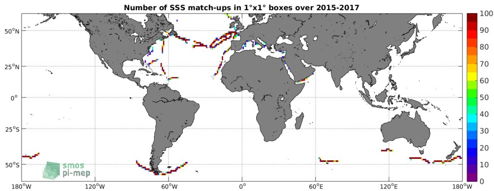
Figure 4: Number of SSS match-ups between TSG-GOSUD-Sailing-ship SSS and the SMAP-L3-RSS-V3-MONTHLY-0.25DEG-40KM SSS product for the SMOS coastal zone ( \approx 800\text{km} ) 60N-60S Pi-MEP region over 1^\circ \times 1^\circ boxes and for the full satellite product period.
