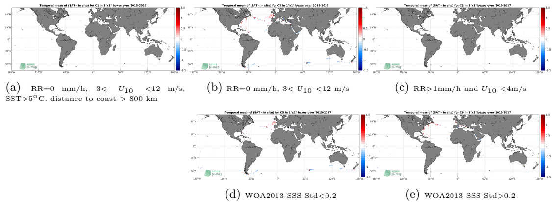
Figure 12: Temporal mean gridded over spatial boxes of size 1^\circ \times 1^\circ of \Delta SSS (SMAP-L3-RSS-V3-MONTHLY-0.25DEG-40KM - TSG-GOSUD-Sailing-ship) for 5 different subdatasets corresponding to:RR=0 mm/h, 3 < U_{10} < 12 m/s, SST >5^\circ C, distance to coast > 800 km (a), RR=0 mm/h, 3 < U_{10} < 12 m/s (b), RR >1 mm/h and U_{10} < 4 m/s (c), WOA2013 SSS Std <0.2 (d), WOA2013 SSS Std >0.2 (e).
