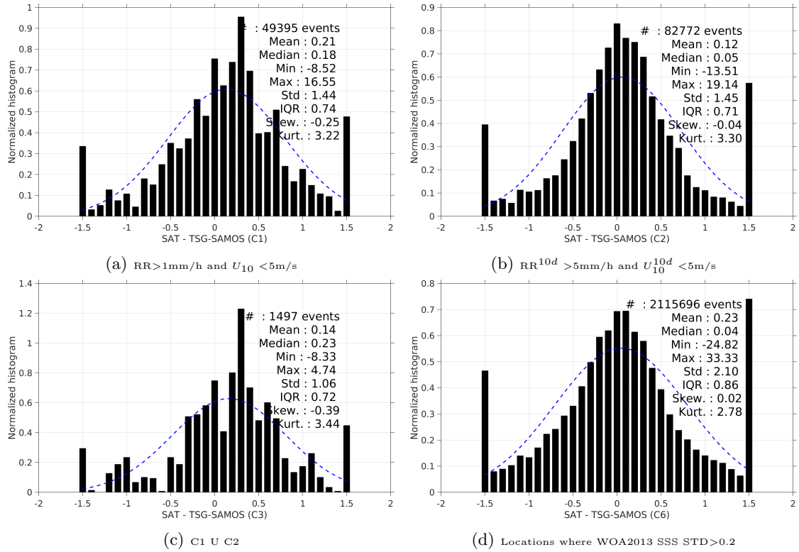
Figure 13: Normalized histogram of \Delta SSS (SMAP-L3-RSS-V2-8DAY-RUNNING-40KM - TSG-SAMOS) for 6 different subdatasets corresponding to: RR > 1mm/h and U_{10} < 5 m/s (a), RR^{10d} > 5 mm/h and U_{10}^{10d} < 5 m/s (b), C1 U C2 (c), Locations where WOA2013 SSS STD > 0.2 (d).
