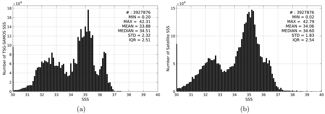
Figure 2: Histograms of SSS from TSG-SAMOS (a) and SMAP-L3-RSS-V2-8DAY-RUNNING-40KM (b) considering all match-up pairs per bins of 0.1 over the SMOS coastal zone ( \approx 800 km) 60N-60S Pi-MEP region and for the full satellite product period.
