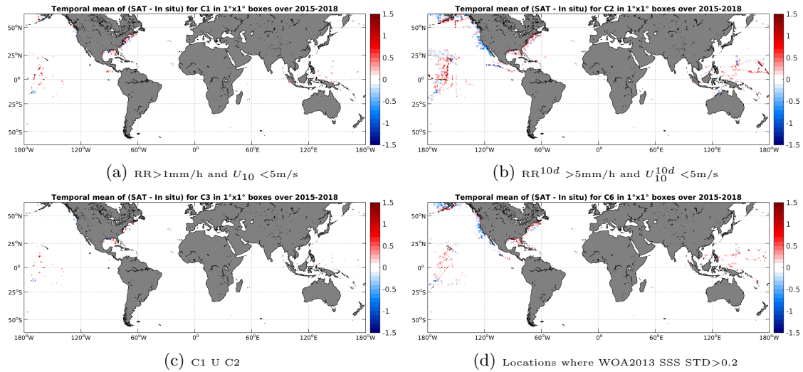
Figure 12: Temporal mean gridded over spatial boxes of size 1^\circ \times 1^\circ of \Delta SSS (SMAP-L3-RSS-V2-8DAY-RUNNING-40KM - TSG-SAMOS) for 4 different subdatasets corresponding to: RR > 1 mm/h and U_{10} < 5 m/s (a), RR 10d > 5 mm/h and U_{10}^{10d} < 5 m/s (b), C1 U C2 (c), Locations where WOA2013 SSS STD > 0.2 (d).
