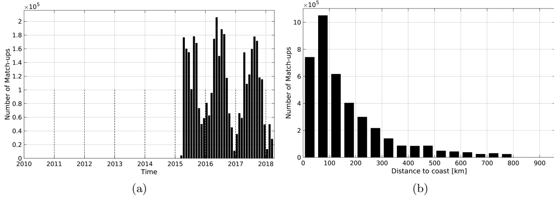
Figure 1: Number of match-ups between TSG-SAMOS and SMAP-L3-RSS-V2-8DAY-RUNNING-40KM SSS as a function of time (a) and as function of the distance to coast (b) over the SMOS coastal zone ( \approx 800 km) 60N-60S Pi-MEP region and for the full satellite product period.
