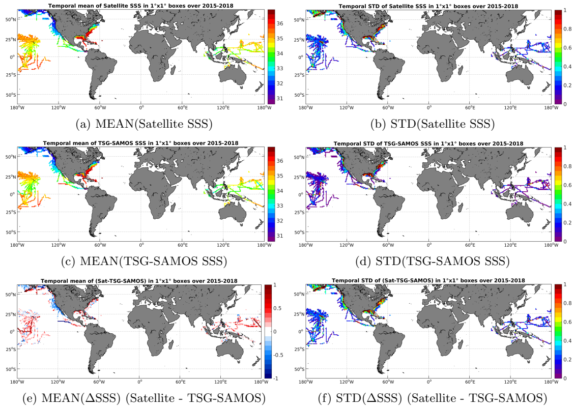
Figure 6: Temporal mean (left) and STD (right) of SSS from SMAP-L3-RSS-V2-8DAY-RUNNING-40KM (top), TSG-SAMOS (middle), and of \Delta SSS (Satellite - TSG-SAMOS). Only match-up pairs are used to generate these maps.
