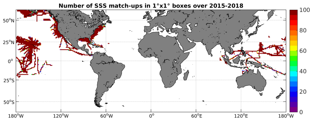
Figure 4: Number of SSS match-ups between TSG-SAMOS SSS and the SMAP-L3-RSS-V2-8DAY-RUNNING-40KM SSS product for the SMOS coastal zone ( \approx 800 km) 60N-60S Pi-MEP region over 1^\circ \times 1^\circ boxes and for the full satellite product period.
